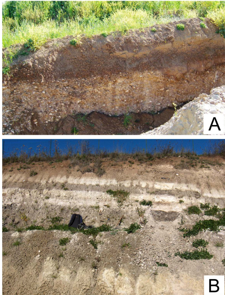
Fig. 2 - (A) Erosive and depositional unconformities marked by paleosols in a middle Pleistocene stratigraphic sequence in the Molise-Apulian Apennines between the Trigno and Fortore rivers (photo courtesy of V. Bracone). (B) Pleistocene pedostratigraphic succession alternating tephra and volcanic ash-bearing paleosols in the Sessano intramontane basin (Molise Apennines).
