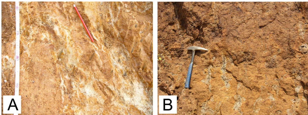
Fig. 15 - Irregular to reticulate (A) and tongued (B) redox depletion zones surrounded by iron-oxide stained pedogenic matrix in two paleosols developed on middle Pleistocene fluvial and marine terraces from the Tyrrhenian and Ionian coasts of Calabria, respectively.
