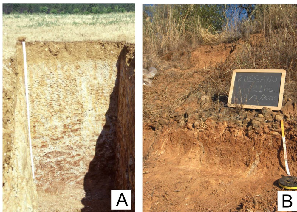
Fig. 14 - Paleosols exhibiting densely-packed horizons with hard consistence and fragic properties, which contributed to the development of glosic features, in places marking lenticular (A) or angular blocky to prismatic (B) structures. (A) Montagnola Senese, Tuscany; (B) Trionto River basin, Calabria).
