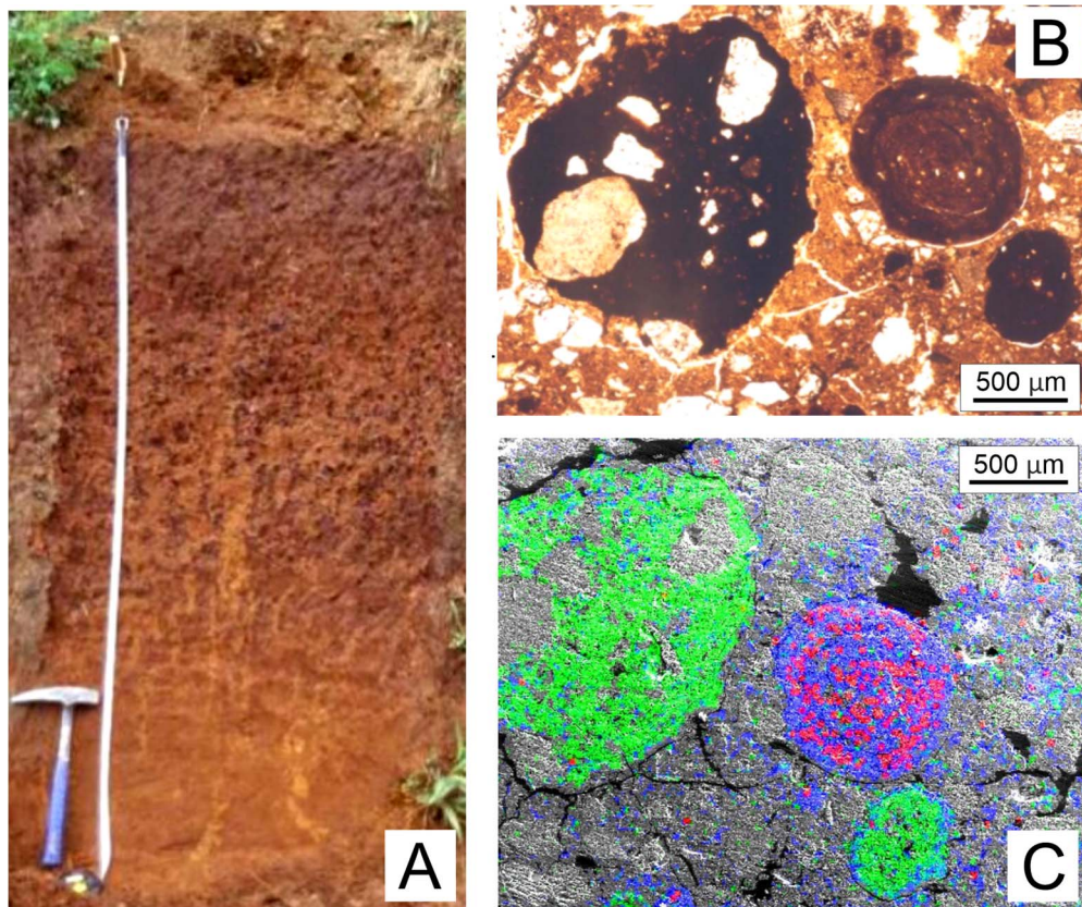
Fig. 8 - Partially truncated middle Pleistocene paleosol buried by marine bioclastic arenites in the Mt. Licosa promontory (Cilento, Campania) (A). Microphotograph of massive and concentric Fe-Mn nodules in the same paleosol (B) and corresponding EDS compositional maps of Mn (green), Fe (blue) and Cl (red) (C).
