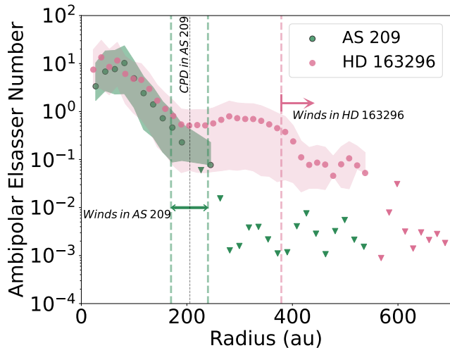
Figure 6. Ambipolar Elsasser number, A_m , calculated for the AS 209 disk (green) and the HD 163296 disk (pink). The triangles show upper limits on A_m when \text{HCO}^+ J = 1 - 0 is not detected. The shaded regions represent the uncertainty on the measurements, which are derived from the uncertainty in the N(\text{HCO}^+) measurement. The green dashed lines and arrows show the radial region where winds are found in AS 209, coincident with the annular gap in ^{12}\text{CO} and the CPD. The grey dashed line shows the radial location of the CPD in AS 209 (Bae et al. 2022b). The pink dashed line and arrow show the radial region where winds are found in HD 163296 (Teague et al. 2019a).
