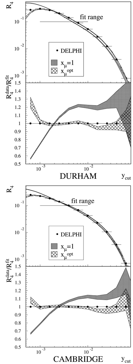
Fig. 12. Fits to the four-jet rate R_4 measured at the Z resonance using different scale evaluation methods. Top: the distributions. The hatched curve shows the results for the experimentally optimised scales. Bottom: the ratio R_4^{\text{data}}/R_4^{\text{fit}} . The grey bands show fit results with the physical scale ( x_\mu = 1 ), the cross-hatched bands for experimentally optimised scales ( x_\mu^{\text{opt}} )
