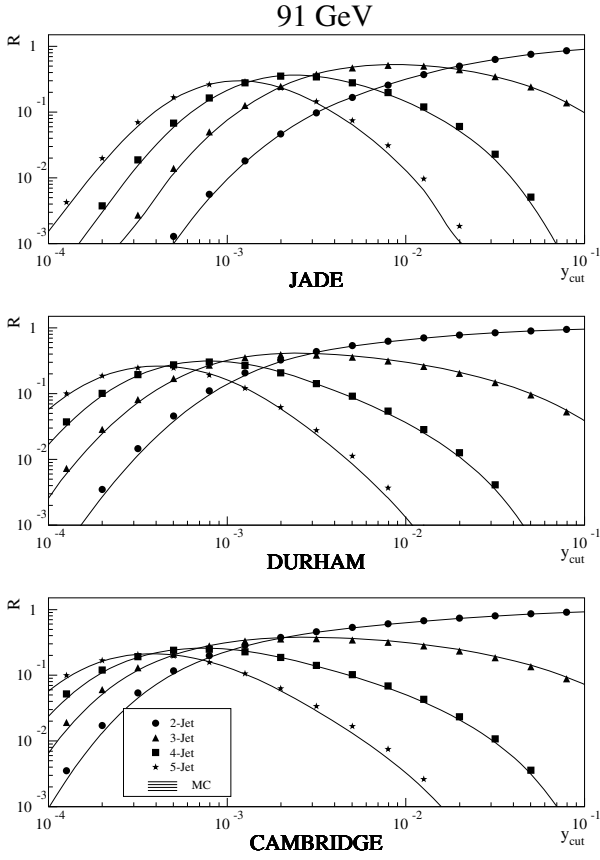
Fig. 4. Jet rates ( R ) at 91 GeV as a function of y_{\text{cut}} compared to the prediction of PYTHIA 6.1
