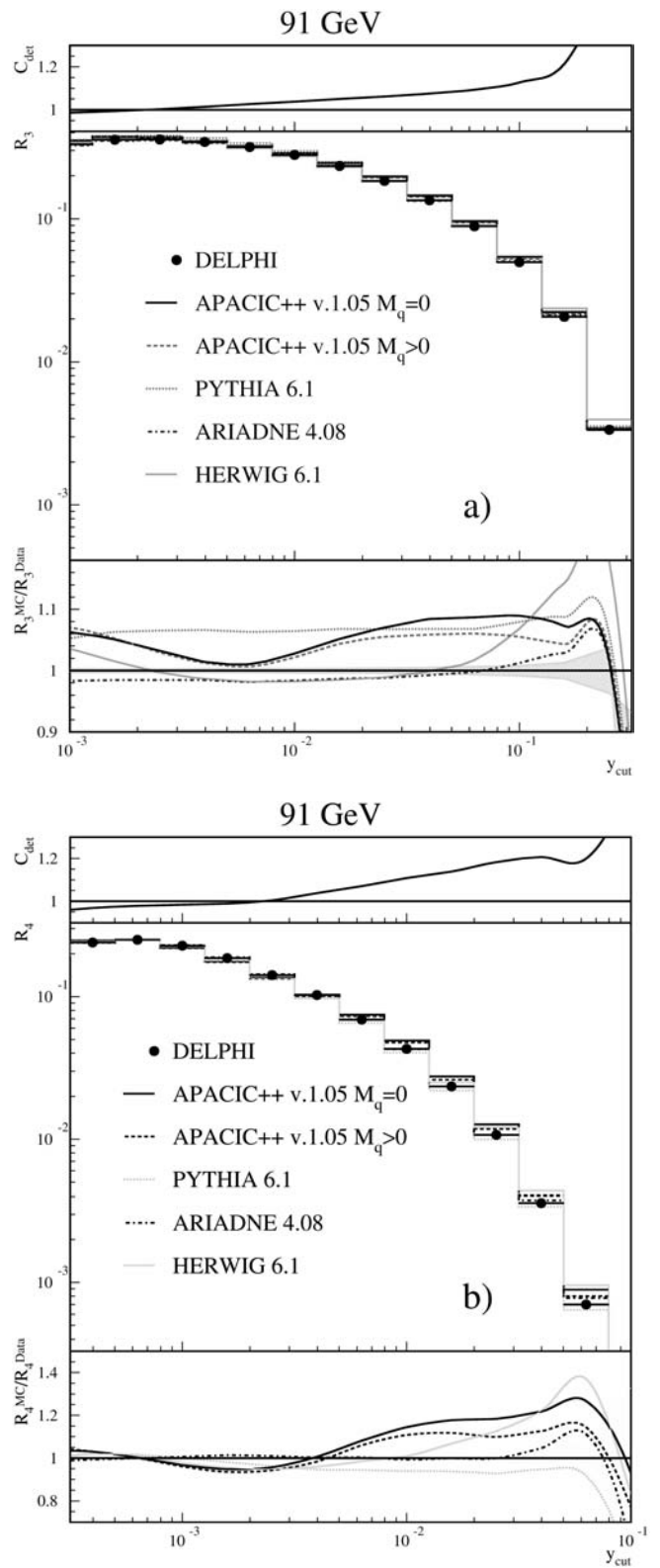
Fig. 7. Jet rates determined with the CAMBRIDGE algorithm. a 3-jet rate at 91 GeV. b 4-jet rate at 91 GeV. The upper inset shows the corrections C_{det} applied to the data. The central plot shows the jet rates with their statistical error in comparison with different Monte Carlo predictions. The lower inset shows the jet rates normalised to the data. The band indicates the statistical and systematical uncertainty of the data
