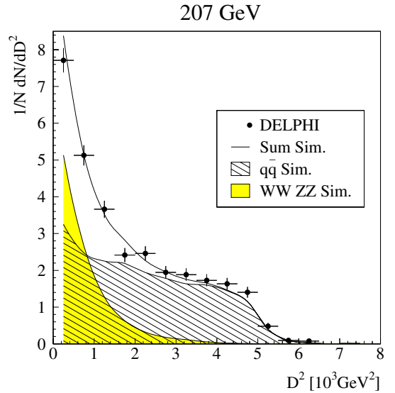
Fig. 2. Distribution of D^2 for accepted data at 207 GeV before applying four-fermion cuts, compared to q\bar{q} and 4f simulation
