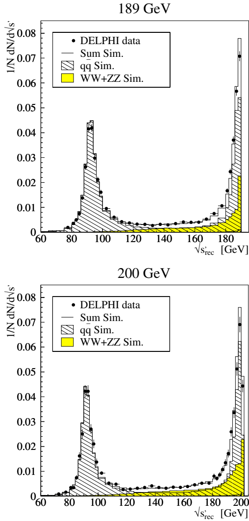
Fig. 1. Reconstructed centre of mass energy \sqrt{s'_{\text{rec}}} before all cuts except the one on \sqrt{s'_{\text{rec}}} compared to QCD and four-fermion simulations. The small differently shaded areas in the bottom right of the plots indicate the size of WW and neutral boson pair background
