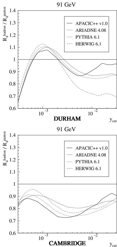
Fig. 10. Distribution of the hadronisation corrections to the four-jet rate. The plots show the ratio of the four-jet rates after and before simulation of the fragmentation, evaluated with different Monte Carlo models
