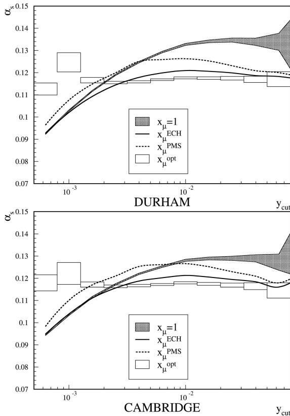
Fig. 13. Dependence of \alpha_s on y_{\text{cut}} : The grey bands give fit results with physical scale ( x_\mu = 1 ), the lines with theoretically optimised scales (ECH, PMS) and the rectangles with experimentally optimised scales ( x_\mu^{\text{opt}} )
