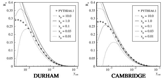
Fig. 9. Predictions (left for DURHAM, right for CAMBRIDGE) of the four-jet rate R_4 at 91 GeV using DEBRECEN and (8) for various values of x_\mu at fixed \alpha_s = 0.118 . Illustrated is the change of the prediction with varying x_\mu . The analytical calculations are compared to the parton level prediction using the PYTHIA generator
