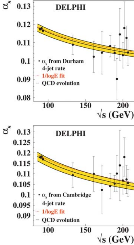
Fig. 14. Energy dependence of \alpha_s as obtained from jet rates with experimentally optimised scales. The errors shown are statistical only. The band shows the QCD expectation when extrapolating the world average [28] to other energies. The dashed lines show the result of the 1/\log \sqrt{s} fits
