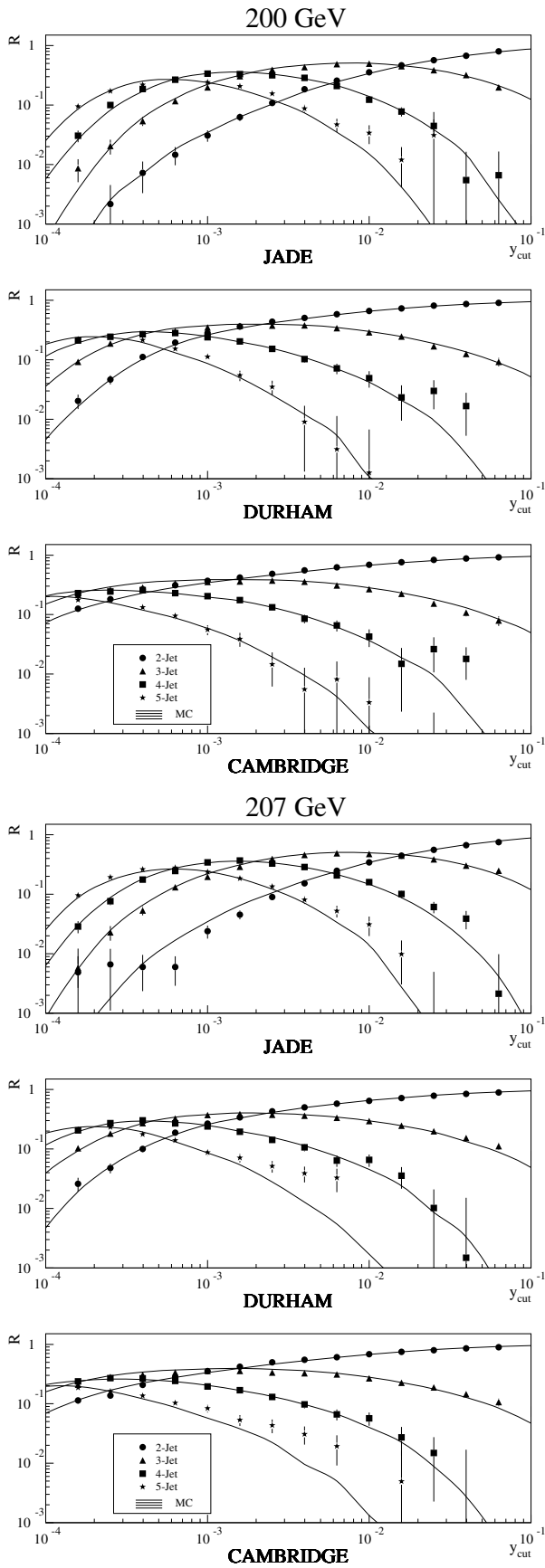
Fig. 6. Jet rates ( R ) at 200 and 207 GeV as a function of y_{cut} compared to the prediction of PYTHIA 6.1
