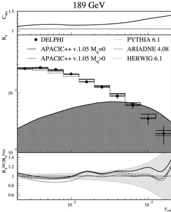
Fig. 8. 4-jet rate at 189 GeV determined with the CAMBRIDGE algorithm. The upper inset shows the corrections C_{\text{det}} applied to the data. The central plot shows the jet rates with their statistical error in comparison with different Monte Carlo predictions. The grey area in the central plot shows the already subtracted background of WW and ZZ events. The lower inset shows the jet rates normalised to the data. The band indicates the statistical and systematic uncertainty of the data
