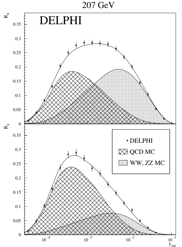
Fig. 3. Four-jet rate ( R_4 ), determined with the CAMBRIDGE algorithm, from raw data at 207 GeV as a function of y_{\text{cut}} , compared to the simulation of the contributing processes. Top: before cuts against four-fermion background. Bottom: After cutting at D^2 > 900 \text{ GeV}^2
