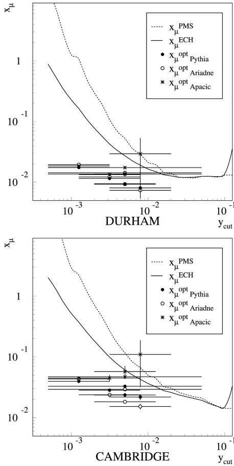
Fig. 11. Optimised renormalisation scales: The lines show the y_{\text{cut}} dependence for theoretically optimised scales at E_{\text{cm}} = 91 \text{ GeV} . The dots give results for experimentally optimised scales. The error bars in the horizontal direction indicate the fit range, the different symbols represent hadronisation corrections applied by different Monte Carlo models
