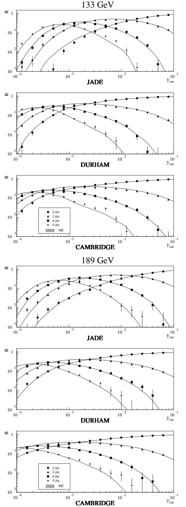
Fig. 5. Jet rates ( R ) at 133 and 189 GeV as a function of y_{\text{cut}} compared to the prediction of PYTHIA 6.1
