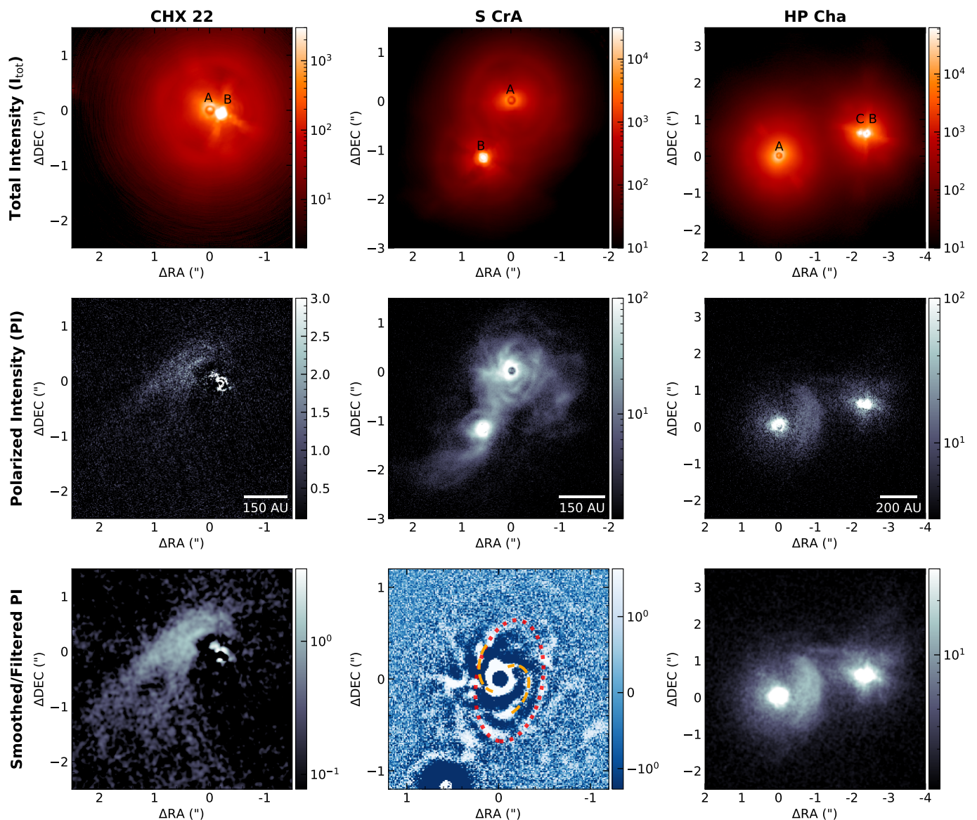
Fig. 1. SPHERE/IRDIS images of the three multiple systems, centered on the primary stars. Each column shows one system, namely CHX 22, S CrA, and HP Cha. Top row: total intensity images. Middle row: polarized intensity images. Bottom row: processed PI images for better visualization of features. The PI image of CHX 22 is smoothed through convolution with a Gaussian kernel with a width of 2 pixels, revealing the dust tail clearly. The PI image of S CrA is high-pass filtered by subtracting the Gaussian smoothed image from the original image, to highlight the potential ring (red dotted ellipse) and spiral features (orange dashed curves). The PI image of HP Cha is also Gaussian smoothed. In the colorbars we show the scaling of the figures in arbitrary units to indicate the significance of the various detected structures. For a flux calibrated version of the polarimetric observations we refer to Appendix E.
