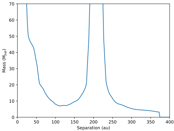
Fig. B.2. Mass limits for companions around the star S CrA, calculated from the contrast curve in Fig. B.1.
