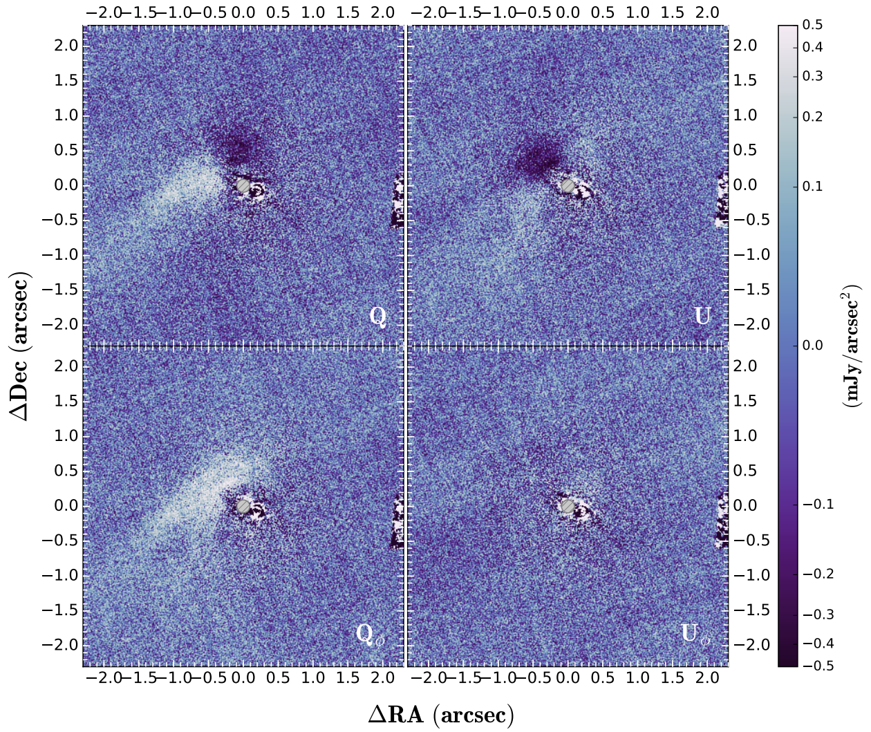
Fig. E.1. Stokes Q , U , Q_\phi , and U_\phi polarized flux images of CHX 22 derived from SPHERE/IRDIS observations. The size of the coronagraphic mask is indicated with the grey, hashed circle.
