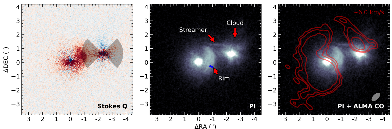
Fig. 3. Left panel: Stokes Q image of HP Cha. The angle of linear polarization in the Stokes Q pattern of the rim corresponds to an illumination source located at the position of companions BC (as delineated by the butterfly shadow centered at companions). Central panel: smoothed PI image where we identified the rim in the circumprimary disk, the streamer connecting the circumprimary and circumsecondary disk, and the nebulous envelope surrounding the BC components. The blue bar delineates the disk height at the most extended point of the outer rim. Right panel: overlay of ALMA CO gas emission (red contour) at the radial velocity of \sim 6.0 \text{ km s}^{-1} . The contours delineate the flux level of [3, 5, 10, 50]\sigma , where \sigma is the standard deviation as measured in the image background. The gray ellipse denotes the beam ( 0.77'' \times 0.40'' ) of ALMA observations.
