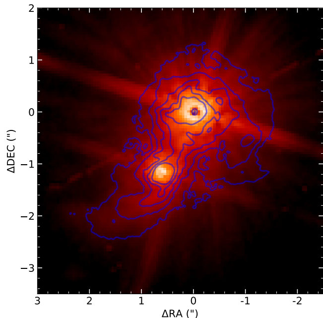
Fig. A.1. HST observations of S CrA. The blue contour delineates the flux level of [5, 10, 20, 40, 80]\sigma in the SPHERE PI image, where \sigma is the standard deviation as measured in the image background.
