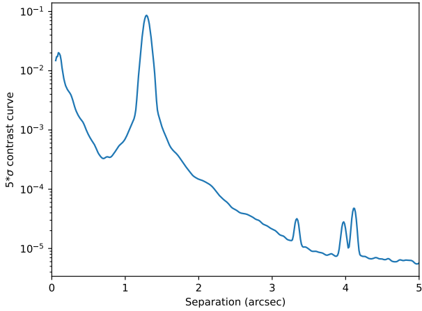
Fig. B.1. Contrast curve at 5\sigma -level for the ADI image of the system S CrA.
