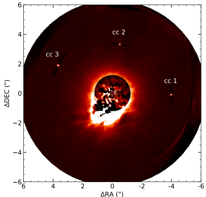
Fig. A.3. PCA image of S CrA with two principal components subtracted.
