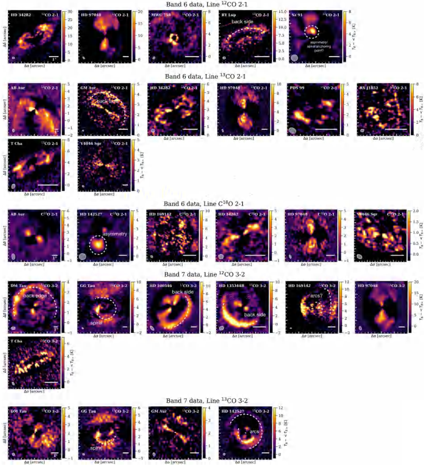
Fig. E.7. Brightness temperature residuals obtained with GoFish, shown for the additional Band 6 and Band 7 lines used in this analysis and for a thick disc geometry. The circle and bar in the bottom left and bottom right corner of each panel indicate the beam and a 1'' scale, respectively. Some features are annotated.
