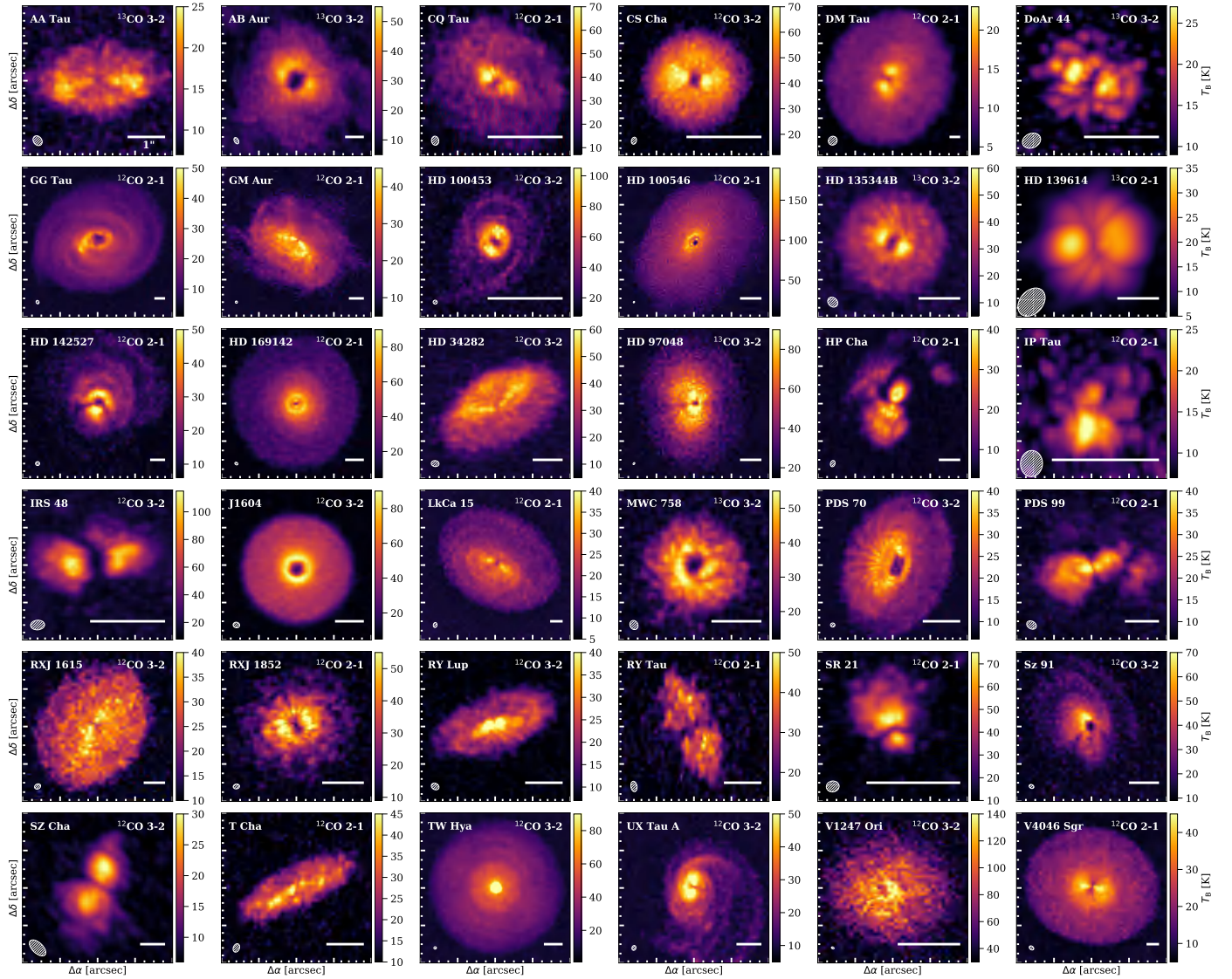
Fig. 1. Peak brightness temperature maps of the gas emission in our targets, shown for the main CO lines used in this analysis. The conversion from peak intensity to units of Kelvin was done with the Planck law. The circle and bar in the bottom left and bottom right corner of each panel indicate the beam and a 1'' scale, respectively.
