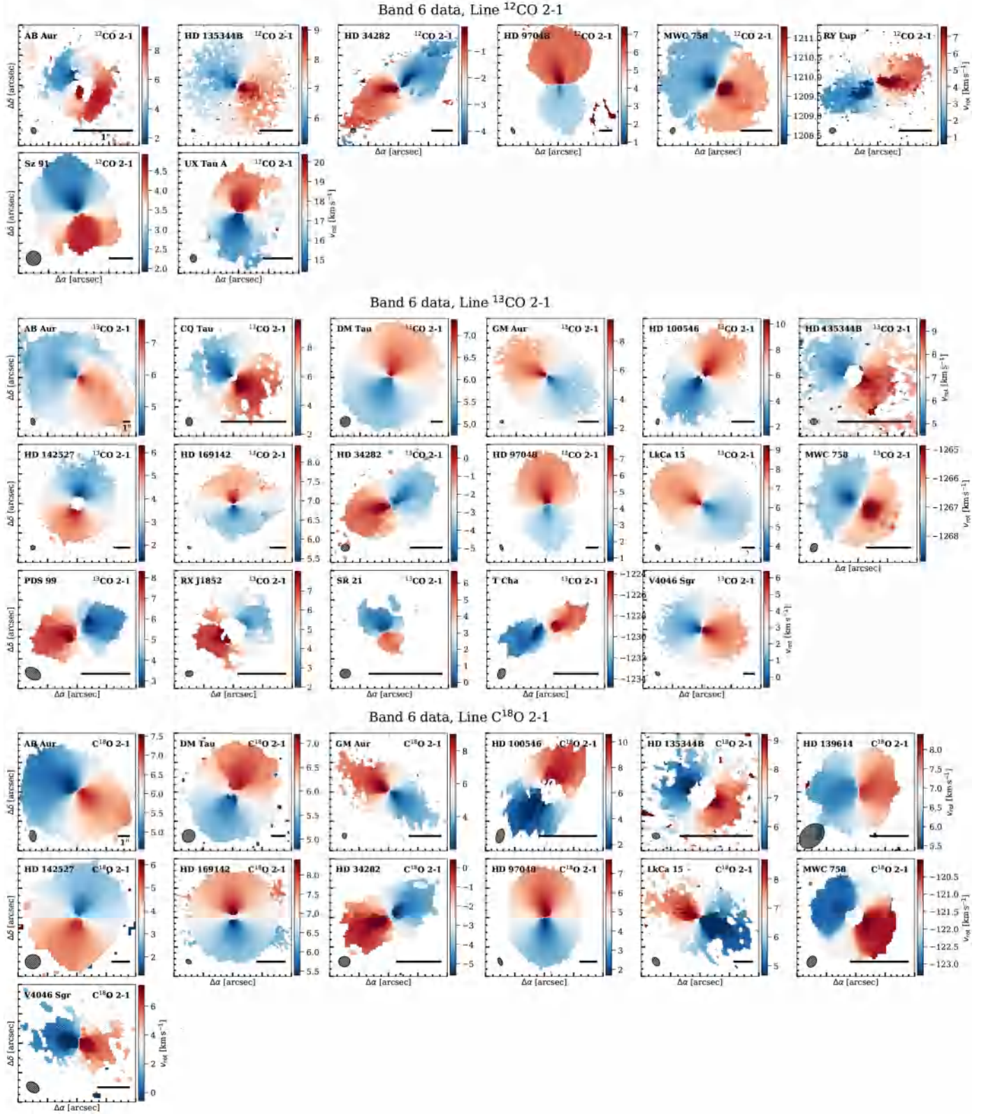
Fig. E.3. Rotation velocity maps of the gas emission in our targets, shown for the additional Band 6 lines used in this analysis. The maps were computed with bettermoments . The circle and bar in the bottom left and bottom right corner of each panel indicate the beam and a 1'' scale, respectively.
