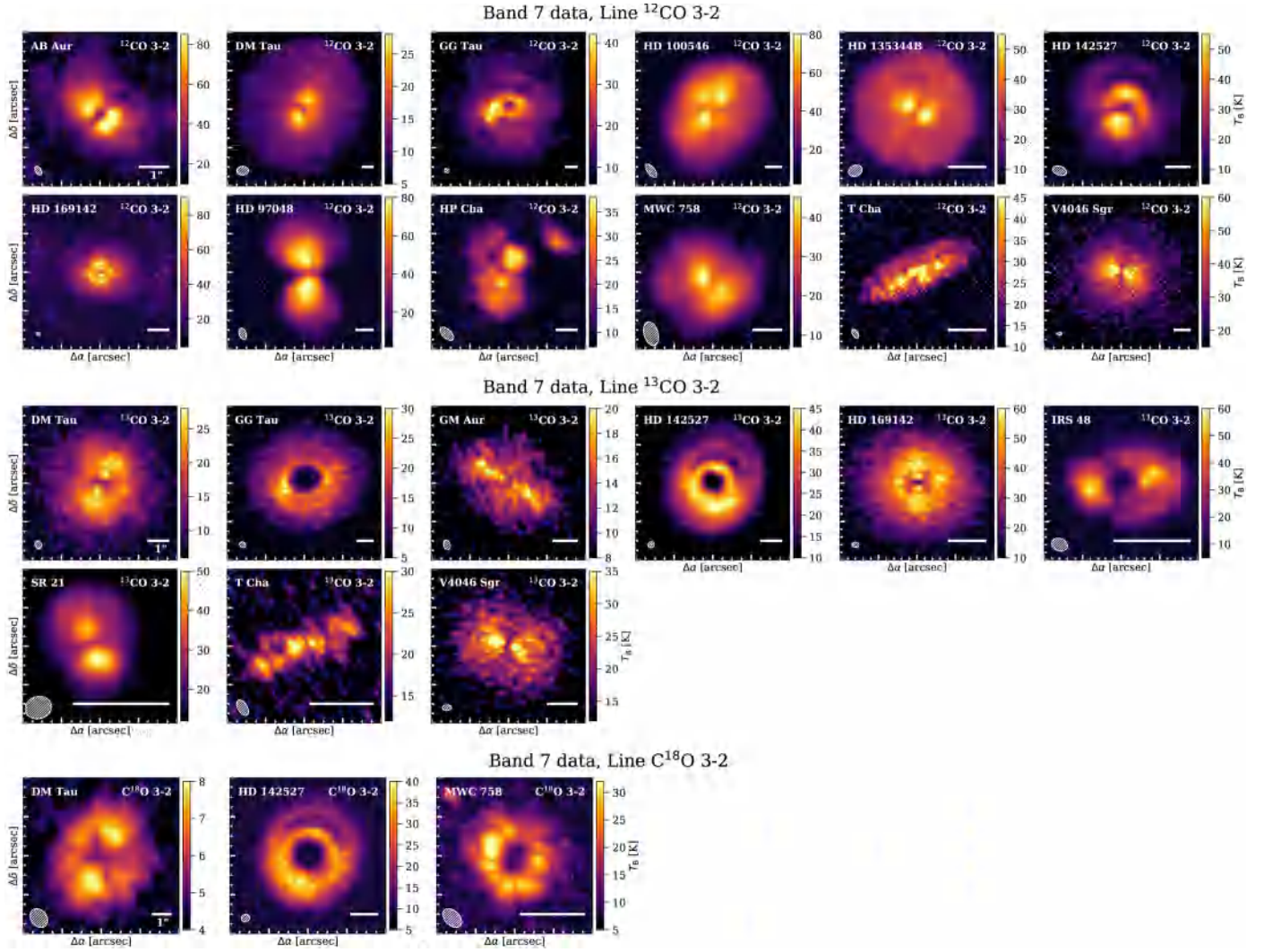
Fig. E.2. Peak brightness temperature maps of the gas emission in our targets, shown for the additional Band 7 CO lines used in this analysis. The conversion from peak intensity to units of Kelvin was done with the Planck law. The circle and bar in the bottom left and bottom right corner of each panel indicate the beam and a 1'' scale, respectively.
