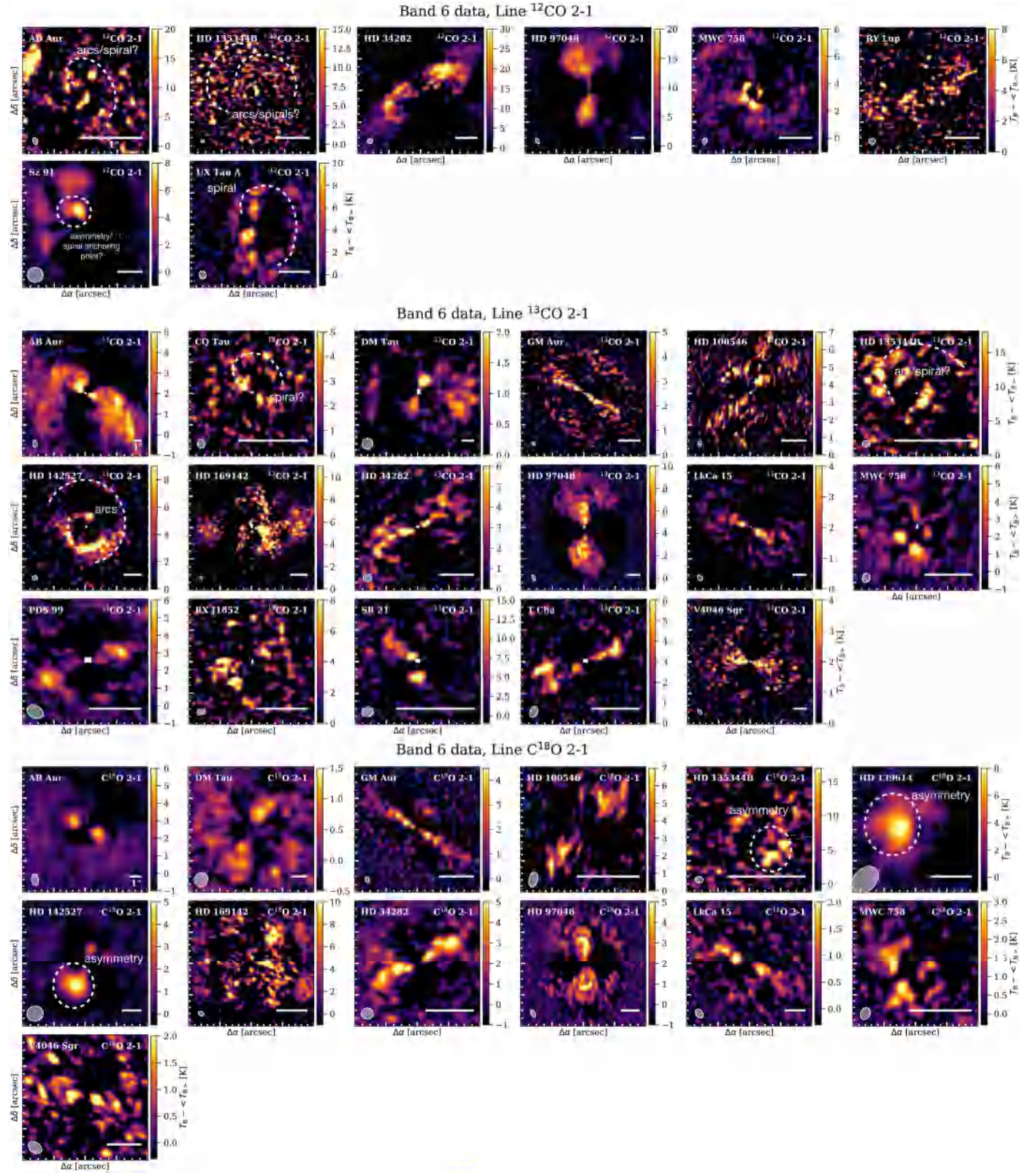
Fig. E.5. Brightness temperature residuals obtained with GoFish, shown for the additional Band 6 lines used in this analysis and for a thin disc geometry. The circle and bar in the bottom left and bottom right corner of each panel indicate the beam and a 1'' scale, respectively. Some features are annotated.
