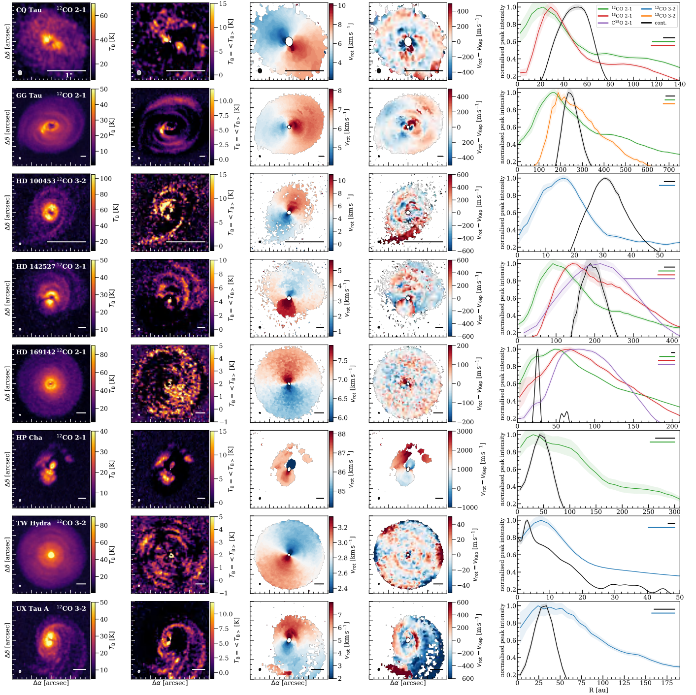
Fig. 7. Brightness temperature and velocity maps as well as their corresponding residuals and radial profiles, shown for the eight targets with the clearest substructures. The circle and bar in the bottom left and bottom right corner of the maps indicate the beam and a 1'' scale, respectively. For the radial profiles, the major beam of each observations is indicated by the bars in the top right corner.
