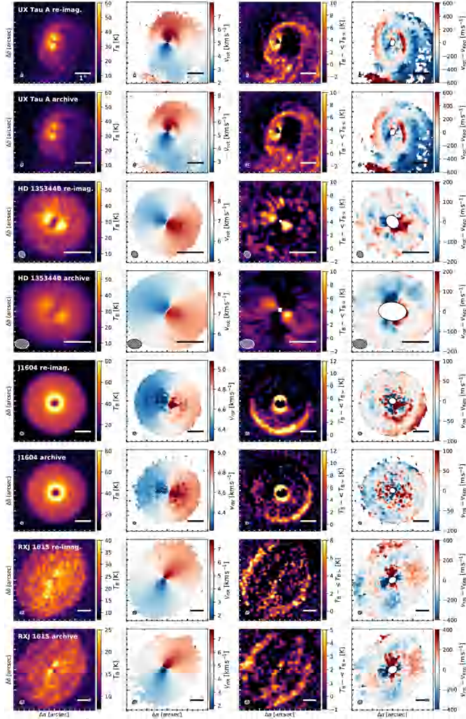
Fig. D.1. Comparison between the re-imaged and archival data for four sample sources, including one with clear spirals, two with tentative features, and one without any features. The circle and bar in the bottom left and bottom right corner of each panel indicate the beam and a 1'' scale, respectively.
