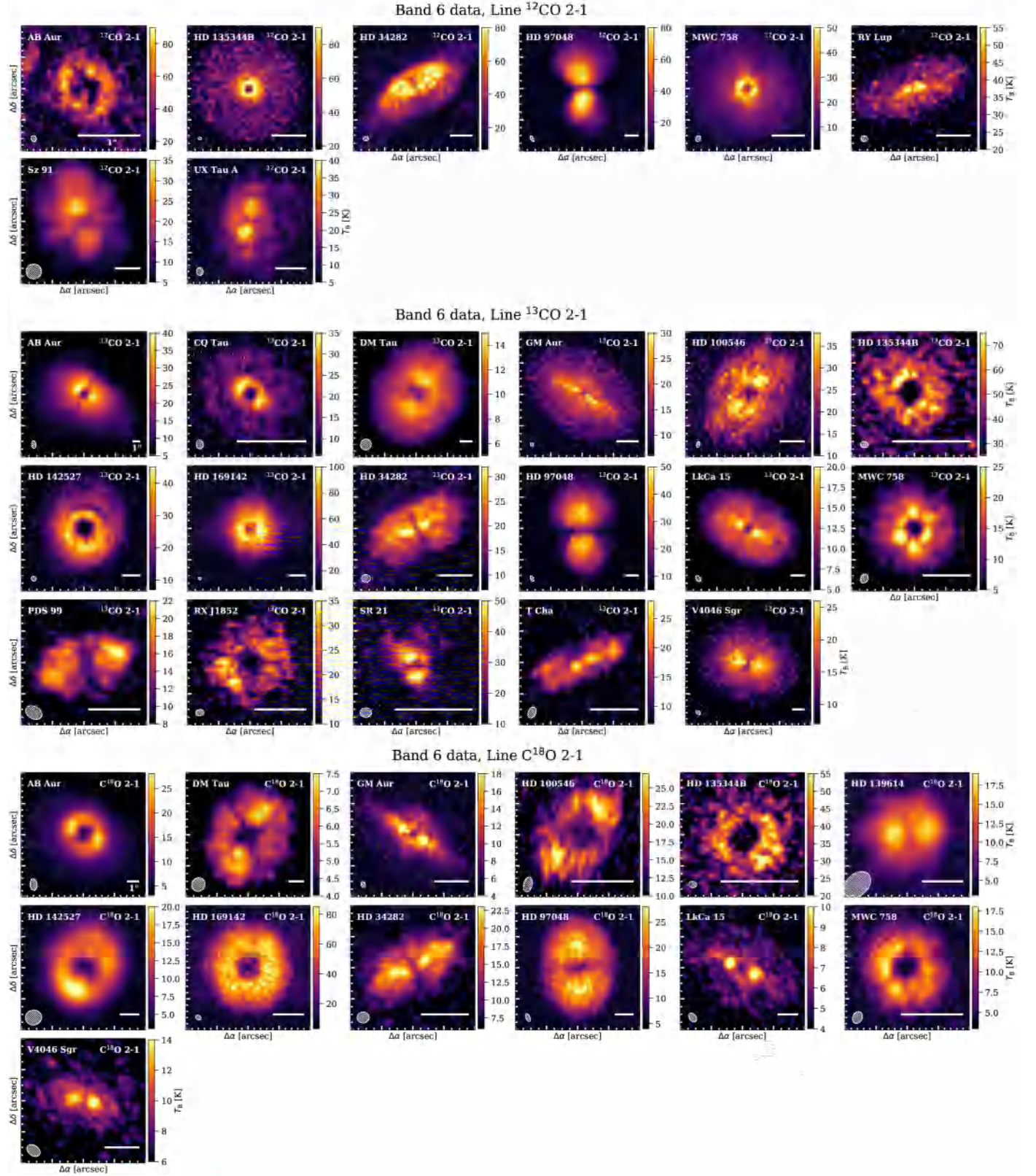
Fig. E.1. Peak brightness temperature maps of the gas emission in our targets, shown for the additional Band 6 CO lines used in this analysis. The conversion from peak intensity to units of Kelvin was done with the Planck law. The circle and bar in the bottom left and bottom right corner of each panel indicate the beam and a 1'' scale, respectively.
