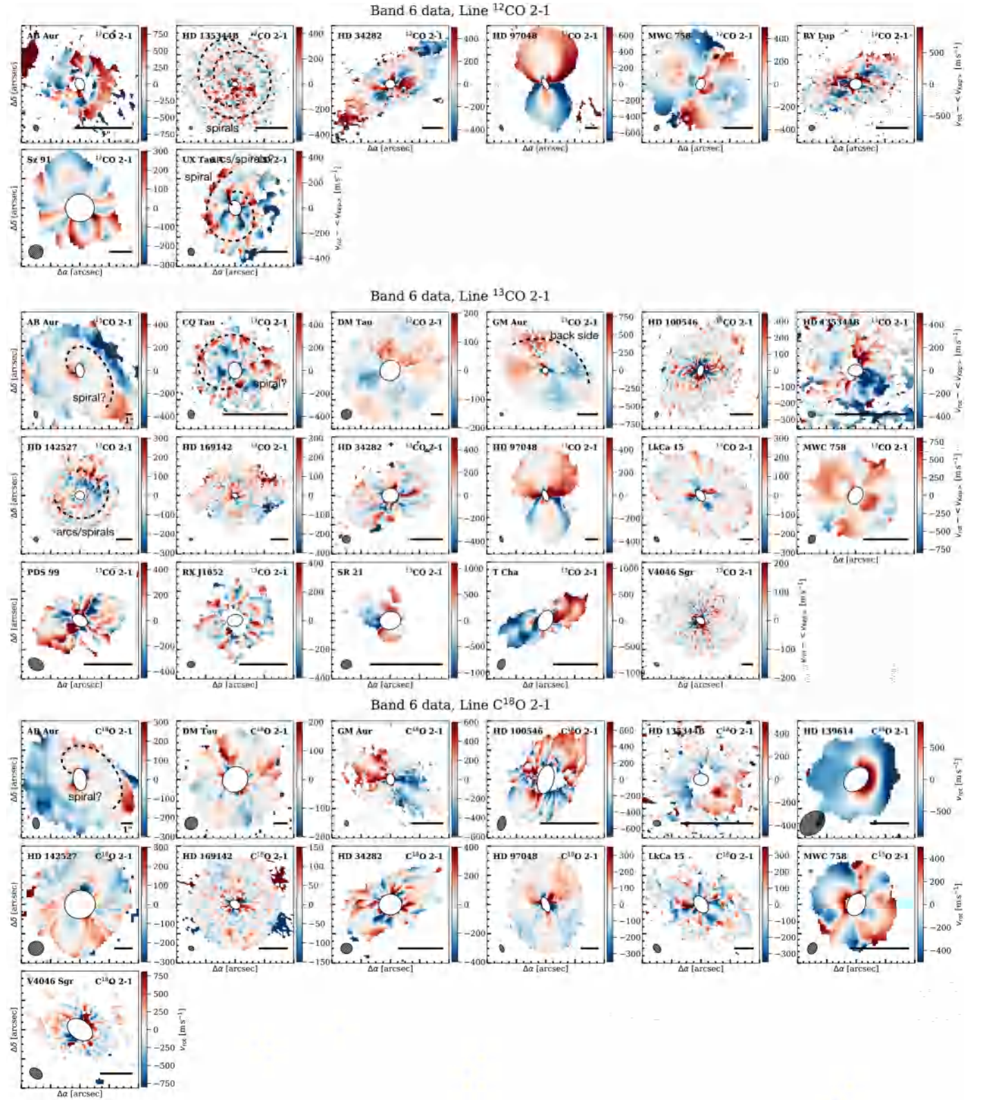
Fig. E.8. Rotation velocity residuals obtained with eddy, shown for the additional Band 6 lines used in this analysis and for a thin disc geometry. The circle and bar in the bottom left and bottom right corner of each panel indicate the beam and a 1'' scale, respectively. Some features are annotated.
