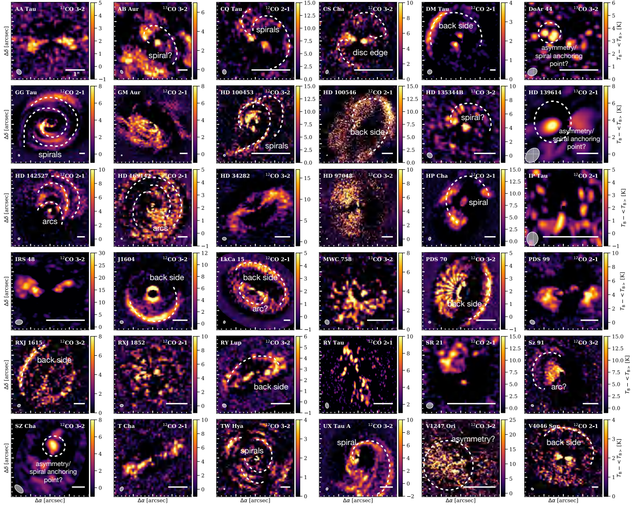
Fig. 5. Brightness temperature residuals obtained with GoFish, shown for the main CO lines used in this analysis and for a geometrically thin disc approximation. The circle and bar in the bottom left and bottom right corner of each panel indicate the beam and a 1'' scale, respectively. The main features are annotated.
