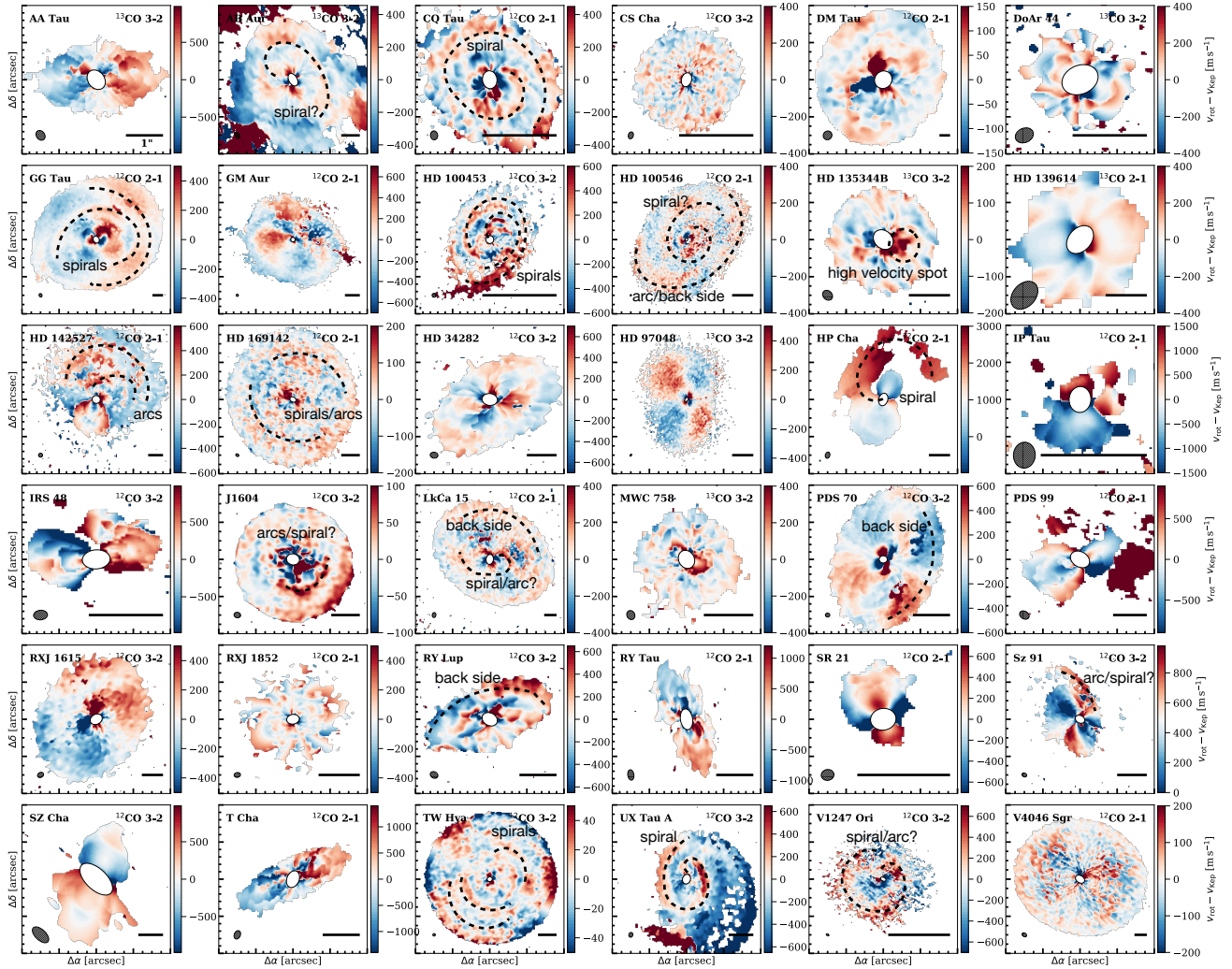
Fig. 6. Rotation velocity residuals obtained with eddy, shown for the main CO lines used in this analysis assuming a thin disc approximation. The circle and bar in the bottom left and bottom right corner of each panel indicate the beam and a 1'' scale, respectively. The main features are annotated.
