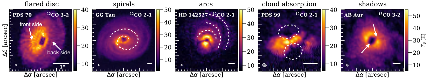
Fig. 2. Examples of the different features seen in the brightness temperature of our sources. The circle and bar in the bottom left and bottom right corner of each panel indicate the beam and a 1'' scale, respectively.
