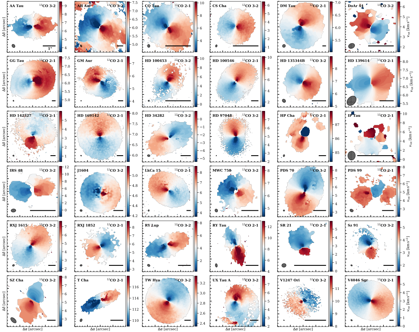
Fig. 3. Rotation velocity maps of the gas emission in our targets, shown for the main CO lines used in this analysis. The maps were computed with bettermoments . The circle and bar in the bottom left and bottom right corner of each panel indicate the beam and a 1'' scale, respectively.
