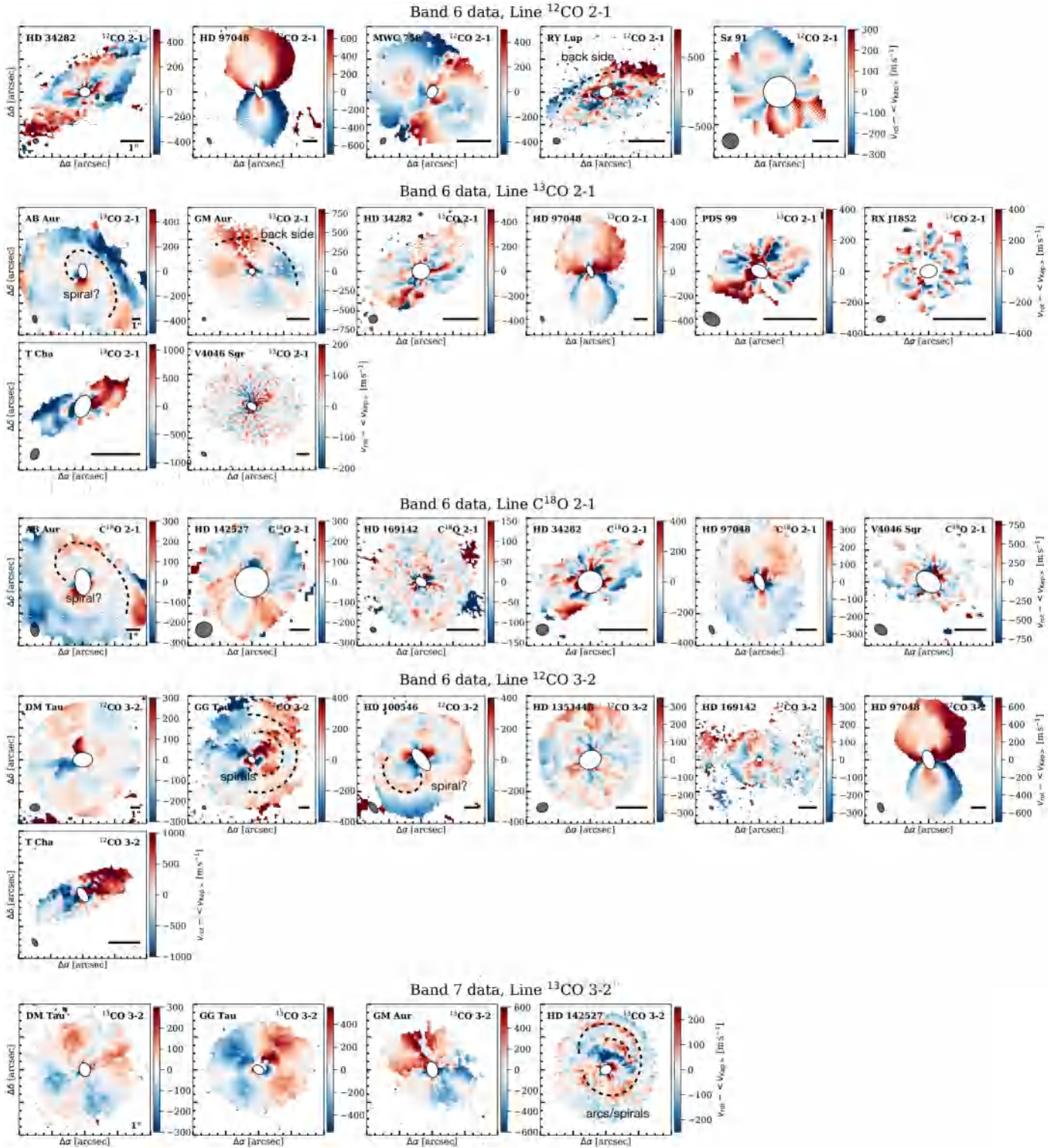
Fig. E.10. Rotation velocity residuals obtained with eddy, shown for the additional Band 6 and Band 7 lines used in this analysis and for a thick disc geometry. The circle and bar in the bottom left and bottom right corner of each panel indicate the beam and a 1'' scale, respectively. Some features are annotated.
