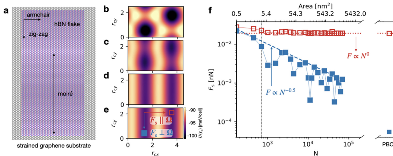
Fig. 7 Directional structural lubricity via strain engineering. (a) An aligned hBN flake on a graphene substrate strained by \varepsilon_{\text{armchair}} \approx 1.8\% in the armchair = \hat{x} direction. The aspect x : y ratio of the hBN flake is approximately 1 : 2. The wavelength of the linear moiré pattern is highlighted with a black arrow. (b–e) Corrugation potential U(r_c) for hBN flakes of size (b) 6.5 nm × 12.7 nm ( N = 170 ), (c) 13 nm × 25.5 nm ( N = 2760 ), (d) 39 nm × 76.5 nm ( N = 11120 ), (e) PBC in the region [0, 0.45 \text{ nm}] \times [0, 0.25 \text{ nm}] . Like in Fig. 6, N is the number of lattice cells, so that the flake consists of 2N atoms in total. (f) Static friction in the armchair lattice-matched direction (red empty symbols) and zig-zag (blue filled symbols), respectively parallel and perpendicular to the CLV \Omega . The dashed (dotted) line indicates the scaling in the direction parallel (perpendicular) to the energy corridors, as indicated in panel (e). The vertical dash-dotted black line marks the critical size N_c of the largest non-matching component \mathbf{G}' .
