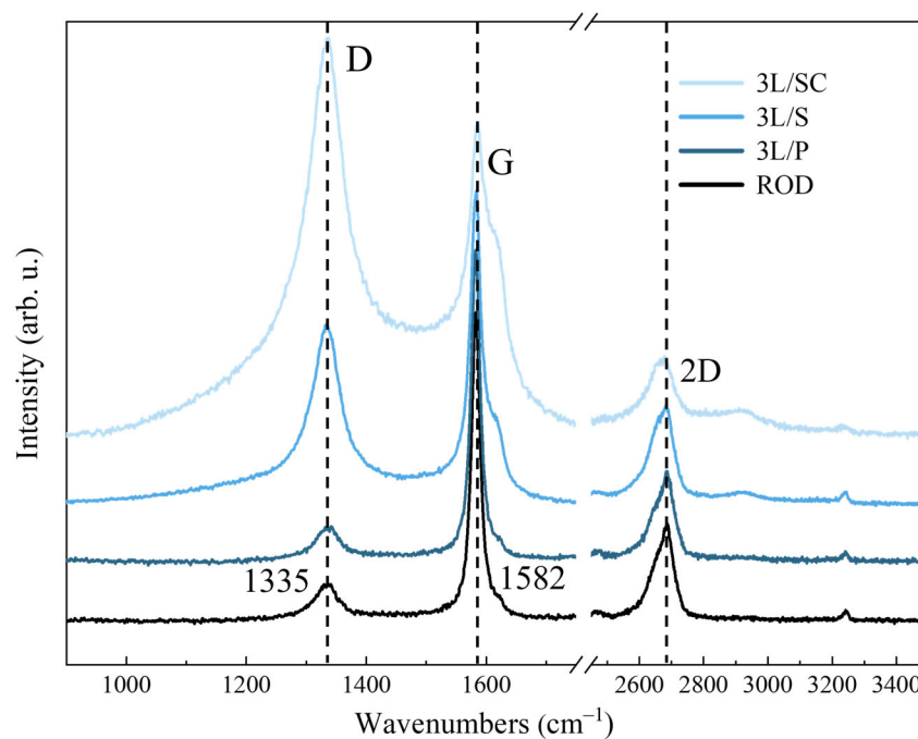
Figure 9. Raman ( \lambda_{\text{exc}} = 633 \text{ nm} ) spectra of the pristine synthetic graphite sample (ROD) and of the commercial 3L GNPs (3L/P: the pristine sample; 3L/S: the sample after sonication in water; 3L/SC: the sample after sonication and centrifugation).
