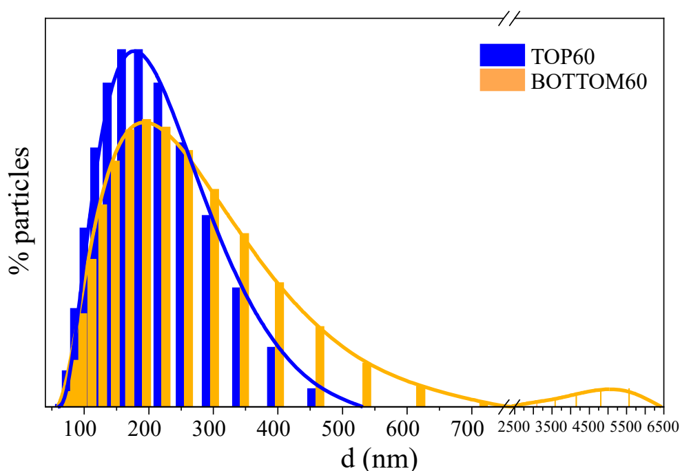
Figure 2. Dynamic light scattering (DLS) diameter ( d ) distribution curve of TOP60 and BOTTOM60.
