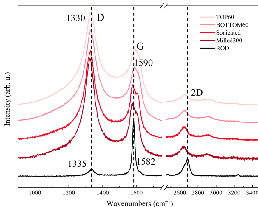
Figure 10. Raman spectra ( \lambda_{\text{exc}} = 633\text{ nm} ) of GNP samples at different preparation steps.
