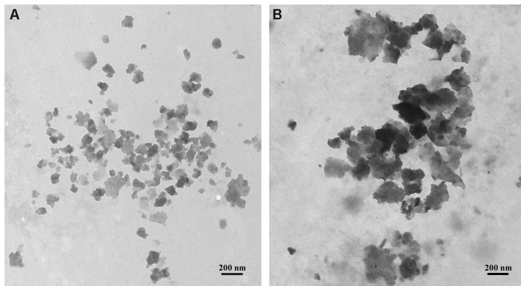
Figure 3. Representative transmission electron microscopy images of (A) TOP60 and (B) BOTTOM60 GNPs. Both nanoparticles show a similar irregular morphology while exhibiting a different lateral size. TOP60 GNPs have an average lateral dimension of 70 nm, while BOTTOM60 GNPs of 120 nm. Furthermore, BOTTOM60 nanoparticles exhibit a pronounced tendency to entangle with each other in a random manner, producing multilayer aggregates more frequently than TOP60 ones.
