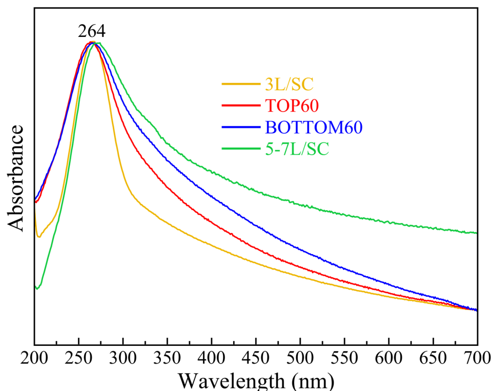
Figure 5. Comparison among normalized UV-vis absorption/extinction spectra of water dispersions containing commercial graphene nano-sheets (3L/SC, 5-7L/SC) and TOP60, BOTTOM60 GNPs.
