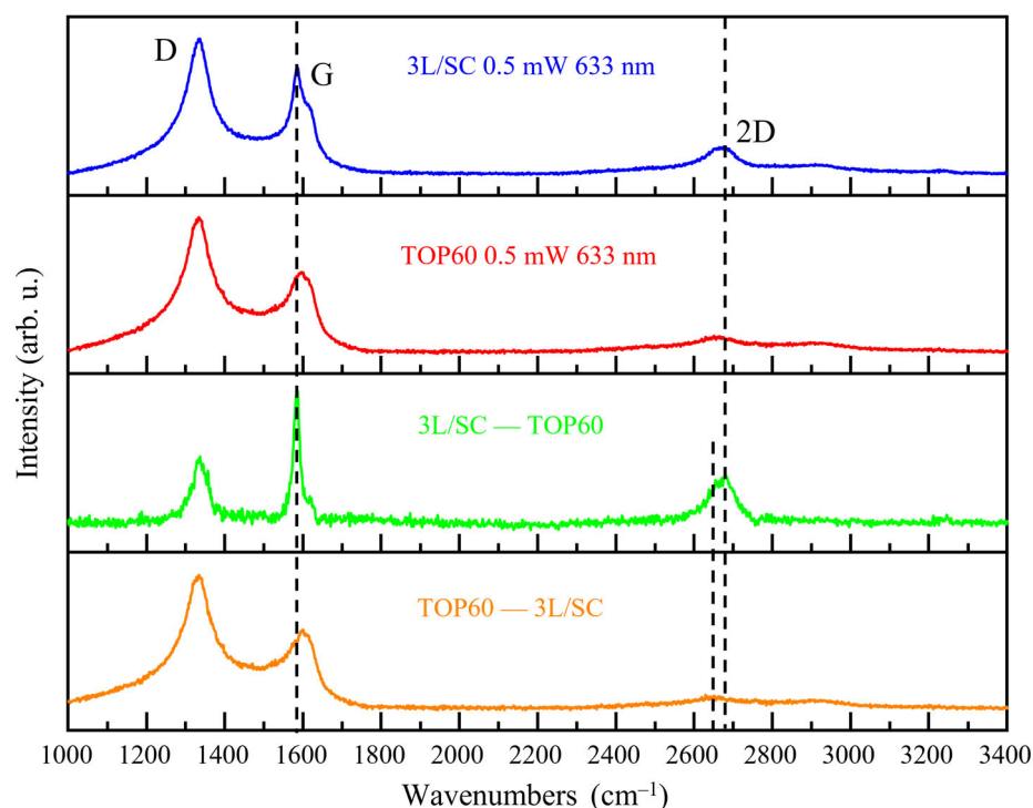
Figure 11. From the top to the bottom: Raman spectra of 3L/SC, TOP60, and subtraction spectra (3L/SC–TOP60) and (TOP60–3L/SC). Raman spectra were recorded with \lambda_{\text{exc}} = 633 nm, with 0.5 mW laser power.
