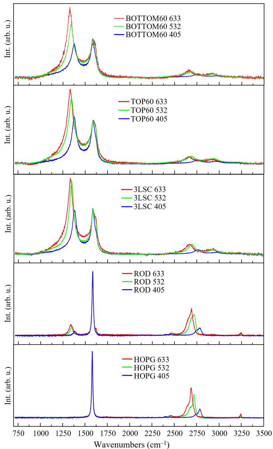
Figure 12. Multiwavelength Raman spectra ( \lambda_{\text{exc}} = 633, 532, 405 \text{ nm} ) of: TOP60, BOTTOM60, 3L/SC, ROD, HOPG samples.
