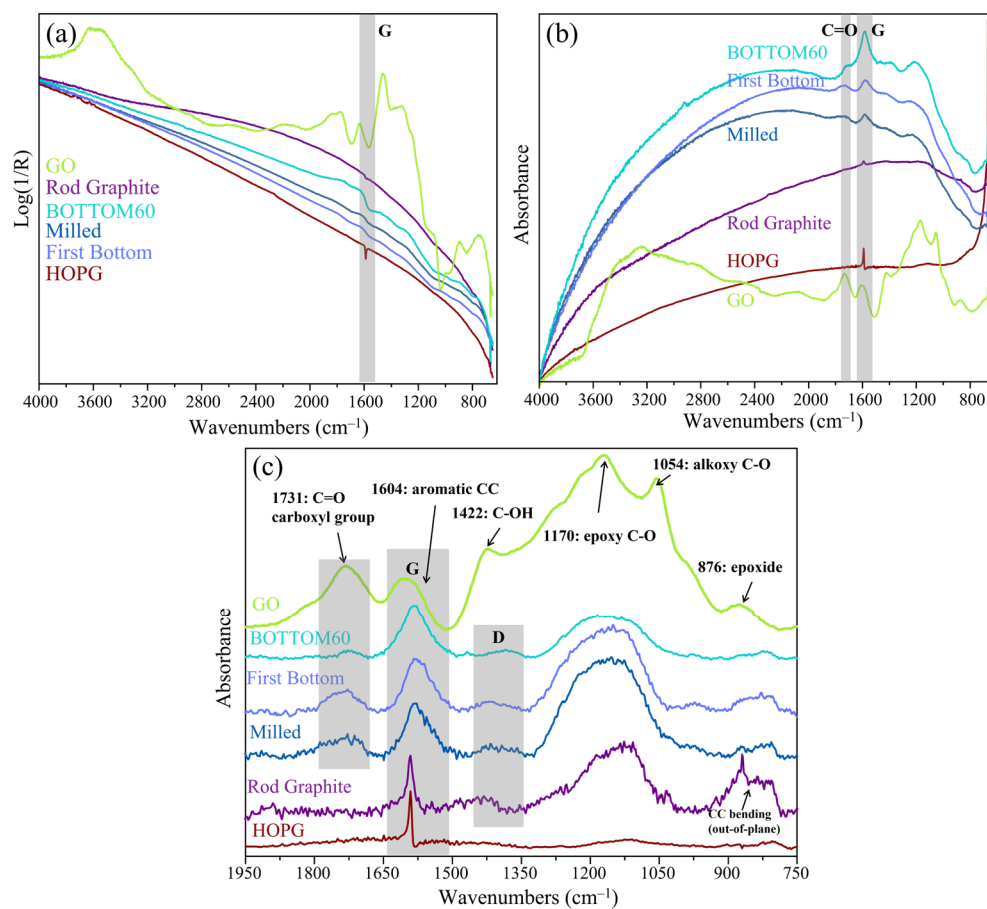
Figure 7. FTIR spectra of HOPG, ROD, GO, and GNPs samples at different preparation steps: (a) Specular reflection (SR) spectra; (b) absorption spectra from SR after Kramers–Kronig transformation; and (c) absorption spectra after baseline correction in the region 1950–750 cm -1 .
