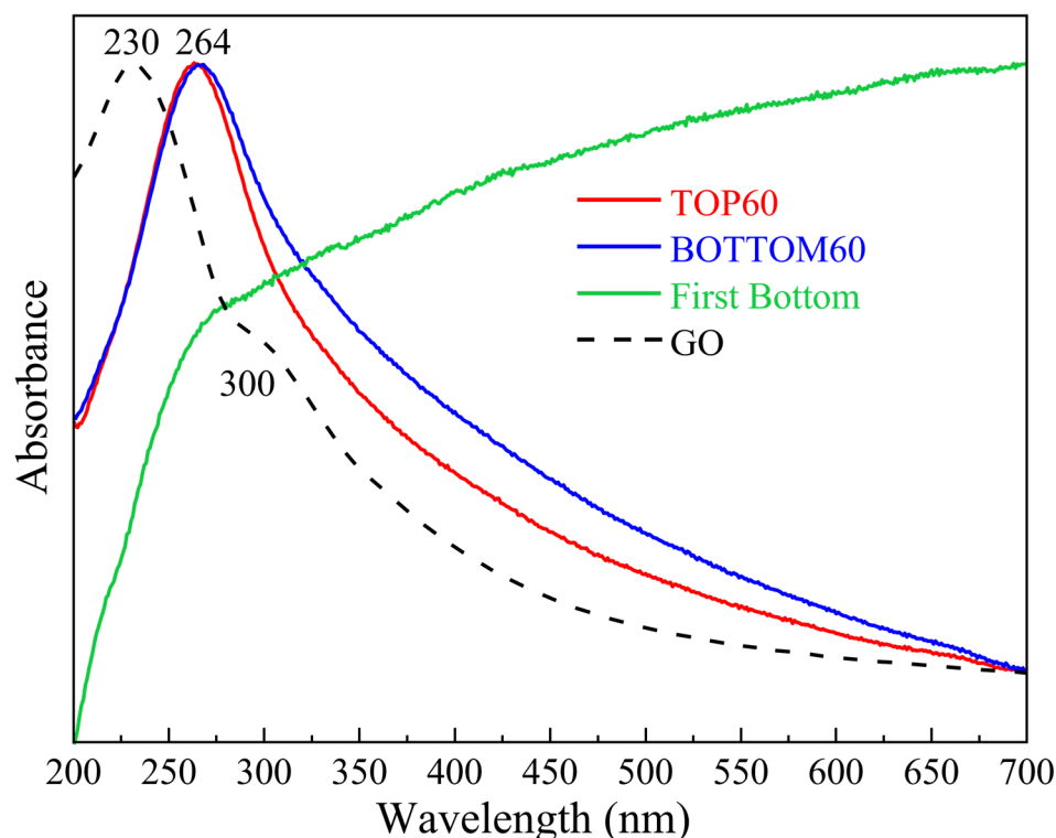
Figure 4. UV-vis normalized extinction/absorption spectra of the GNPs samples of TOP60, BOTTOM60, First BOTTOM and Graphene Oxide (GO).
