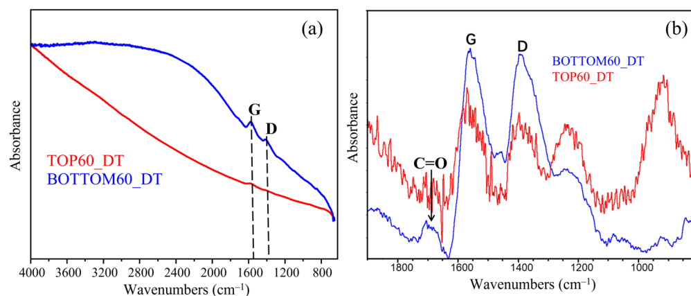
Figure 6. Normalized FTIR spectra of TOP60 and BOTTOM60 obtained in double transmission: (a) Spectra, as recorded; and (b) Spectra after baseline correction.
