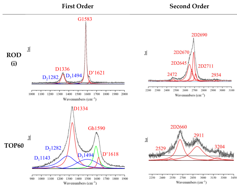
Figure 8. Result of the curve fitting (deconvolution) of the Raman spectra ( \lambda_{\text{exc}} = 633 \text{ nm} ) of ROD(i) sample and of TOP60 sample.
