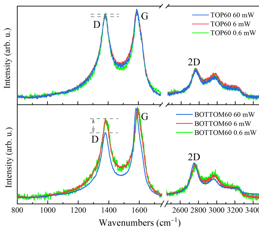
Figure 13. Raman spectra of the GNPs samples of TOP60 and BOTTOM60 excited by blue ( \lambda_{exc} = 405 nm) laser at different power values at the same point.
