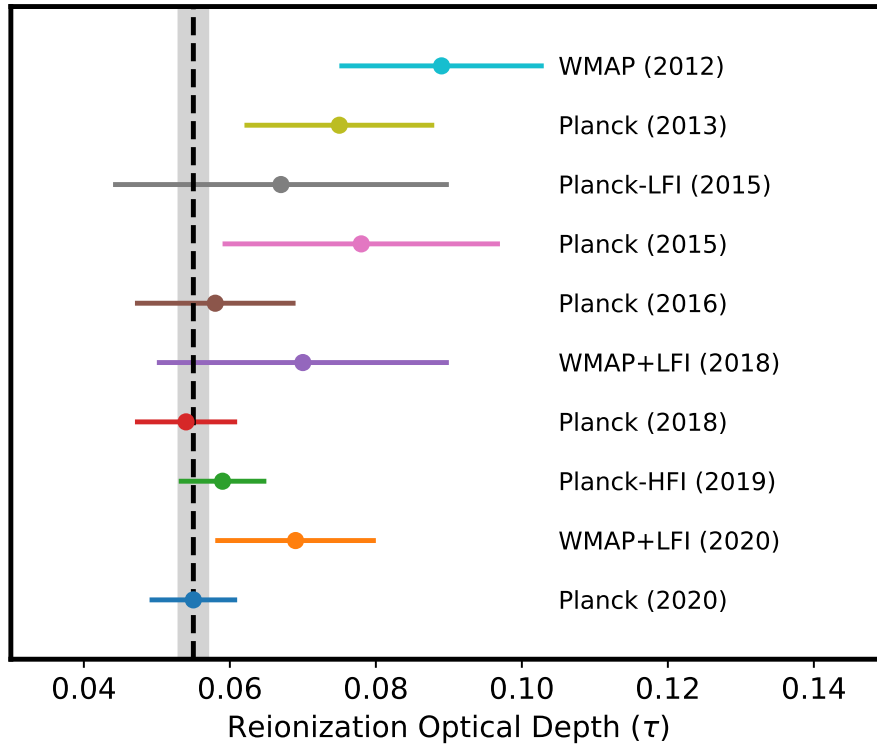
Fig. 48: Measurements of \tau based on the CMB power spectra: WMAP (2012) [75]; Planck (2013) [332]; Planck (2015) [289]; Planck (2016) [330]; WMAP+LFI (2018) [333]; Planck (2018) [279]; Planck-HFI (2019) [334]; WMAP+LFI (2020) [335]; and Planck (2020) [331]. The gray band shows the LiteBIRD uncertainty forecast for \tau .
