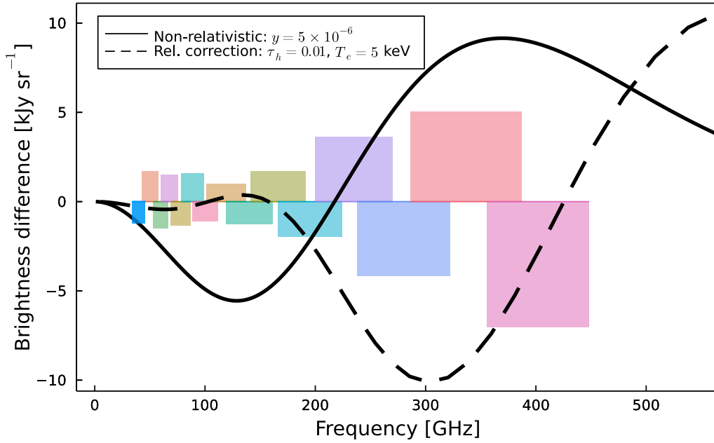
Fig. 51: Spectrum of the thermal SZ effect. The solid line shows the example spectrum in units of \text{kJy sr}^{-1} in the non-relativistic limit, k_{\text{B}}T_{\text{e}}/m_{\text{e}}c^2 \ll 1 , with y = \tau_{\text{h}}k_{\text{B}}T_{\text{e}}/m_{\text{e}}c^2 = 5 \times 10^{-6} . The dashed line shows the spectrum of the relativistic correction for \tau_{\text{h}} = 0.01 and k_{\text{B}}T_{\text{e}} = 5 \text{ keV} (which gives y = 9.8 \times 10^{-5} ) relative to the non-relativistic SZ effect with y = 9.5 \times 10^{-5} , calculated by the SZpack package [393, 394], i.e., the difference between the full and non-relativistic spectra in units of \text{kJy sr}^{-1} . We show the difference between the relativistic and non-relativistic SZ spectra with two different values of y to highlight the genuine effect of the relativistic correction, which cannot be absorbed by changing the value of y . The colored bars show the sensitivity of the 15 partially overlapping bands of the LiteBIRD detectors. For clarity we show half of the bands as positive and the other half as negative quantities, but only their absolute values are meaningful.
