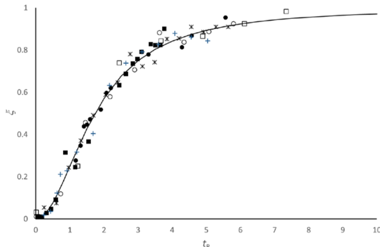
Figure 2. Gathered growth curves from a variety of microbes ( Lactobacillus delbrueckii subsp. bulgaricus , Streptococcus thermophilus , Salmonellae , C. jejuni , Pseudomonas fluorescens and Candida sake ) adjusted from [18]. For further data, see also Figure 2 in [21]
