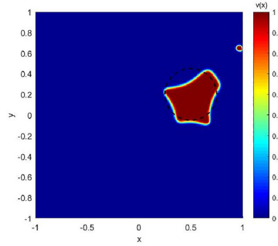
(b) (\mu, \lambda) = (0.2, 1) , \tau_n = 5 \times 10^{-4} . \tilde{\alpha} = 5 \times 10^{-2} , n = 14361 . Noise level 5%.
