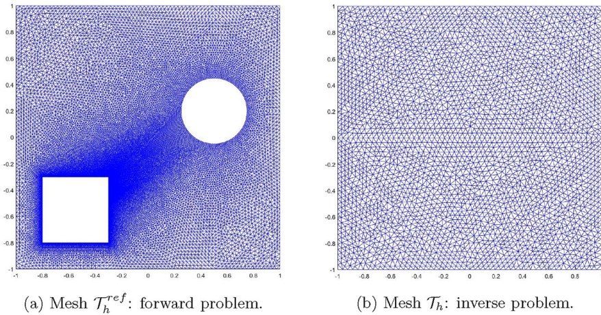
Fig. 1 Example of the meshes adopted
