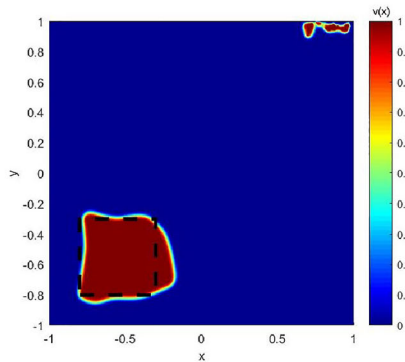
(d) (\mu, \lambda) = (0.5, 1) , \tau_n = 5 \times 10^{-4} . n = 15854 . Noise level 5%.
