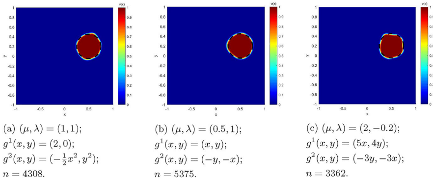
Fig. 4 Test 2. Reconstruction of a circular cavity using several parameters and data. For each experiment, we report the configuration at the final step n . Dotted line represents the target cavity
