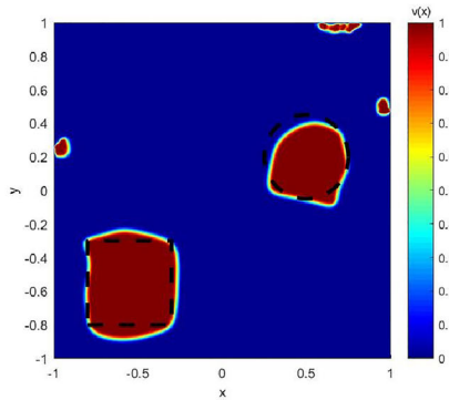
(f) (\mu, \lambda) = (0.5, 1) , \tau_n = 5 \times 10^{-4} . n = 25480 . Noise level 5%.
