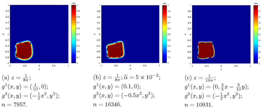
Fig. 5 Test 3. Reconstruction of a square-shaped cavity. Dotted line represents the target cavity
