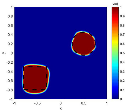
(e) (\mu, \lambda) = (0.5, 1) . n = 11776 . Noise level 2%.
