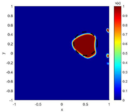
(a) (\mu, \lambda) = (0.2, 1) , \tau_n = 5 \times 10^{-4} . n = 11071 . Noise level 2%.
