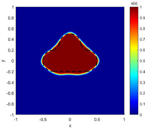
Fig. 7 Test 5. Reconstruction of a non-convex domain. It seems that the algorithm tends to reconstruct a convex domain. Dotted line represents the target cavity
