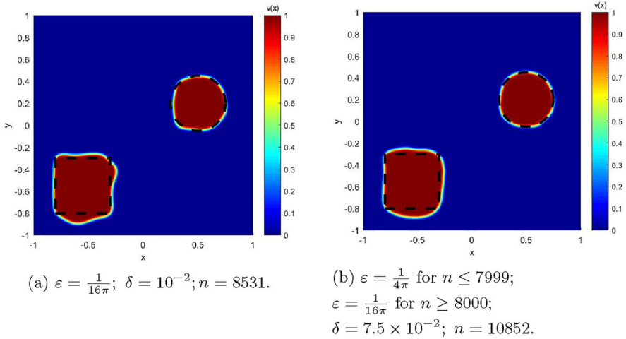
Fig. 6 Test 4. Reconstruction of two cavities. Dotted line represents the target cavity
