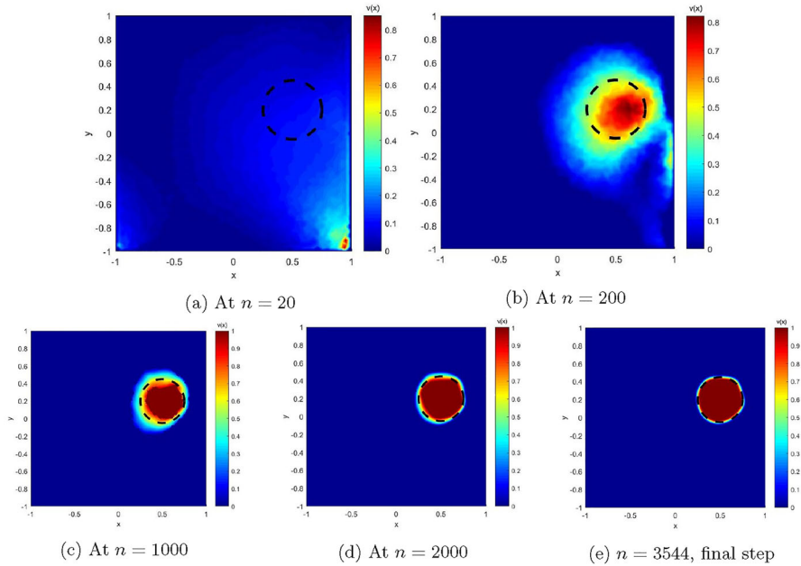
Fig. 3 Test 1. Reconstruction of a circular cavity. Dotted line represents the target cavity
