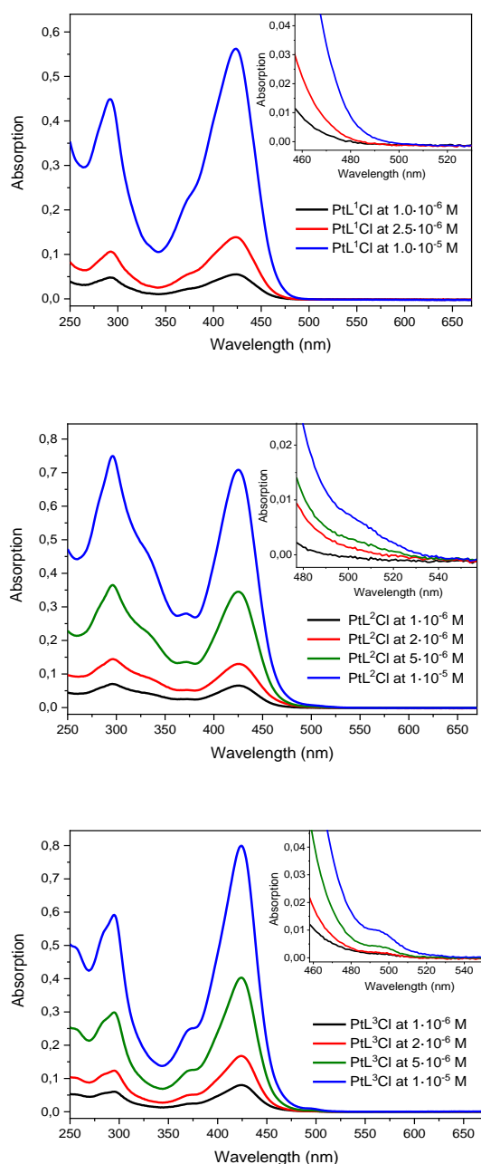
Figure 1. Absorption spectra at different concentrations of [PtL 1 Cl] , [PtL 2 Cl] and [PtL 3 Cl] in CH 2 Cl 2 at 298 K. The weak bands at longer wavelengths are shown on an expanded scale for clarity.
