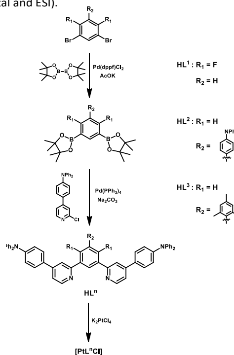
Scheme 2. Synthesis of [PtL n Cl].
