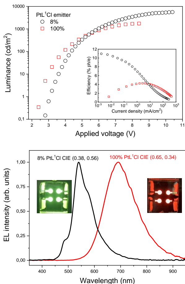
Figure 4 a) Luminance vs applied voltage and external EL efficiency vs current density (inset) of the OLEDs. b) Electroluminescence spectra at 7 V of OLEDs. In the inset there are photos of yellow-green and deep red OLEDs based on [PtL 1 Cl].
