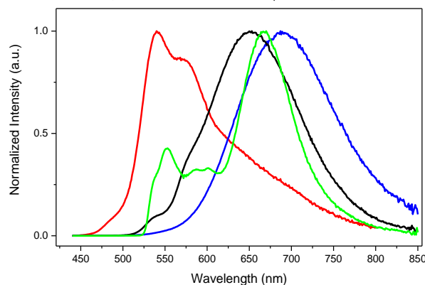
Figure 3. Normalized emission spectra of [PtL 1 Cl] complex in solid state.
