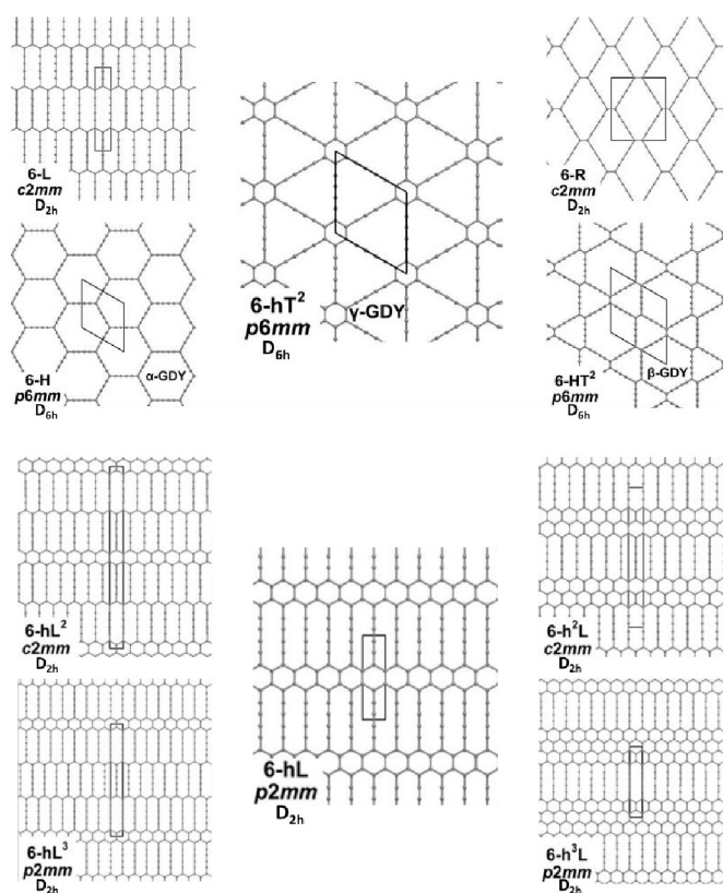
Figure 1: Sketch of the 2D-GDY (top) and 2D-GZY (bottom) structures analysed. For each structure, the unit cell, plane group and point group symmetry (factor group at I' point of BZ) are illustrated.
