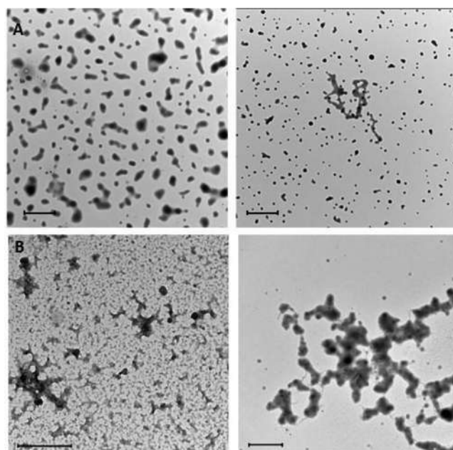
Figure 6. (A) TEM micrographs of F127@7-NPs doped with 10 (5% with respect to 7, average size 120 nm, PDI: 0.088 measured by DLS, left) and of F127@9-NPs doped with 10 (5% with respect to 9, average size 102 nm, PDI: 0.088 measured by DLS; right) incubated at 37 °C for 1 h in 10 mM glutathione. (B) TEM micrographs of F127@7-NPs doped with 10 (5% with respect to 7, average size 110 nm, PDI: 0.046 measured by DLS) incubated at 37 °C for 24 h in 10 mM glutathione (left) and 10 mM DTT (right). Scale bars: 1 \mu\text{m} (A), 500 nm (B, left), and 2 \mu\text{m} (B, right).
