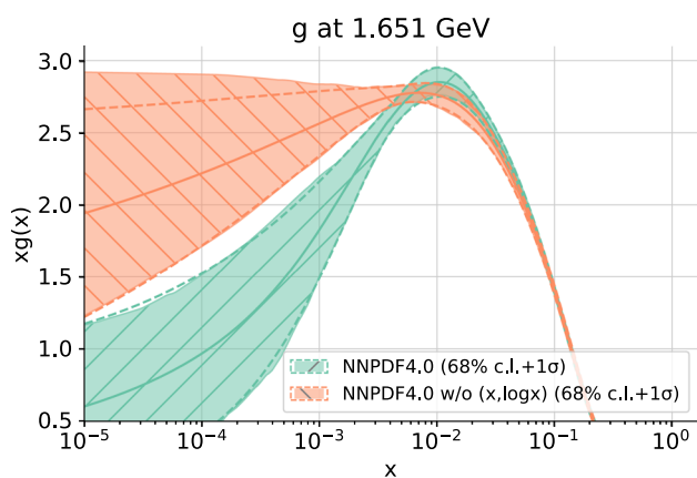
Fig. 2 Comparison between the gluon PDF generated with the standard NNPDF4.0 methodology (green) and our modification in which we have removed the splitting layer of x to (x, \log x) (orange). While we observe good compatibility between both PDFs in the large- x region, as we enter in the small- x region our modified PDF saturates. This is evident also in the \chi^2 of the modified fit which was blocked at \chi^2 = 1.20 while NNPDF4.0 is able to get it down to \chi^2 = 1.16
