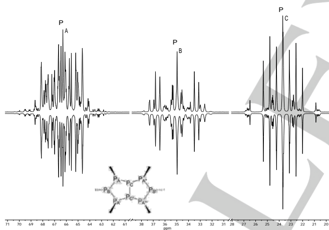
Figure 1. Experimental (top) and simulated (bottom) ^{31}\text{P}\{^1\text{H}\} NMR spectrum of octaphosphane 2 (AA'A''A'''BB'CC' spin system with C_{2v} symmetry). Chemical shifts in ppm: \delta(P_A) = +66.3 , \delta(P_B) = +35.0 , \delta(P_C) = +23.7 . Selected coupling constants in Hz: ^1J_{AB} = -292.30(3) , ^1J_{AC} = -262.67(3) , ^1J_{CC'} = -311.99(12) , ^2J_{AA''} = +143.18(8) .
