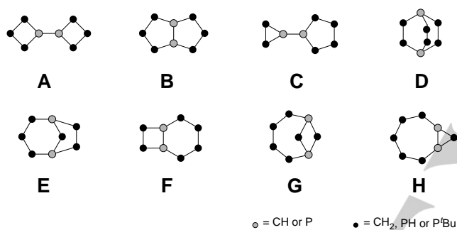
Scheme 4. Possible constitutional isomers of C 8 H 14 , P 8 H 6 or P 8 tBu 6 precluding multiple bonds.
