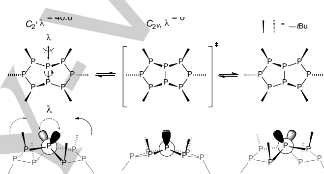
Scheme 3. Libration of octaphosphane 2 . The transition state corresponds to the average structure in solution. The remaining structures (left and right) correspond to the enantiomeric structure found in the solid state.
