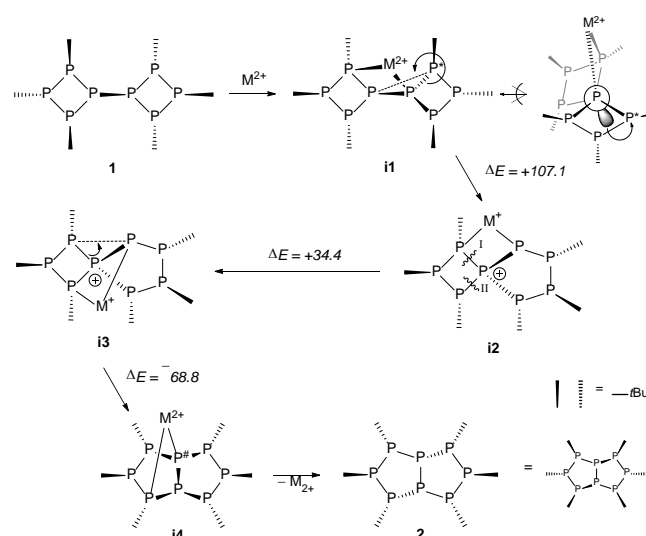
Scheme 1. Isomerization reaction between octaphosphane 1 and 2 as well as for the isolobal bi(cyclobutane) to bicyclo[3.3.0]octane (pentalane) and bicyclo[3.2.1]octane.
