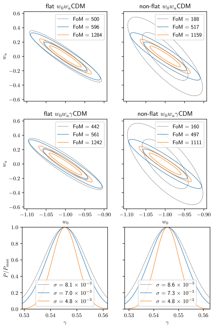
Fig. 7. Predicted 1D and 2D marginalised distributions for the w_0 – w_a and/or \gamma parameters, for four cosmological model: flat w_0 w_a CDM (top left); non-flat w_0 w_a CDM (top right); flat w_0 w_a \gamma CDM (middle and bottom left); and non-flat w_0 w_a \gamma CDM (middle and bottom right). This is for the same scenario as Fig. 6, using the same colour coding (where Euclid -only constraints are here in dashed black). Each plot is accompanied by the corresponding FoM or 1\sigma uncertainties.
