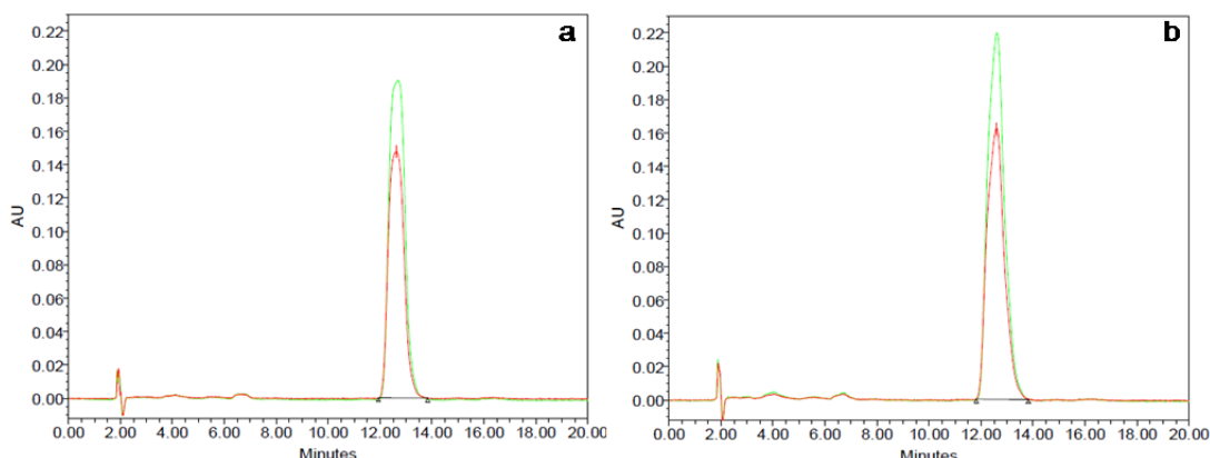
Figure 2: HPLC-UV/Vis chromatograms at 470 nm of acetone extracts from untreated (red curve) and PEF treated (5 kV/cm; 5 kJ/kg, green curve) tomato peels at 20°C (a) and 50°C (b) of extraction temperature.
