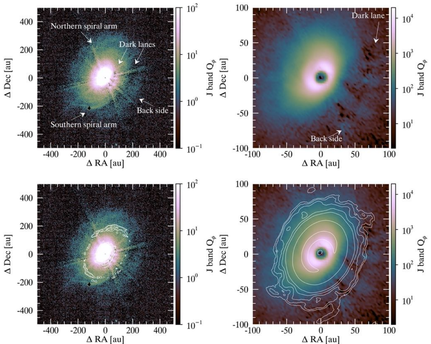
Fig. 4. VLT/SPHERE IRDIS polarimetric observations of HD 100546 (from Sissa et al. 2018 ) showing the large-scale (left) and small-scale (right) structures. The main substructures are overlaid in the top panels. The ALMA 870 \mu\text{m} contours are overlaid in the bottom panels.
