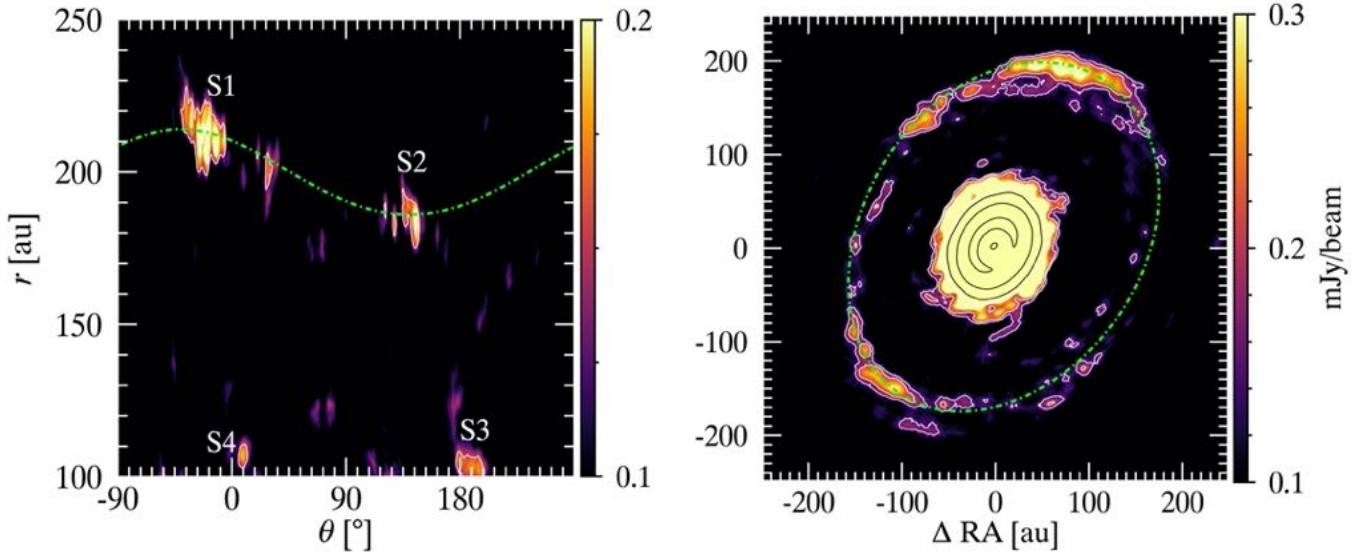
Fig. 3. Eccentricity of the outer ring. ( left ) Surface brightness of the outer disk region in polar coordinates after de-projection and subtraction of a Gaussian ring centered at r = 200 au. The dot-dashed green line is the best fit of the outer ring with an eccentricity of 0.07 (see Sect. 4 for details). ( right ) Surface brightness with the eccentric ring overlaid.
