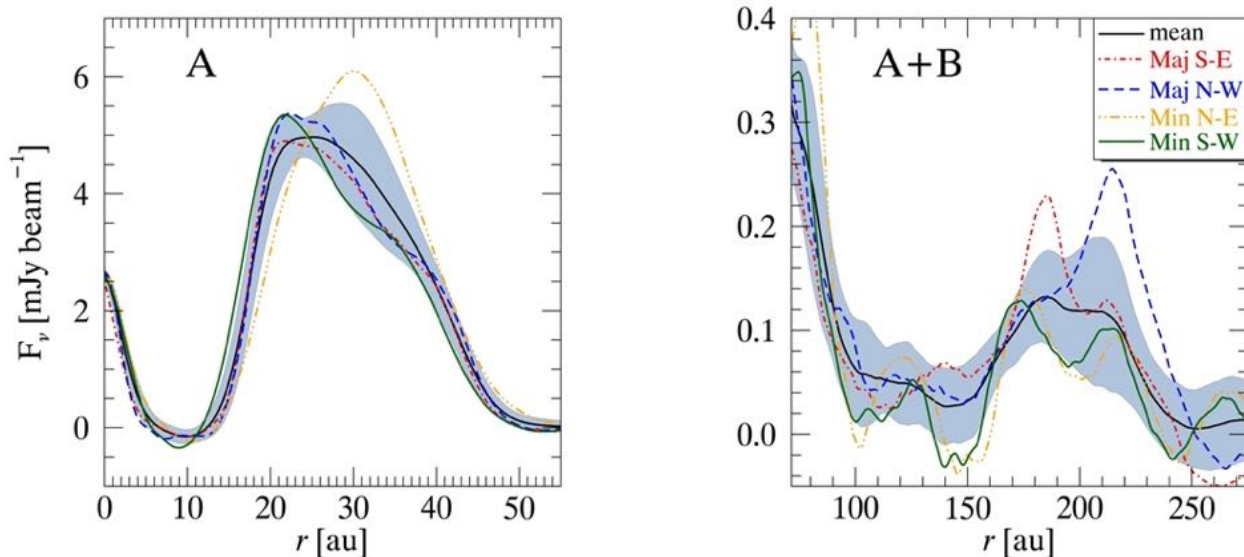
Fig. 2. Surface brightness profiles of the inner (left, from data set A) and outer (right, combined data sets A+B) disk of HD 100546. The black curve and the gray region represent the azimuthally averaged profile and standard deviation obtained after de-projecting the images by 42^\circ . The profiles along the semimajor and semiminor axes are overplotted in color; they were obtained by averaging the radial profiles over a range of \pm 10^\circ around the corresponding axis.
