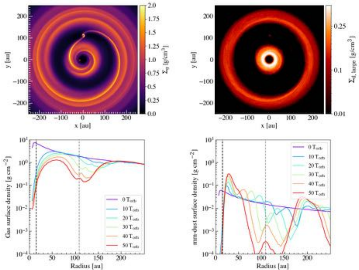
Fig. 5. SPH results. ( top ) Surface density of gas and 1 mm dust grains after t = 50 T_{\text{orb}} . The positions of the planets are shown as red dots in the left panel. ( bottom ) Temporal evolution of the azimuthally averaged surface density profiles. The final positions of the two planets are indicated by the vertical dashed lines. The shape of the outer gap, both in gas and in dust, reflect the radial migration of the planet.
