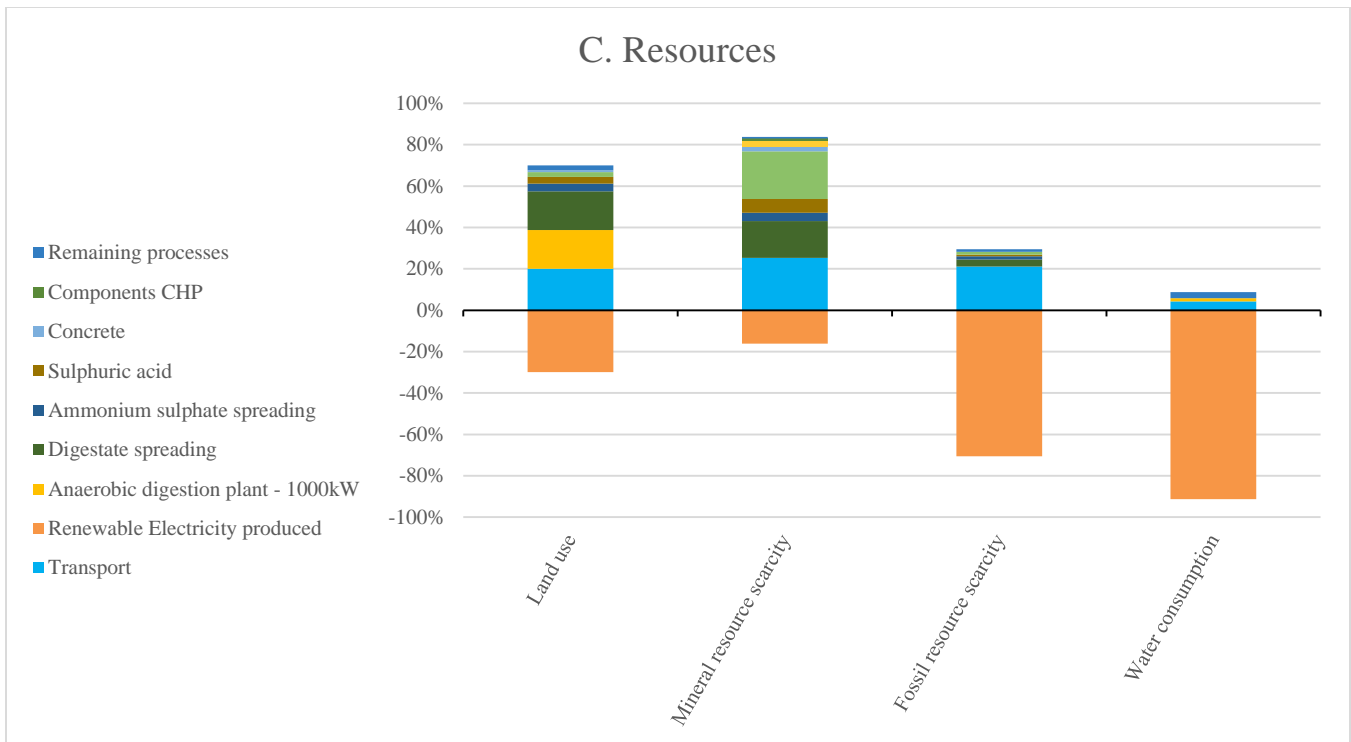
Figure 3. Process contribution to impact categories of Scenario RF, focusing on the ecosystem (a), toxicity (b) and resources (c). Impacts assessments were calculated according to ReCiPe 2016 midpoint (H) V 1.03 method and data reported as percent of the total impact.
