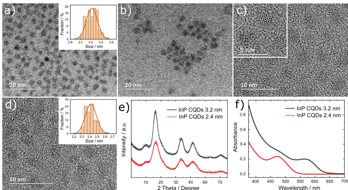
Figure 1. TEM images of the: 3.2 nm InP CQDs a) before and b) after ligand exchange, c) magnified view of as synthesized CQDs (the inset shows a further magnification); d) 2.4 nm InP CQDs. Figure 1a and 1d report the CQDs size distribution of the two nanocrystal sizes. e) X-ray powder diffraction (XRPD) diffractograms and f) UV-Vis spectra of the 3.2 and 2.4 nm CQDs.
