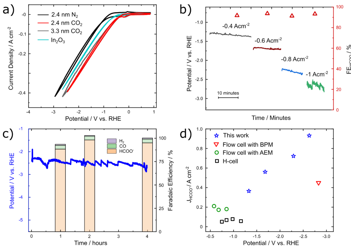
Figure 2. a) Current-voltage characteristics of cathodes containing \text{In}_2\text{O}_3 nanoparticles (100 nm size) as control material, \text{InP} CQDs of two sizes using 30 mL of 1 M KOH electrolyte, in the presence of \text{CO}_2 or \text{N}_2 with 50 \text{ cm}^3 \text{ min}^{-1} flow rate. b) Chronopotentiometry as we step the current density from -0.4 to -1 \text{ A cm}^{-2} . Each step was recorded with a fresh \text{CC}/\text{InP} electrode containing 20 \mu\text{g cm}^{-2} of CQDs with 30 mL of 3M KOH electrolyte and with a \text{CO}_2 flow rate of 50 \text{ cm}^3 \text{ min}^{-1} . To maintain a consistent sampling time at each current density, a catholyte sample for HPLC analysis was collected after a charge equal to 480 Coulomb was passed through the electrolyzer, see Supporting Information for details. Formate FE for each current density (red triangles) is reported on the right axis. All potentials are not iR corrected. c) 4-hour chronopotentiometry at -400 \text{ mA cm}^{-2} (blue trace and left Y axis) and Faradaic efficiencies (right axis) at different sampling times recorded with the \text{CC}/\text{InP} electrode loaded with 20 \mu\text{g cm}^{-2} of CQDs with 200 mL 1 M KOH catholyte and anolyte. d) comparison of current density for formate in 3 M KOH (open blue stars) relative to selected formate current density reported in the recent literature for H-cells (open black squares), flow cells with anion exchange membrane and solid state electrolyte (open green circle) and a flow cell with bipolar membrane (the potential is estimated from the cell potential reported by the authors) see Table SI7 and Figure S7 for details.
