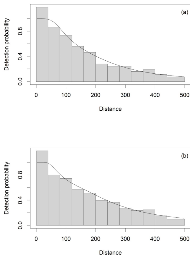
Figure 1 – Probability density from Hazard-rate detection function with simple polynomial adjustments returned by the best fitting model for the distances collected with MCDS for first (a) and second (b) distance sampling occasion to estimate red deer PG density on summer pastures of the Stelvio National Park during June-September 2020.
