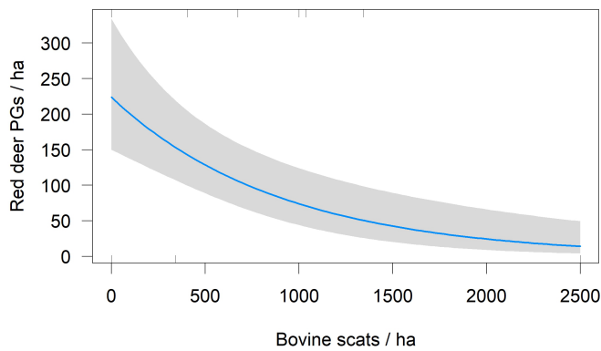
Figure 2 – Marginal effect of bovine scat density (Bovine scats/ha) on the expected deer scat density (Red deer PGs/ha) on summer pastures of the Stelvio National Park in 2020. The grey shaded area indicates 95% confidence interval.
