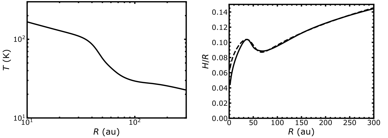
Fig. C.1. Left: density-weighted, vertically integrated disk temperature profile from the MCRT iterations described in Sec. 4.1. Right: disk aspect ratio H/R corresponding to the temperature profile in the left panel, adopting a stellar mass of 1.25 M_{\odot} and a mean molecular weight of 2.4. The dashed curve shows a fit to the profile between 30 and 300 au, as expressed by Eq. 3.
