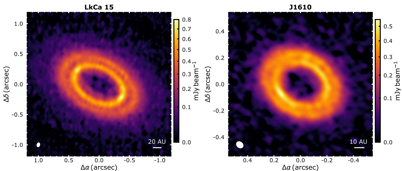
Fig. 1. Intensity maps of LkCa 15 (left panel) and J1610 (right panel). Note the different angular scales of the two panels. The color scale has been stretched to highlight the fainter regions of the disks.
