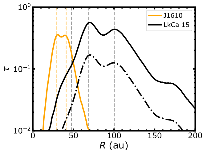
Fig. 8. Optical depth profiles of both disks derived from Eq. 5. The solid curves show the optical depth profiles assuming the temperature profile from Eq. 6. The dashed-dotted line portrays the optical depth profile of LkCa 15 obtained with the temperature profile calculated with the radiative transfer model (see Sec. 4 and Eq. 3). The optical depth profiles have been computed assuming absorption opacities only. The vertical dashed lines indicate the rings locations as derived from the (u, v) -plane modelling.
