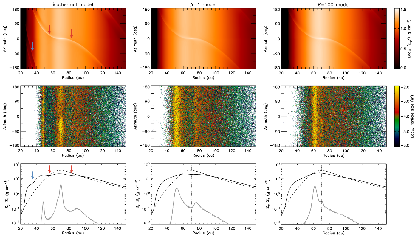
Fig. 6. Two-dimensional distributions of (upper panels) gas and (middle panels) particles in a radius - azimuthal angle plane. The lower panels show azimuthally-averaged radial profiles of gas (solid black lines) and dust (solid gray lines) surface density. The black dashed curves present the initial gas surface density profile, while the black dotted lines present the radial location of the planet. In the isothermal model, the red and blue arrows indicate the location of the shocks due to the primary (red) and secondary (blue) spiral arms. From left to right: (left) isothermal model, (middle) \beta = 1 model, and (right) \beta = 100 model. The planet is located at (R, \phi) = (70 \text{ au}, 0^\circ) . The disk rotation is upward in the upper and middle panels.
