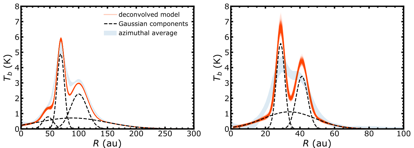
Fig. 3. Deconvolved brightness temperature radial profiles of LkCa 15 (left panel) and J1610 (right panel), calculated in the Rayleigh-Jeans approximation (see Sec. 3.2). The red curves show 800 random realizations of the posterior distribution of the GALARIO model, while the dashed black lines indicate the best fit of the Gaussian components used in the model. The underlying blue shaded region shows the deprojected and azimuthally averaged brightness temperature profile derived from Fig. 1 (see Sec. 3.1).
