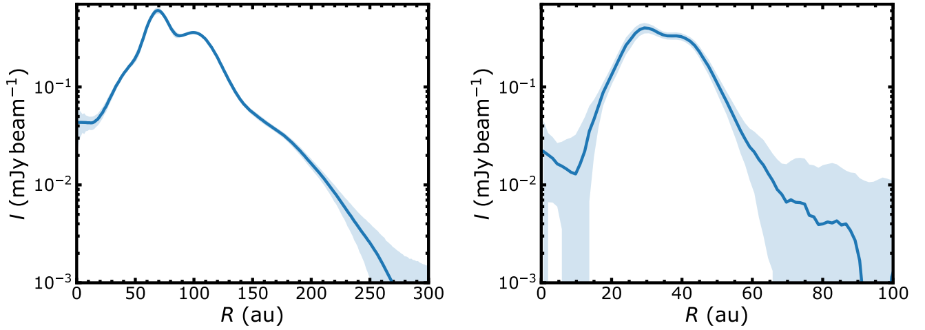
Fig. B.1. Deprojected and azimuthally averaged radial intensity profile of the continuum emission of LkCa 15 (left panel) and J1610 (right panel) as in Fig. 2. The blue ribbon shows the quadratic sum of the standard deviation of the intensity across pixels in each radial bin and the rms of the observations divided by the square root of the number of independent beams sampling the same radial bin in the azimuthal direction.
