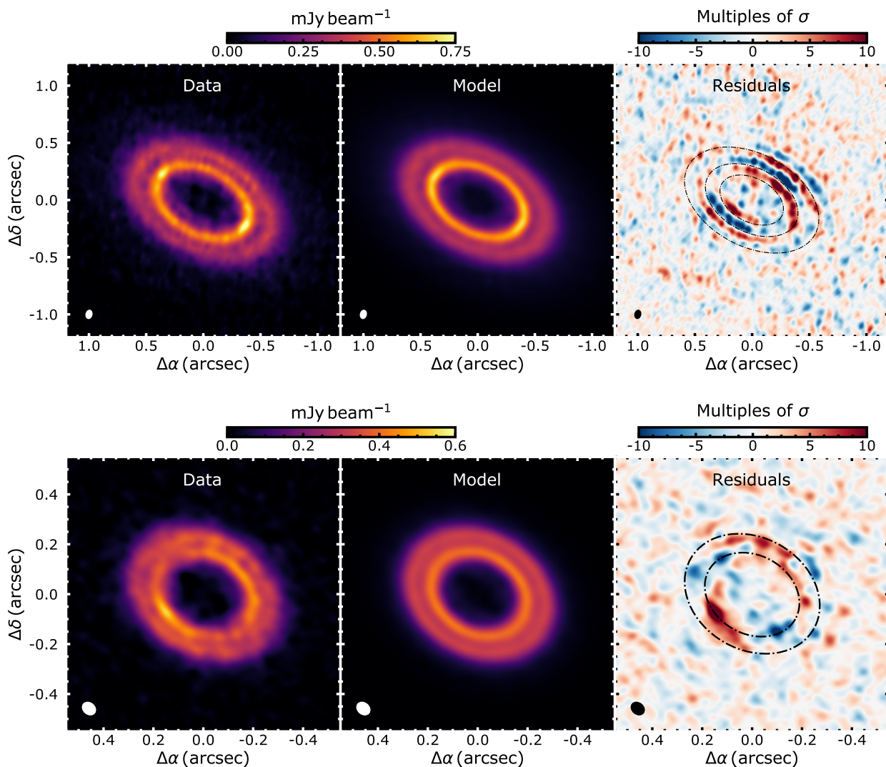
Fig. 4. From left to right: intensity map of the data, best fit model and residual visibilities for LkCa 15 (top) and J1610 (bottom). The intensity map of the best fit model and residuals have been generated using the same uv-sampling as the original data. In the residual map, the black dashed-dotted lines show the location of the rings (see Tables 2 and 3).
