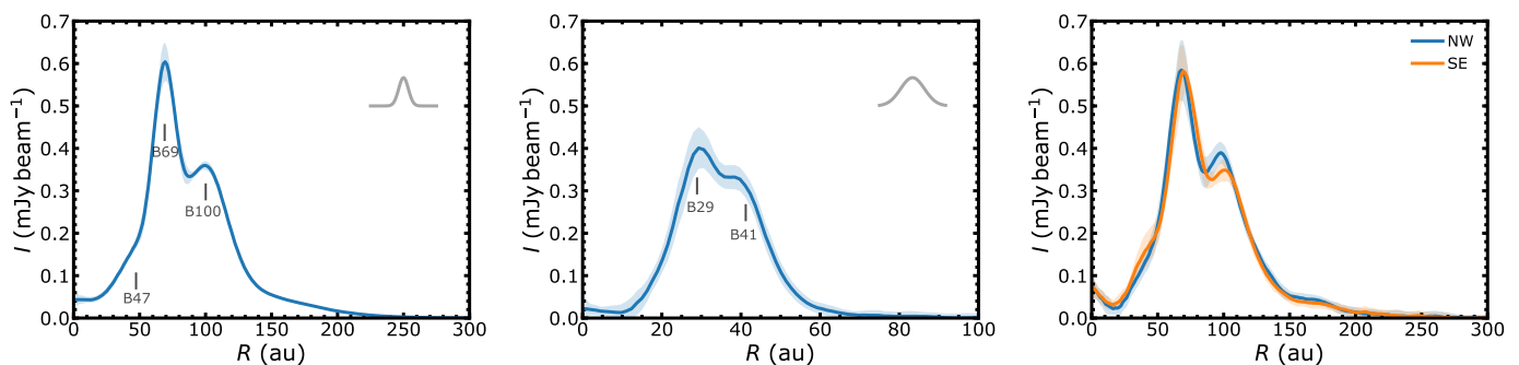
Fig. 2. Left and middle: deprojected and azimuthally averaged radial intensity profile of the continuum emission of LkCa 15 (left) and J1610 (middle). The ribbon shows the quadratic sum of the standard deviation of the intensity across pixels in each radial bin and the rms of the observations divided by the square root of the number of independent beams sampling the same radial bin in the azimuthal direction. The Gaussian profile in the top right corner of the panels shows the FWHM of the average of major and minor axis of the synthesized beam. Right: azimuthal average of the South-East, North-West sides of LkCa 15, respectively, where the disk has been divided in two sub-regions along the major axis. The inner shoulder is more prominent in the South-East side of the disk.
