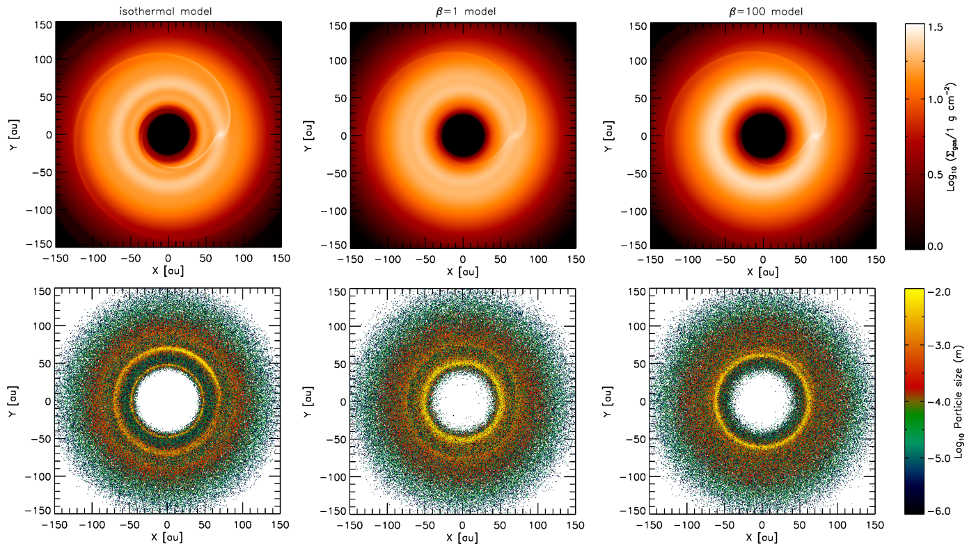
Fig. 5. Two-dimensional distributions of (upper panels) gas and (lower panels) particles. From left to right: (left) isothermal model, (middle) \beta = 1 model, and (right) \beta = 100 model. The planet is located at (X, Y) = (70 \text{ au}, 0 \text{ au}) . The disk and planet orbit clockwise about the central star.
