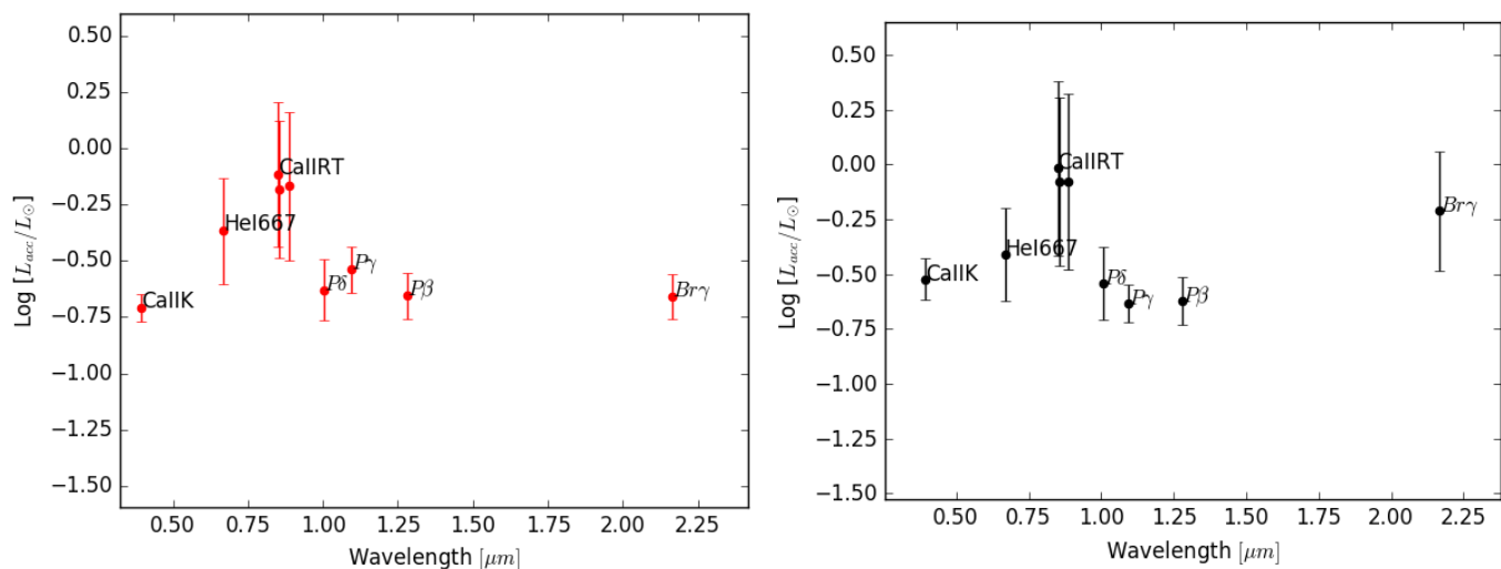
Fig. 9. Left: Accretion luminosities versus wavelength for the bright state. The fluxes of the optical lines have been corrected for A_V=0.4 (White & Ghez 2001). Right: Accretion luminosities versus wavelength for the dim state. The fluxes have been corrected for the observed extinction curve of Fig. 7.
