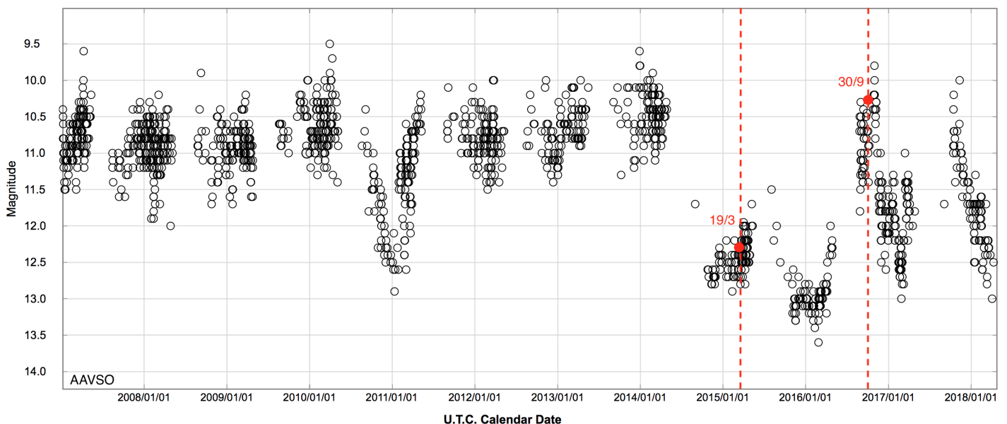
Fig. 1. Light curve of the RW Aur system in the visual. The plot is taken from The American Association of Variable Star Observers (AAVSO). The red dots indicate the time of our observations. The magnitudes for the two epochs were computed by producing synthetic photometry from the spectra.
