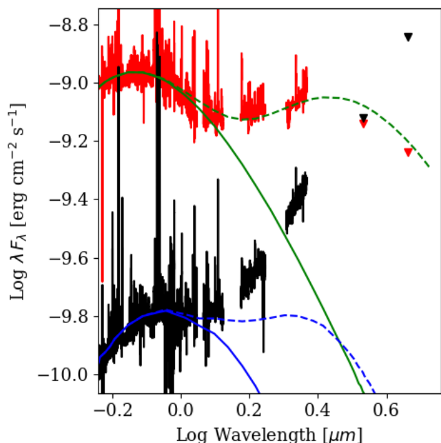
Fig. 8. X-Shooter spectral energy distribution of the bright state is shown in red. The red triangles show the WISE flux obtained in March 2014, when RW Aur A was in a bright state, assuming that half of the flux is contributed by RW Aur B, which is included in the WISE beam. The green curves show the photosphere, approximated by a black-body with T = 4900 K and L = 1L_{\odot} , and the total emission of the photosphere plus an additional black-body at T = 1180 K and \text{area} \sim 5.6 \times 10^{24} \text{ cm}^2 . The X-Shooter spectrum in the dim state is shown in black. The black triangles are the WISE fluxes, computed assuming that RW Aur B does not vary during the period of the observations. The blue curves show the photosphere and the best-fitting model of the bright state emission reddened according to the extinction curve derived in Sect. 3.3.
