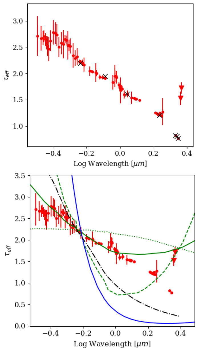
Fig. 7. Top panel: Effective optical depth of the dimming layer vs. wavelength computed from the ratio of the dim to the bright X-Shooter spectra. The red circles are the median of the values over intervals of 5 \text{ \AA} , the error is the standard deviation within the interval. The triangles show the optical depth derived from the ratio of the CO bandheads, computed as the median of three points around the peak of the first two bandheads. The black crosses correspond to continuum points in the spectrum. Bottom panel: The red points (circles and triangles) are the same as in the top panel. The black dashed line is the Cardelli extinction law for R_V = 3.1 (Cardelli et al. 1989). The green curves plot Q_{\text{abs}} (dashed), Q_{\text{scat}} (dotted), and Q_{\text{tot}} = Q_{\text{abs}} + 0.12Q_{\text{scat}} (solid) for a distribution of olivine with minimum and maximum size a_{\min} = 0.1 \mu\text{m} , a_{\max} = 150 \mu\text{m} , q = 3 (see text). The blue curve plot Q_{\text{tot}} = Q_{\text{abs}} + Q_{\text{scat}} (solid) for the same material, a_{\min} = 0.06 \mu\text{m} , a_{\max} = 0.1 \mu\text{m} , q = 3 . All curves are normalised to the observed optical depth at 0.58 \mu\text{m} .
