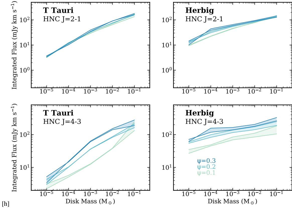
Fig. E.1. Disk-integrated line fluxes (calculated at a distance of 150 pc) of HNC J=2-1 and J=4-3 as a function of disk mass (left for disks around T Tauri stars, and right for Herbig stars). Colors represent different levels of disk flaring. Upper and lower panels: different transitions.
