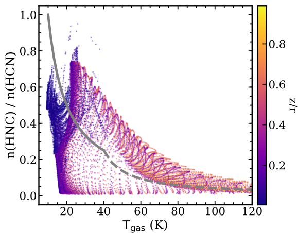
Fig. 6. Extracted HNC and HCN abundance ratio and the corresponding gas temperature for all models with M_{\text{gas}} = 0.01 M_\odot , color-coded by scale height z/r . Only grids with an HNC gas number density higher than 1 \times 10^{-5} \text{ cm}^{-3} are selected. The line ratio-gas temperature correlations from Hacar et al. (2020) are overplotted as gray curves.
