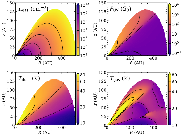
Fig. 1. Two-dimensional profiles of gas density, UV flux, dust temperature, and gas temperature for our fiducial model: a 10^{-2} M_{\odot} disk with \psi = 0.2 , h_c = 0.1 surrounding a T Tauri star. The UV flux is plotted in units of the mean interstellar radiation field ( G_0 , Draine 1978 ). Temperature only shows a limited range to highlight the cold outer disk region.
