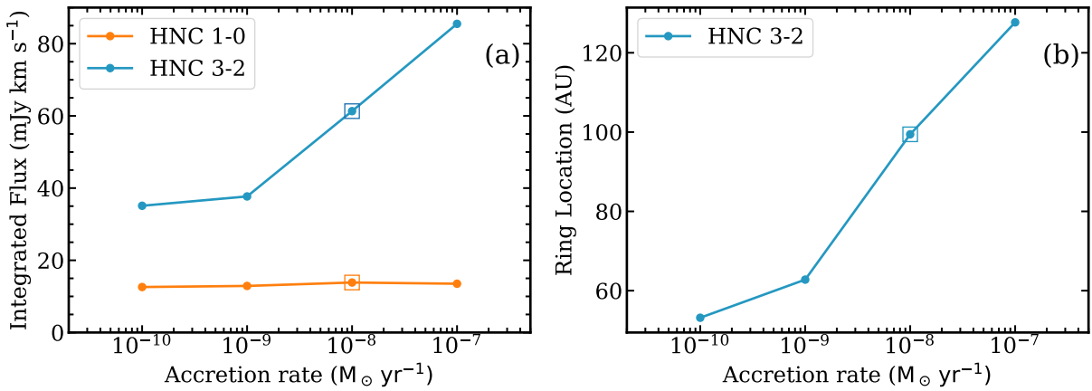
Fig. B.2. (a) Disk-integrated line fluxes for models with different accretion rates, which are a measure of UV luminosity. (b) Emission peak location change for the HNC 3–2 line, which is sensitive to UV radiation. The fiducial model results are marked as open squares.
