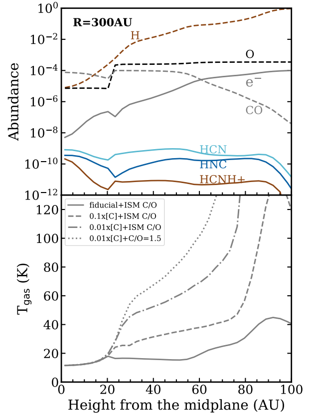
Fig. 10. Top: abundance profiles along the vertical disk direction at the radius of 300 \text{ au} for HNC and HCN in the fiducial model, as well as species relevant to their formation ( \text{HCNH}^+ and e^- ) and destruction (H and O). The drop in CO abundance in the top layer reflects where CO photodissociation becomes important. Bottom: gas temperature profile along the vertical disk direction at 300 \text{ au} for the fiducial model (solid line), as comparisons to carbon and oxygen depletion models (dashed line: a factor of 10; dash-dotted line: a factor of 100; and dotted line: \text{C/O}=1.5 ).
