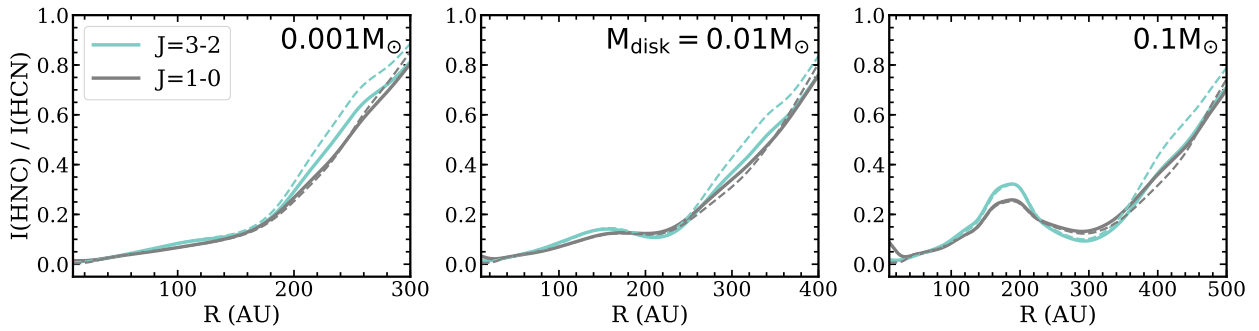
Fig. 5. Radial profiles of HNC-to-HCN line intensity ratio for the two transitions for the R_c = 60 \text{ au} models. The dashed lines are shown for the HNC-to- \text{H}^{13}\text{CN} line ratio, reduced by a factor of 65 (the isotopic ratio), to illustrate the possible optical depth effect. Models with disk masses of 0.001, 0.01 (the fiducial model), and 0.1 M_\odot are shown from left to right.
