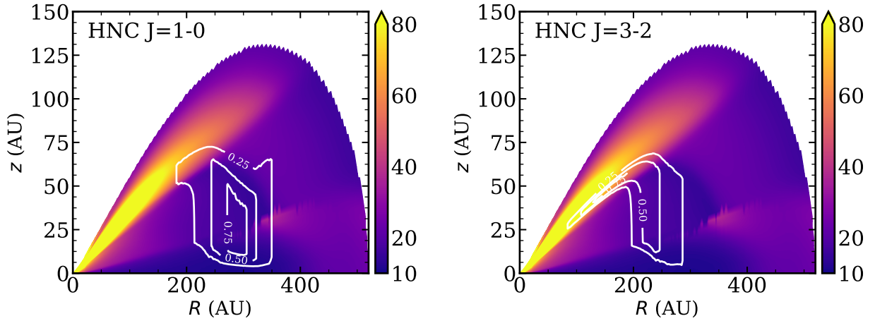
Fig. A.1. Contribution function distribution on top of the disk gas temperature distribution. White contours indicate the locations from which 25, 50, and 75% of the emission originates. HNC J = 1-0 mostly emits from the coldest disk region close to disk midplane, while HNC J = 3-2 largely comes from the warm finger tip.
