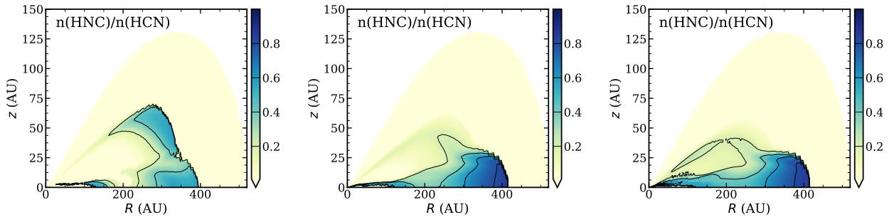
Fig. D.1. Similar plot as in Fig. 3, but for models including initial elemental depletion. From left to right: (1) C and O depleted by a factor of 10, (2) C and O depleted by a factor of 100, and (3) C depleted by a factor of 100, with O further depleted to reach C/O = 1.5 .
