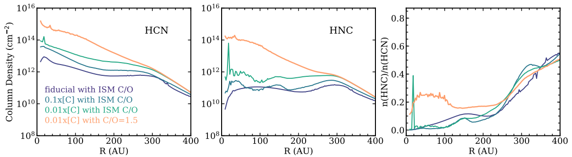
Fig. 8. Column density profiles of HCN and HNC, as well as their ratio profiles, for disk models with different levels of C and O initial abundances: the fiducial model with C/O = 0.3 close to the ISM level (in purple), C and O abundances reduced by a factor of 10 (in blue) and 100 (in cyan) from fiducial values, thus with the same ISM C/O , and the C abundance reduced by a factor of 100 from fiducial values with enhanced O depletion to reach a high C/O = 1.5 (in orange).
