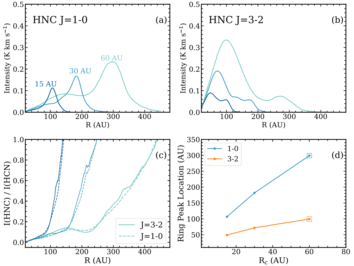
Fig. B.1. Line emission patterns in models with different R_c values (disk sizes): (a) radial intensity profiles for HNC 1–0, (b) radial intensity profiles for HNC 3–2, (c) HNC-to-HCN intensity ratio profiles, and (d) emission peak location for both transitions. The fiducial model results are marked as open squares.
