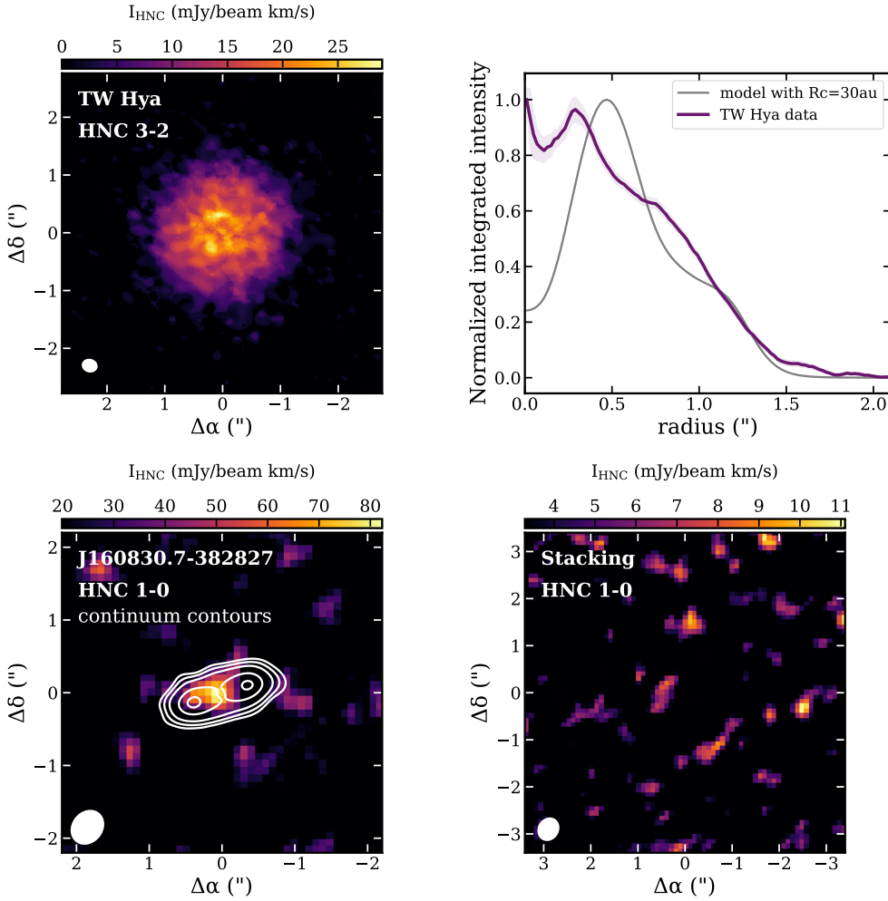
Fig. 9. Upper panels: HNC 3–2 emission for TW Hya from ALMA observations and the deprojected azimuthally averaged (normalized) radial intensity profile for HNC emission in TW Hya (purple line). A model profile convolved with the same beam size as the ALMA observations is also shown for comparison (gray line). Lower panels: moment-zero maps for the HNC 1–0 detection of J160830.7-382827 and stacking results for the remaining 28 disks in the Lupus sample from ALMA observations. White contours depict the continuum emission for the transition disk J160830.7-382827, where dust emission is absent in the disk center, while HNC 1–0 emission mostly originates within the dust hole. The beam sizes are shown in the left corner of each panel.
