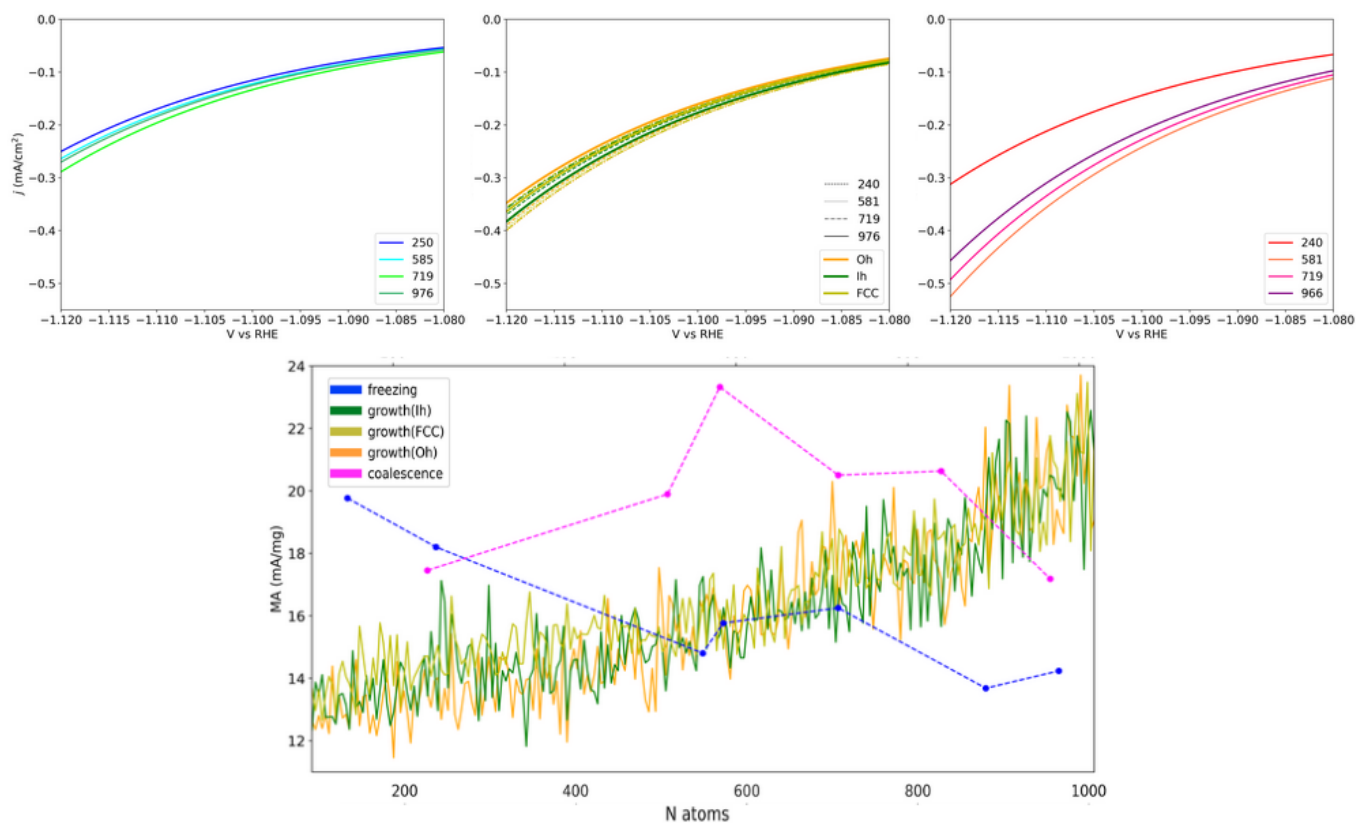
Fig. 6 Upper row displays the current densities for \text{CO}_2 \rightarrow \text{CH}_4 conversion around U=-1.1\text{V} vs RHE for Cu-NPs of different sizes. Left panel represents Cu-NPs from the annealing of a liquid droplet (top-left, blue), the middle panel from the atom-by-atom growth (top-centre, orange is for Oh seed, dark-green for Ih and olive for FCC initial seeds, respectively). Right panel reports coalesced Cu-NPs (top-right, pink). The bottom row shows the mass activity for \text{CH}_4 conversion at U=-1.1\text{V} vs RHE plotted versus the size of Cu-NPs sampled over the three formation processes (blue annealing; green-orange growth; magenta coalescence). Dashed lines for annealing and coalescence are a guide to an eye. Growth lines look continuous as data are available at each size. Those data points are filtered via a Gaussian Kernel for readability. The non-filtered data display oscillations within \pm 5\text{mA/mg} , due to the instantaneous appearance/disappearance of surface defects with aGCN values close to the structural relationship's maximum (Fig. 2).
