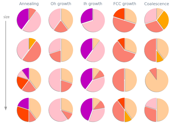
Fig. 3 The pie charts represents the statistical shape-distribution from 10 independent simulations. Each row corresponds to a certain size (from top to bottom: 240-250, 581-585, 719 and 966-976 atoms). The colours refers to the formation of icosahedra (Ih), defected Ih (dlh), FCC, defected FCC (dFCC, i.e. FCC with a twinning plane, light red), decahedra (Dh), defected (dDh). Such classification is done on the basis of CNA-signatures - such as (5,5,5), (4,2,1) and (4,2,2) - which enable to distinguish Ih, Dh, and FCC. A shape is classified into a certain family when more than the 70% matches the reference values.
