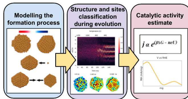
Fig. 1 Graphical representation of the multiscale numerical strategy adopted here. The modelling of the formation processes (annealing, growth, coalescence) is by means of molecular dynamics (MD) starting from a plethora of Cu-NPs of different shapes and sizes. We perform an accurate structural analysis of each trajectory and per each time-step the NP is classified into geometrical families and the type and the occurrence of each adsorption site is monitored following the time evolution of the atop generalised number. We then estimate the CH 4 mass activity for each Cu-NP during their formation process by the multiscale model of Ref. 40 .
