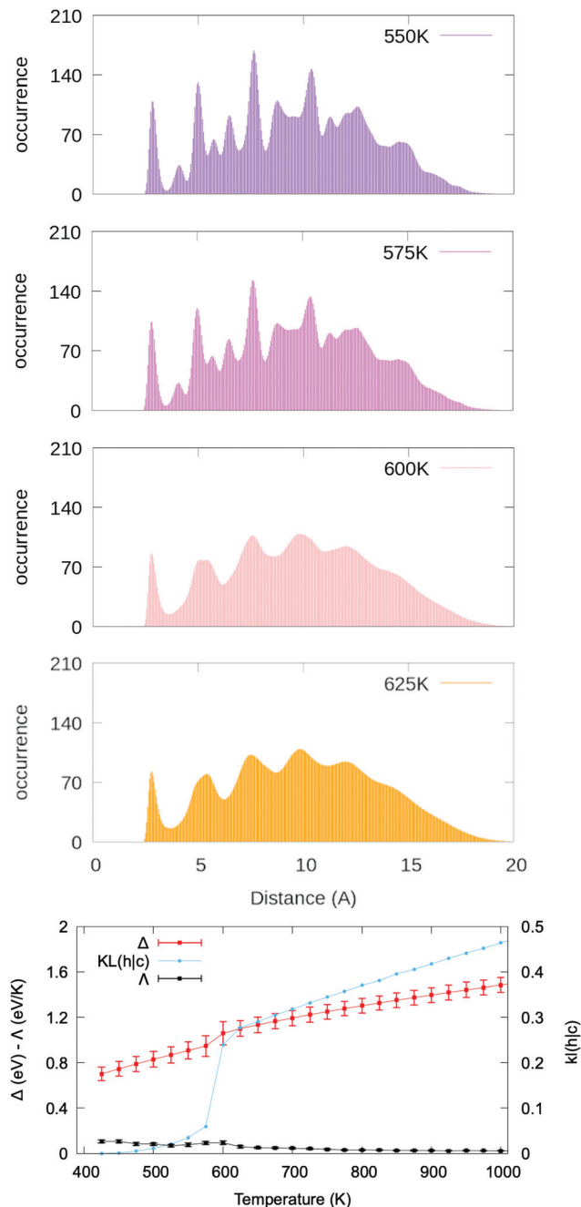
Fig. 5 The upper panels show the average PDDF for \text{Ag}_{201} (~1.8 nm) embedded in a strongly interacting environment ( p = 1.5 , \epsilon = 0.04 eV per atom) at different temperatures. Note the disappearance of the second peak of the PDDF for temperatures above 600 K. The lower panel shows caloric curve (red squares), heat capacity (black circles) and \text{KL}(\text{h|c}) temperature dependence (blue circles), lines act as a guide to the eye. A quasi-first order transition in the \text{KL}(\text{h|c}) curve at 625 K signals the nanoparticle melting, yet this is less evident from the caloric and heat capacity curves.
