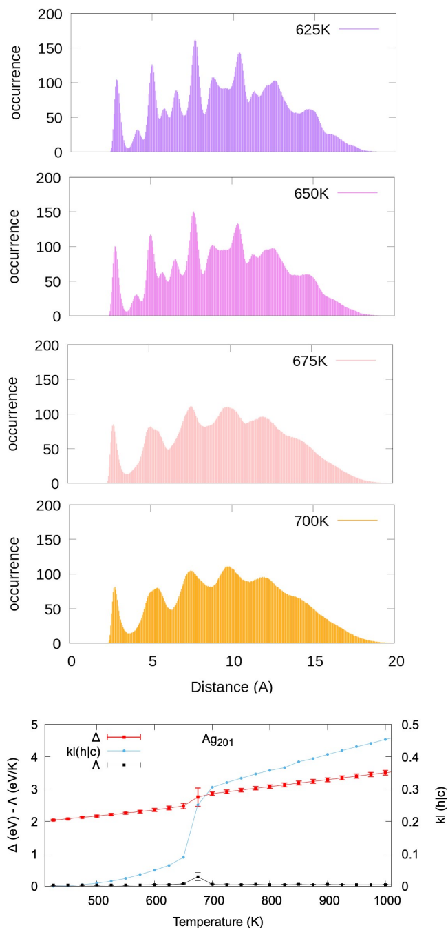
Fig. 2 The upper panels show the average PDDF for Ag 201 (~ 1.8 nm) taken at different temperatures. Above 675 K, the second peak has disappeared, whilst there is just a shoulder visible at ~4.08 Å at 675 K. The bottom panel reports the caloric curve (red squares), heat capacity (black circles) and KL(h|c) (blue circles) temperature dependence for a Ag nanoparticle of 201 atoms. Lines act as a guide to the eye. A quasi-first order transition occurs at 675 K.
