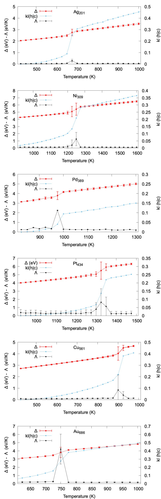
Fig. 3 Caloric curve (red squares), heat capacity (black circles) and KL(h|c) (blue circles) dependence with respect to temperature in an array of systems of different size, composition, and initial structure. Both \Delta and KL display a quasi-first order transition at the melting, whilst \Lambda displays a maximum.
