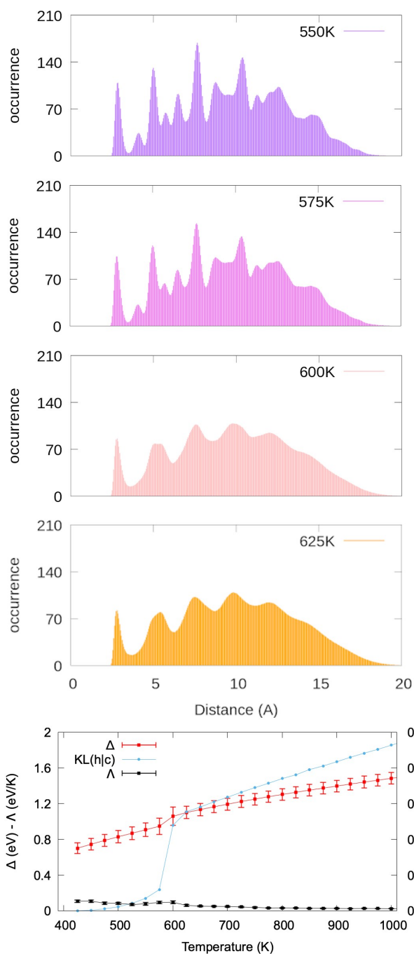
Fig. 5 The upper panels show the average PDDF for \text{Ag}_{201} ( \sim 1.8 nm) embedded in a strongly interacting environment ( p=1.5 , \epsilon=0.04\text{eV/atom} ) at different temperatures. Note the disappearance of the second peak of the PDDF for temperatures above 600 K. The lower panel shows caloric curve (red squares), heat capacity (black circles) and \text{KL}(h|c) temperature dependence (blue circles), lines act as a guide to the eye. A quasi-first order transition in the \text{KL}(h|c) curve at 625 K signals the nanoparticle melting, yet this is less evident from the caloric and heat capacity curves.
