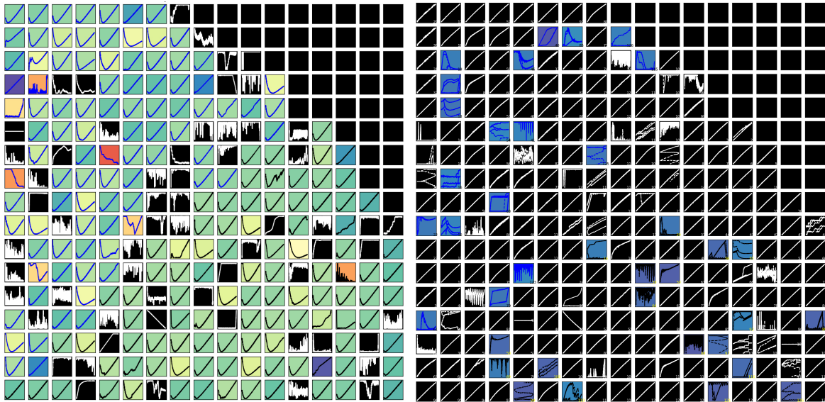
Figure 9. Left : I-V curves of the QUBIC P87 TES array measured in the blind configuration at 348mK down to about 60% of the normal resistance. The color code indicate the turn-over bias voltage. Right : same array measured in open configuration at 382mK. (Color figure available online)
