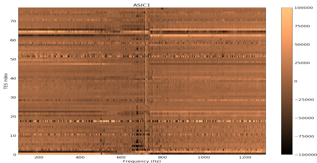
Figure 17. timelines in ADU of some TES as a function of the frequency of excitation.(colorfull graph available online)
