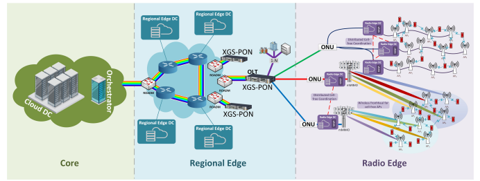
Fig. 1. Main concept of MARSAL project describing a complete 5GB system set-up from access to the core networks
