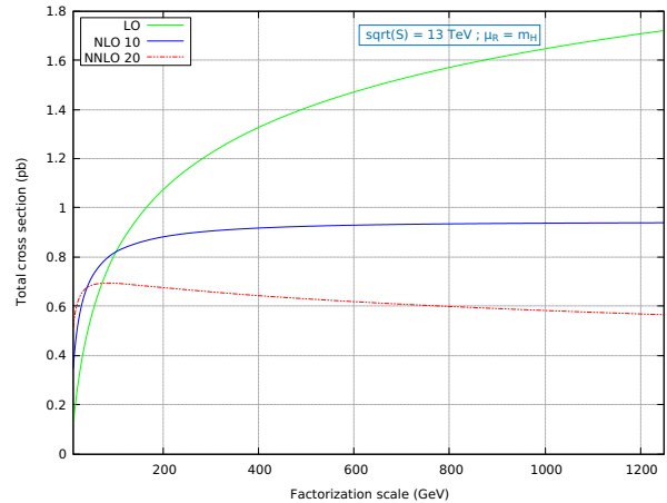
FIG. 6: The factorization scale variation of the total cross section at various perturbative orders in QCD.
