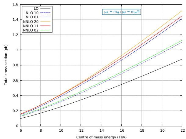
FIG. 4: The total cross section at various perturbative orders at energy scales varying from 6 to 22 TeV at LHC.
