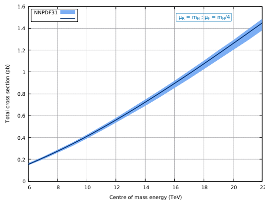
FIG. 7: PDF uncertainties.
