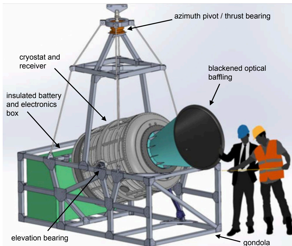
Figure 11. LSPE-SWIPE overview. The instrument is contained in a large liquid Helium cryostat, which also contains the optical elements, including the HWP based Stokes polarimeter. The on-board electronics and the Lithium batteries based power system are contained in an Aerogel insulated box, to optimize thermal balance.
