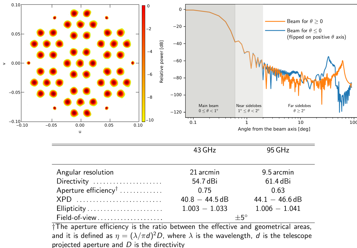
Figure 5. Left: footprint of the LSPE-Strip main beams in the (u, v) plane (large beams, 43 GHz, small beams, 95 GHz). Right: beam cut for \phi = 0 of the central horn. We have flipped the beam section for \theta < 0 on the positive axis to better highlight the asymmetries. The (u, v) variables are defined as u = \sin(\theta) \cos(\phi) , v = \sin(\theta) \sin(\phi) , where (\theta, \phi) are standard spherical coordinates, with the center of the telescope pointing towards \theta = 0 . The inset table reports the averaged main optical parameters.
