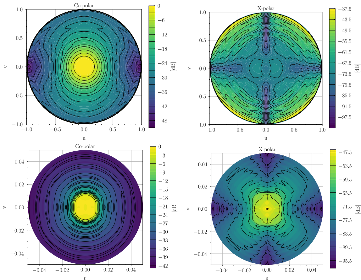
Figure 14. panels: simulated beam response of the SWIPE multi-moded horns. Radiation is propagated into the far field with linear polarization parallel to the v axis in the plane of the horn aperture, corresponding to the \phi = 90^\circ axis in the far field. Bottom panels: simple physical optics simulation of the SWIPE telescope main beam, for a pixel at the center of the focal plane. The simulation includes the feed pattern shown above, the aperture stop and the HDPE lens. A perfectly absorbing tube and no further obstructions apart from the cold aperture stop have been assumed. Co-polar and cross-polar patterns have been calculated according to Ludwig’s third definition in [78] and are mapped as a function of u = \sin(\theta) \cos(\phi) and v = \sin(\theta) \sin(\phi) , where (\theta, \phi) are the standard spherical coordinates, and the telescope bore-sight is pointing at \theta = 0 . Contours are shown every 3 dB for the co-polar patterns and every 6 dB for the cross-polar patterns.
