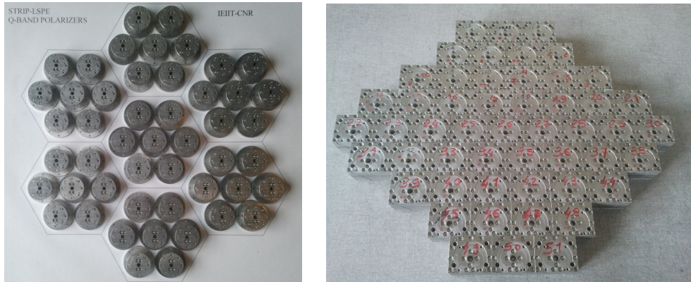
Figure 8. Left: the 49 Strip Q-band polarizers arranged according the 7-module feedhorn footprint. Right: the 49 Strip Q-band platelet OMTs.
