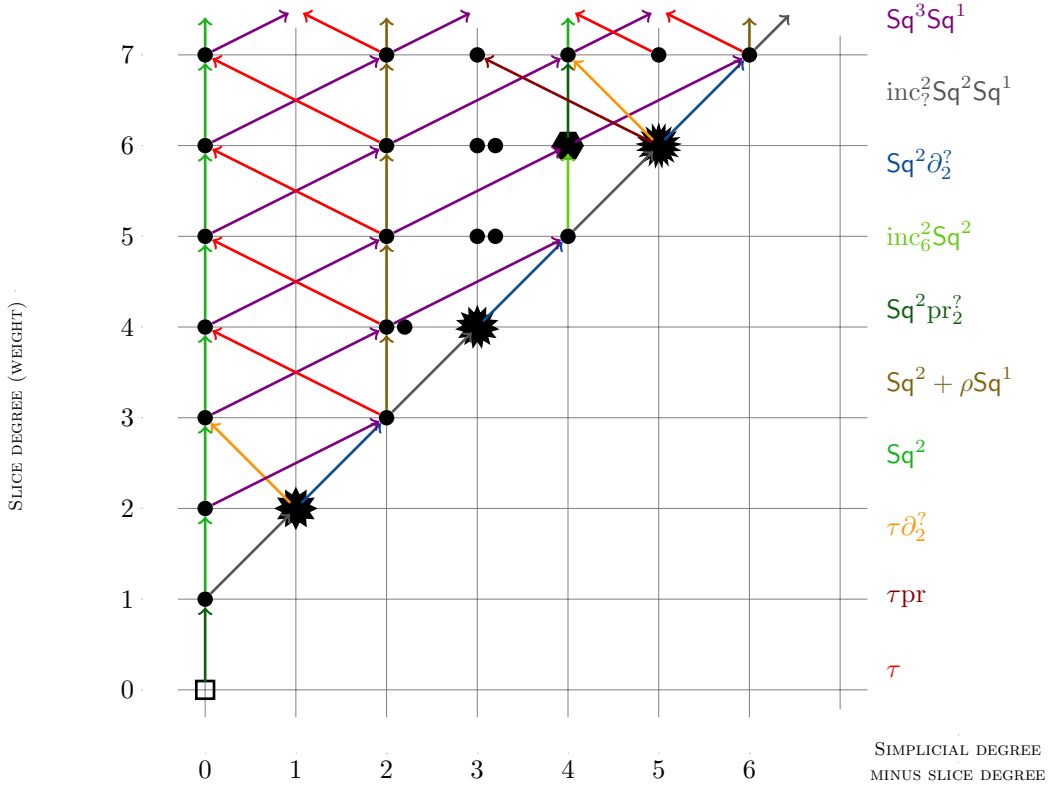
Figure 4.1: The first slice differential for \mathbf{1}_\Lambda .
