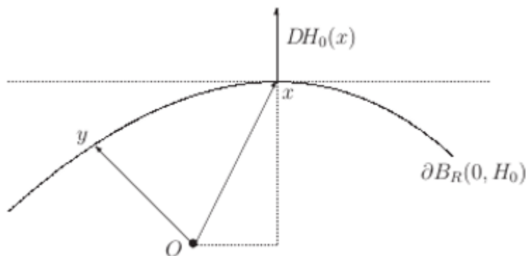
FIGURE 1. Maximizing the scalar product y \cdot DH_0(x) under the constraint H_0(y) = R
