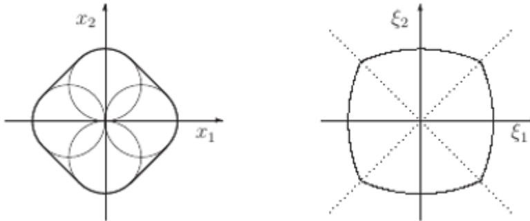
FIGURE 2. The ball B_1(0, H_0) (left) is smooth, its dual (right) is not.
