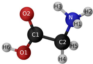
Figure 5. Protonated Glycine (GlyH + ) lowest energy conformer at DFT-B3LYP/aug-cc-pVDZ level of theory.
