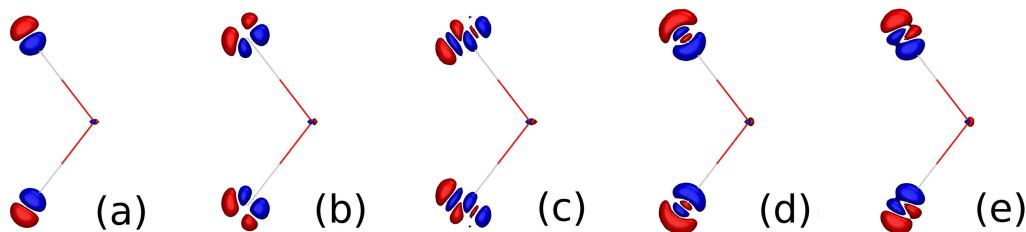
Figure 2. Differences of the anharmonic one-nucleus density with the corresponding harmonic one. State (000) in panel (a), (010) in (b), (020) in (c), (100) in (d), and (001) in (e). Red indicates positive contributions, where the molecular density concentrates due to anharmonicity, while blue stands for the negative contributions, where the density is depleted due to anharmonicity. The isodensity surfaces are set to +5 and -5 a.u..
