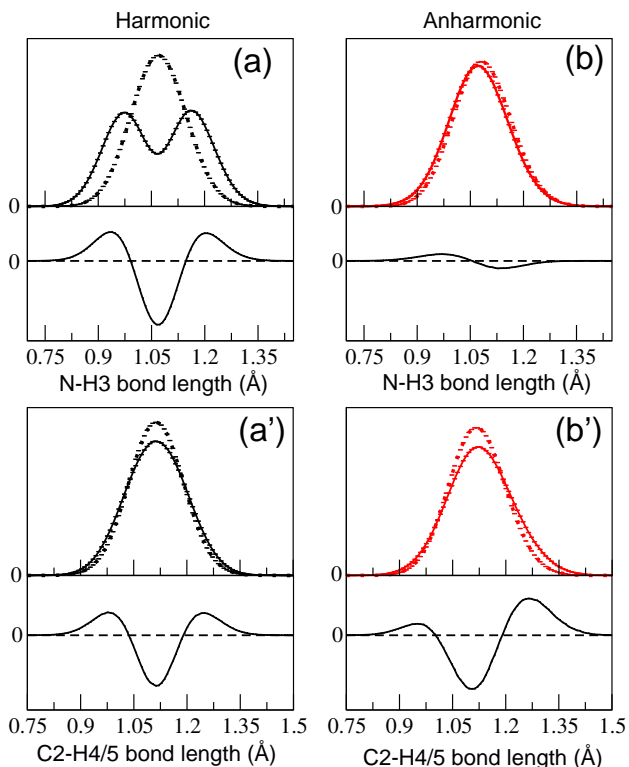
Figure 10. The \nu_{23} = 1 excited state (continuous lines) and the ground state (dotted lines) bond-length distributions. Panels (a) and (a') in harmonic approximation along the N-H3 and C2-H4/5 stretch directions respectively. Panels (b) and (b') show the anharmonic case. The ground state densities are presented in our previous work. [38] The lower parts of the plots show the difference of the curves reported in the upper parts.
