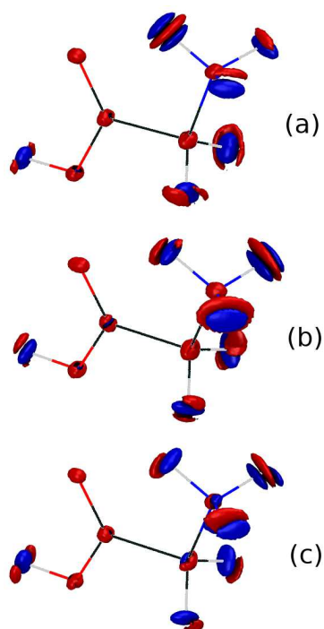
Figure 7. One-nucleus density differences between the anharmonic and the corresponding harmonic marginal one-nucleus density for the (a) \nu_{23} = 1 , (b) \nu_{25} = 1 , and (c) \nu_{26} = 1 vibrational excited states. Red indicates positive contributions, where the density concentrates due to anharmonicity, while blue stands for the negative contributions, where the density is depleted due to anharmonicity. The isodensity surfaces are respectively set to +0.15 and -0.15 a.u..
