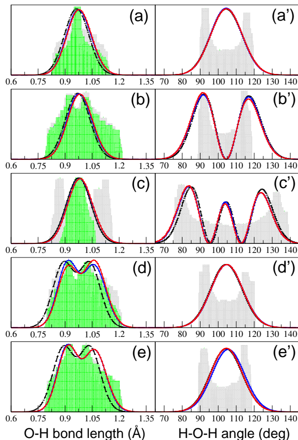
Figure 3. Water bonds and H-O-H angle probability density distributions obtained from quantum harmonic (black dashed line), DVR [39] (blue line), and semiclassical (red line) wavefunctions. Left panels (a), (b), (c), (d), and (e) are respectively for the radial O-H distribution of the ground (000), (010), (020), (100) and (001) vibrational eigenfunctions. Right panels (a'), (b'), (c'), (d'), and (e') are for the angular H-O-H distributions of the same ordered vibrational states. The filled-area plots on the background represent the classical distributions obtained from the classical trajectory used to generate each wavefunction with our semiclassical approach. In the left panels, gray and green histograms stand for the two bond-length distributions along each water O-H bond and, in the right panels, gray histograms are for the H-O-H angle.
