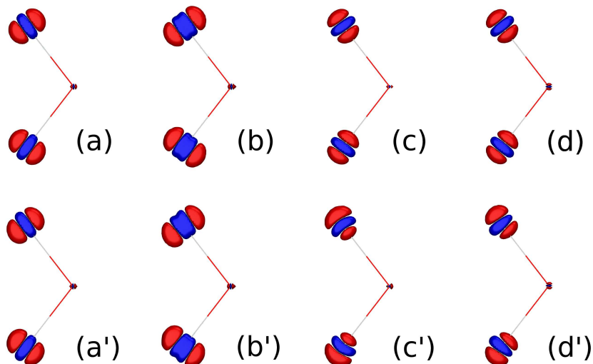
Figure 4. Harmonic (top panels (a), (b), (c), and (d)) and semiclassical anharmonic (lower panels (a'), (b'), (c'), and (d')) nuclear density differences obtained by subtracting the zero point energy (000) state one-nucleus density to respectively the (010), (020), (100) and (001) excited state densities. Red indicates positive contributions, where the density concentrates due to the excitation, while blue stands for the negative contributions, where the density is depleted due to the excitation. The isodensity surfaces are set to +5 and -5 a.u..
