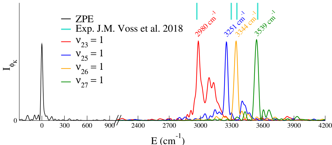
Figure 6. GlyH + MC-SCIVR power spectrum. Each peak is obtained from a trajectory with energy equal to the fundamental mode 23, 25, 26, and 27 using the initial conditions of Eq. 12 and the relative harmonic reference state.[46] The peak positions are shown relative to the ZPE one, and the peak heights have been arbitrarily scaled, since we are interested on peak positions only, i.e. E_n in Eq. 14. The ZPE and \nu_{27} peaks are taken from our previous study.[38] Vertical lines are the peak positions from the experimental IR spectrum Voss, Fischer, and Garand [12].
