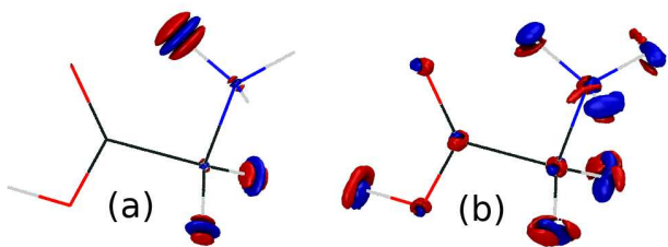
Figure 9. GlyH + one-nucleus density difference plots for \nu_{23} = 1 vibrational eigenstate. Panel (a) depicts the difference between excited and ground harmonic densities, while panel (b) shows the anharmonic case. Red indicates positive contributions, while blue stands for the negative contributions. All isodensities are set to +0.1 and -0.1 a.u..
