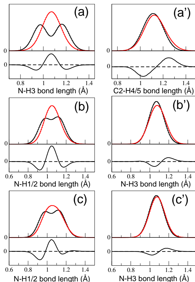
Figure 8. Bond-length distributions comparison between harmonic (black lines) and anharmonic (red lines) states for excitation \nu_{23} = 1 along the N-H3 and C2-H4/5 stretching (panels (a) and (a')), \nu_{25} = 1 along N-H1/2 and N-H3 ones (panels (b) and (b')), and \nu_{26} = 1 along N-H1/2 and N-H3 directions (panels (c) and (c')). The lower part of each plot shows the difference of the two curves reported in the upper part by subtracting the harmonic distribution from the anharmonic one.
