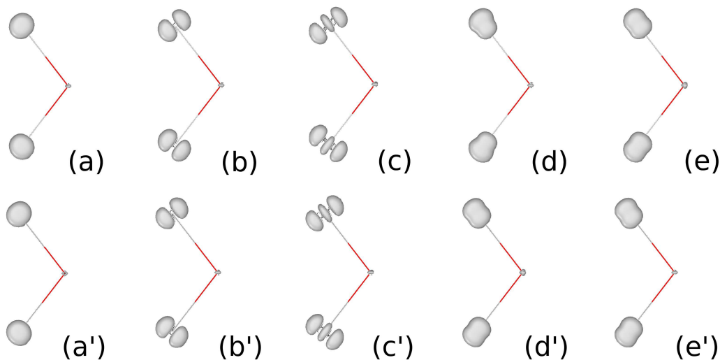
Figure 1. Water molecule one-nucleus densities. Anharmonic vibrational state eigenfunction (000) in panel (a), (010) in panel (b), (020) in panel (c), (100) in panel (d), and (001) in panel (e). Harmonic vibrational eigenfunction (000) in panel (a'), (010) in panel (b'), (020) in panel (c'), (100) in panel (d'), and (001) in panel (e'). All isodensity surfaces are set to 10 a.u..
