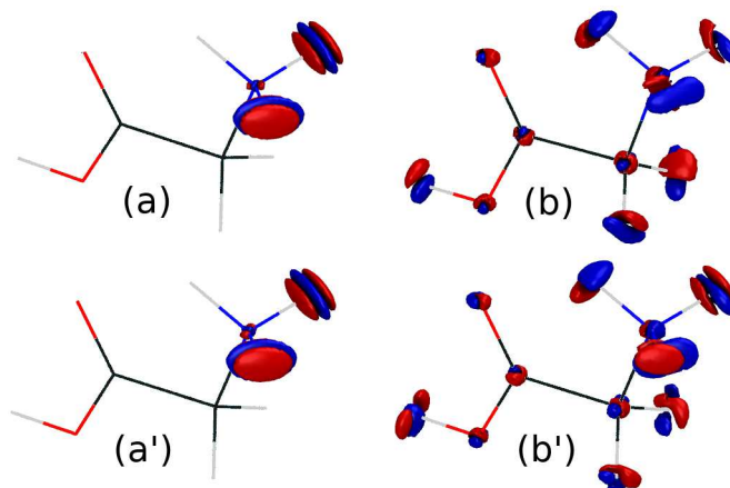
Figure 11. One-nucleus density difference plots for the GlyH + \nu_{25} = 1 (panels (a) and (b)) and \nu_{26} = 1 (panels (a') and (b')) vibrational eigenstates. Panels (a) and (a') depict the difference of the harmonic excited state and ground state densities, while panels (b) and (b') refer to the anharmonic case. Red indicates positive contributions, while blue stands for the negative contributions. All isodensities are set to 0.1 and -0.1 a.u..
