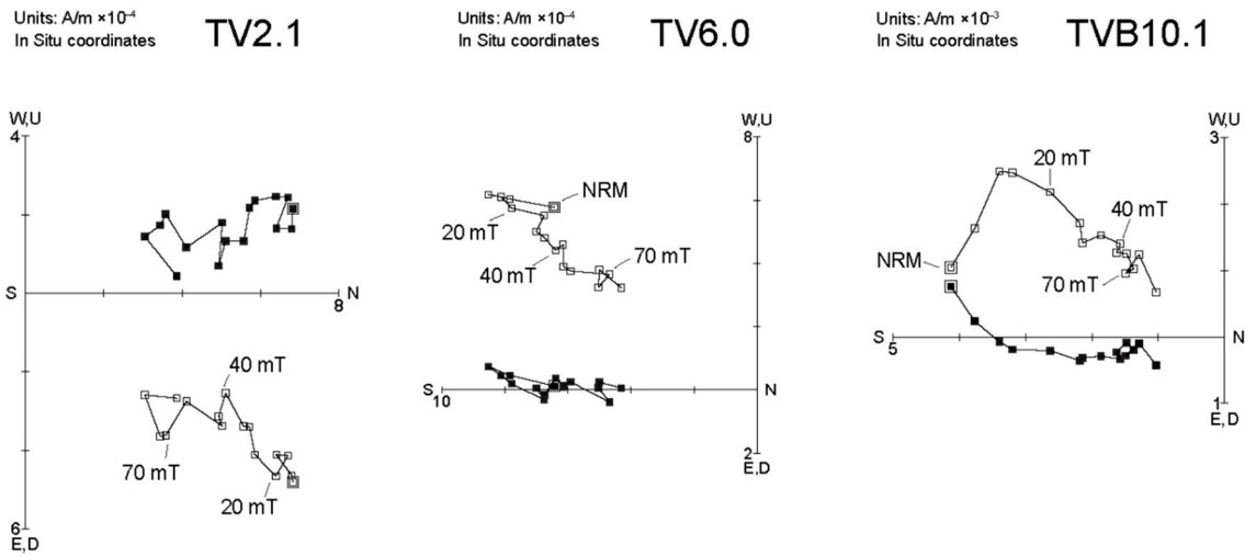
Figure 6. Vector end-point demagnetization diagrams of key samples from the Tsiotra Vryssi section in in situ coordinates. Closed squares are projections onto the horizontal plane, and open squares are projections onto the vertical plane. Applied AF covers a range 0–100 mT with steps of 5 mT up to 50 mT and of 10 mT up to 100 mT.
