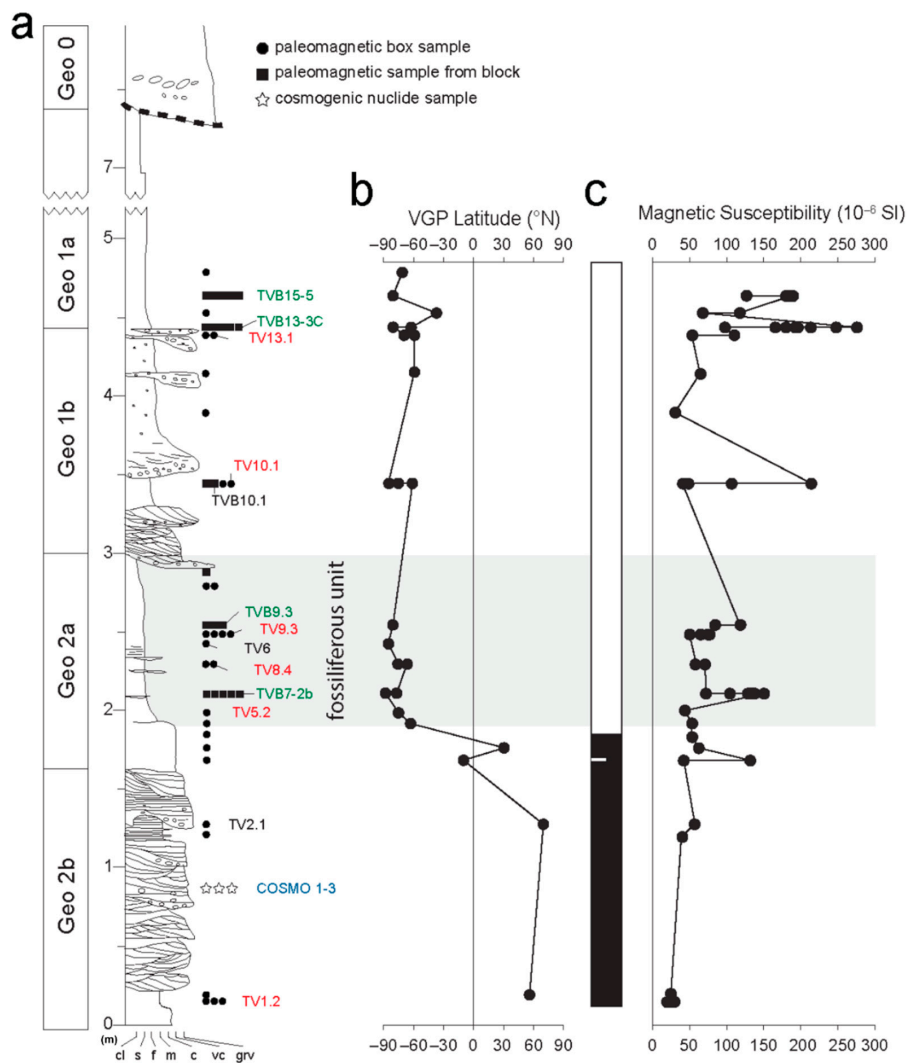
Figure 4. (a) Stratigraphic log (modified from [33]) of the Tsiotra Vryssi section with location of the samples for magnetostratigraphy and experiments for rock magnetism, and for cosmogenic radionuclides dating; (b) Latitude of the virtual geomagnetic poles (VGP) with interpreted magnetostratigraphy (black is normal polarity, white reverse polarity); (c) Magnetic susceptibility \kappa .
