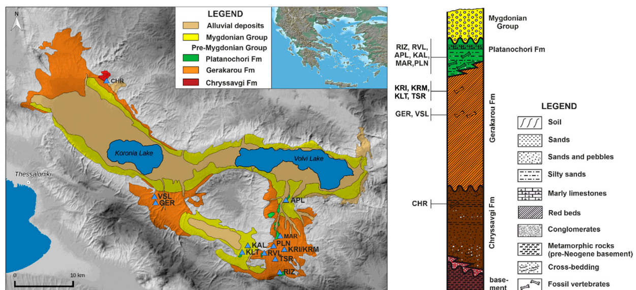
Figure 2. Geological map of the Neogene and Quaternary lithostratigraphic units of the Mygdonia Basin (left) and simplified composite stratigraphic column of the basin indicating the position of the fossiliferous localities (right). Modified from [21] and data from [19]. Map of Greece from Copernicus Land Monitoring Service ( https://land.copernicus.eu/ ).
