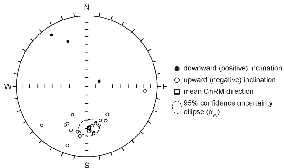
Figure 7. Equal-area projections of the ChRM component directions from the Tsiotra Vryssi section (see Table 3 for mean direction).
