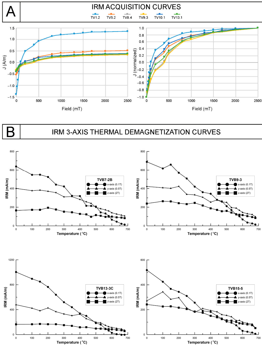
Figure 5. (A) Isothermal remanent magnetization (IRM) backfield acquisition curves and (B) thermal decay curves of three-axis IRM of selected samples from Tsiotra Vryssi (see Figure 4 for location).
