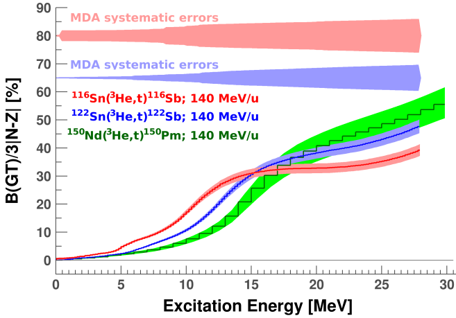
Figure 16. Full integral of the B(GT) spectra as a function of the excitation energy up to where the integral was truncated. The data on ^{150}\text{Nd}(^3\text{He}, t)^{150}\text{Pm} were obtained from Guess et al. [23]. The other data were obtained from figs. 11 and 12. Systematic errors from the MDA fitting procedure were not included in the ^{116,122}\text{Sn}(^3\text{He}, t)^{116,122}\text{Sb} error bands, but shown as separate bands instead. For ^{150}\text{Nd}(^3\text{He}, t)^{150}\text{Pm} , these systematic errors are included in the error band.
