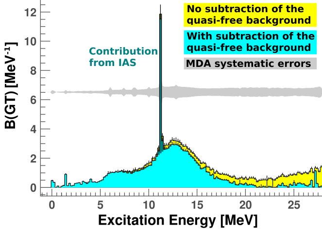
Figure 12. Same as fig. 11, but now for the ^{122}\text{Sn}(^3\text{He}, t)^{122}\text{Sb} reaction.
