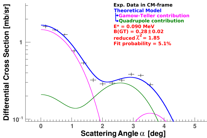
Figure 9. Angular distribution of the differential cross section of the state labelled 1 in fig. 7. The MDA used to extract the corresponding B(GT) value was also shown.
