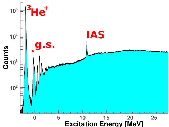
Figure 4. Same as fig. 3, but for the ^{122}\text{Sn}(^3\text{He}, t)^{122}\text{Sb} reaction.
