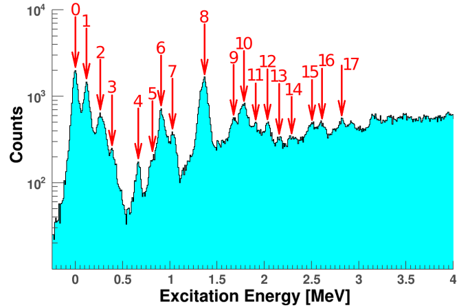
Figure 8. Same as fig. 7, but now for the ^{122}\text{Sn}(^3\text{He}, t)^{122}\text{Sb} reaction.
