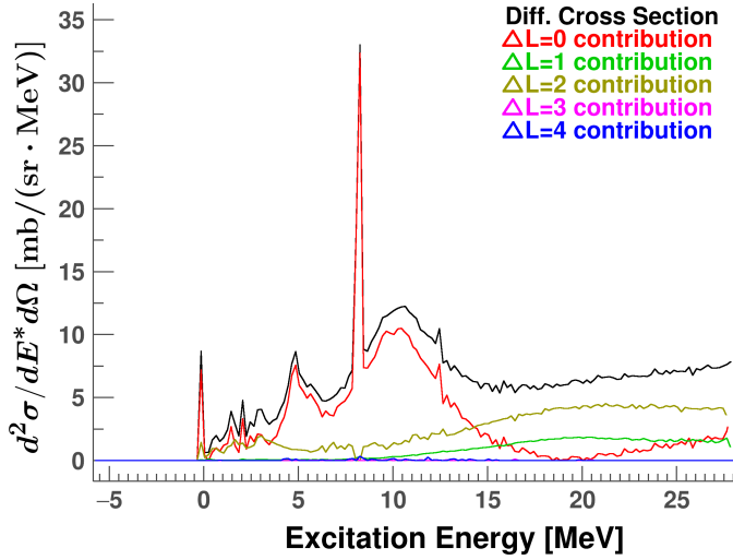
Figure 13. Different multipolarity contributions to the differential cross section for the ^{116}\text{Sn}(^3\text{He}, t)^{116}\text{Sb} reaction at 140 MeV/u without subtraction of the quasi-free background. The \Delta L = 3 and \Delta L = 4 contributions are relatively small.
