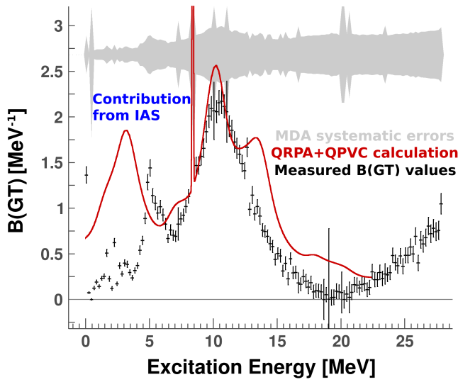
Figure 18. Comparison between experimental data (measured with (^3\text{He}, t) at 140 MeV/u) and QRPA+QPVC calculations for the Gamow-Teller strength distribution of ^{116}\text{Sb} in the situation where the quasi-free background was not subtracted. Note that higher B(\text{GT}) ‘ \Delta L = 0 ’ strength could possibly be due to the low-energy tail of the IV(S)GMR ( 2\hbar\omega ), which was not included in the calculations.
