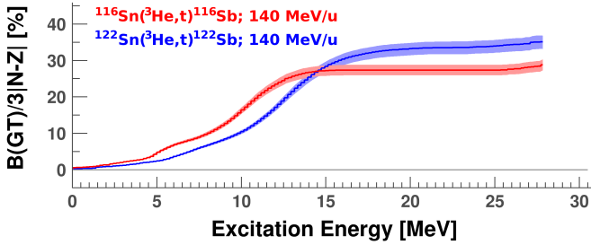
Figure 17. Same as fig. 16, except now the quasi-free background was subtracted (with N_0 being maximal). The ^{150}\text{Nd}(^3\text{He}, t)^{150}\text{Pm} results are not shown for this situation, since those data were not available in ref. [23]. Systematic errors are approximately the same as in fig. 16.
