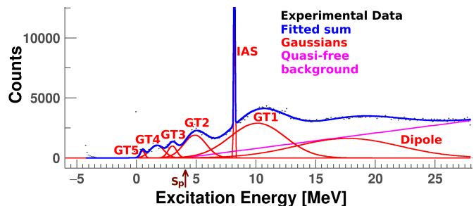
Figure 15. Illustration of the fitting procedure used by Pham et al. [21], applied to the present ^{116}\text{Sn} data and subjected to the condition 0^\circ \leq \theta \leq 1.3^\circ .
