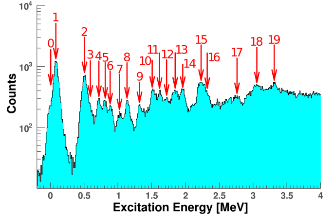
Figure 7. States that could be resolved in the low-energy region of the excitation-energy spectrum for the ^{116}\text{Sn}(^3\text{He}, t)^{116}\text{Sb} reaction.
