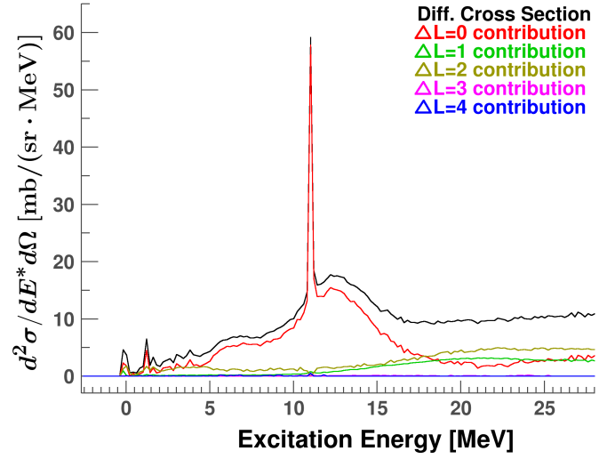
Figure 14. Same as fig. 13, but now for the ^{122}\text{Sn}(^3\text{He}, t)^{122}\text{Sb} reaction at 140 MeV/u.
