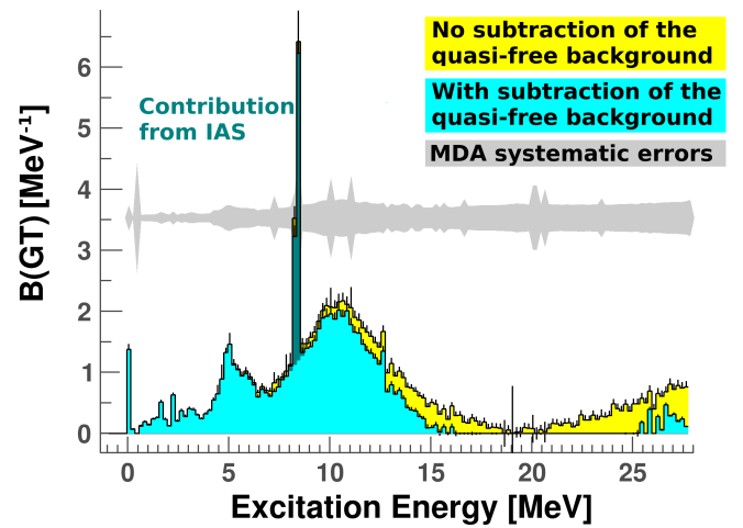
Figure 11. B(GT) spectrum for the ^{116}\text{Sn}(^3\text{He}, t)^{116}\text{Sb} reaction at 140 MeV/u. Both the situation where the quasi-free background is not subtracted and the situation where the upper bound of the quasi-free background is subtracted are shown. Note that if the subtraction leads to negative B(GT) values, they are set to zero in the figure.
