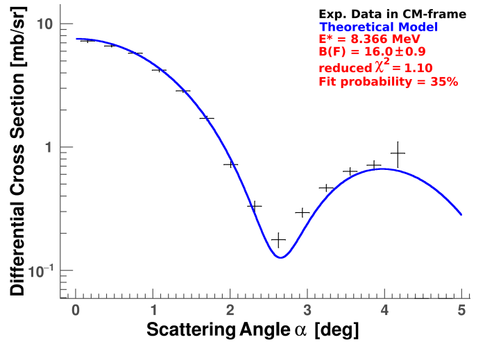
Figure 5. Extracted differential cross section of the IAS for the ^{116}\text{Sn}(^3\text{He}, t)^{116}\text{Sb} reaction at 140 MeV/u. The theoretical model is computed with FOLD as described in the text, and fitted to the data with the overall normalisation as the only variable parameter. The fit probability is the area under the reduced \chi^2 distribution to the right of the reduced \chi^2 value of the fit.
