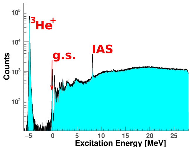
Figure 3. Measured excitation-energy spectrum for the ^{116}\text{Sn}(^3\text{He}, t)^{116}\text{Sb} reaction in the range 0^\circ \leq \theta \leq 4.2^\circ at 140 MeV/u, obtained after a sieve-slit calibration.
