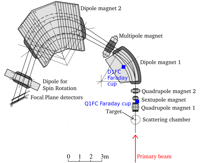
Figure 1. Schematic overview of the Grand Raiden Spectrometer; based on [24].
