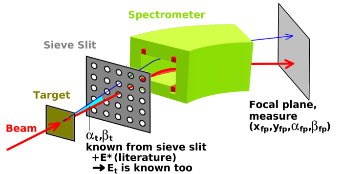
Figure 2. Illustration of the sieve-slit measurement used to calibrate the excitation energy and the horizontal and vertical scattering angles at the target.
