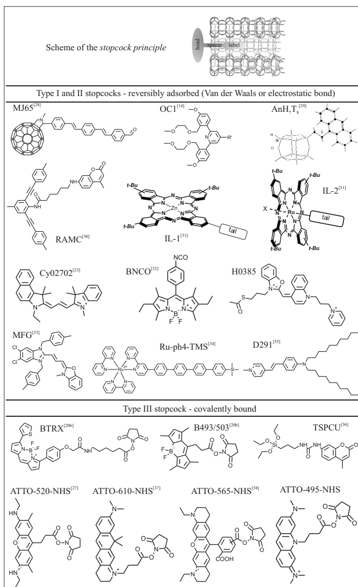
Fig. 4. Stopcock molecules
