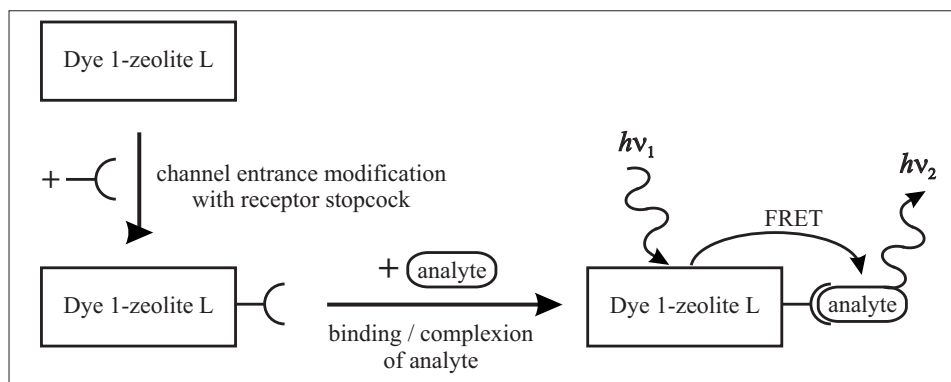
Scheme. Working principle of a functional energy transfer label. In a first step, the channel entrances of zeolite L crystals, loaded with Dye 1, are modified with a receptor stopcock. [27,41] The resulting material can now bind to a compatible analyte, so that the distance between Dye 1 and the analyte is short enough for energy transfer to occur.
