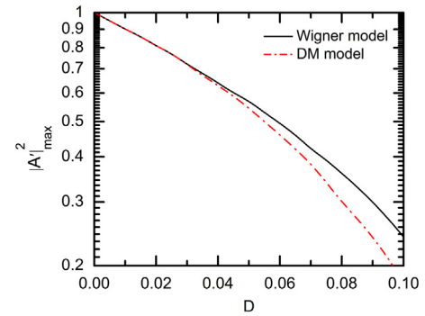
Fig. 5. Comparison between the maximum peak |A|^2 as predicted by the density matrix (DM) and Wigner models where |A|^2 is plotted against D .
