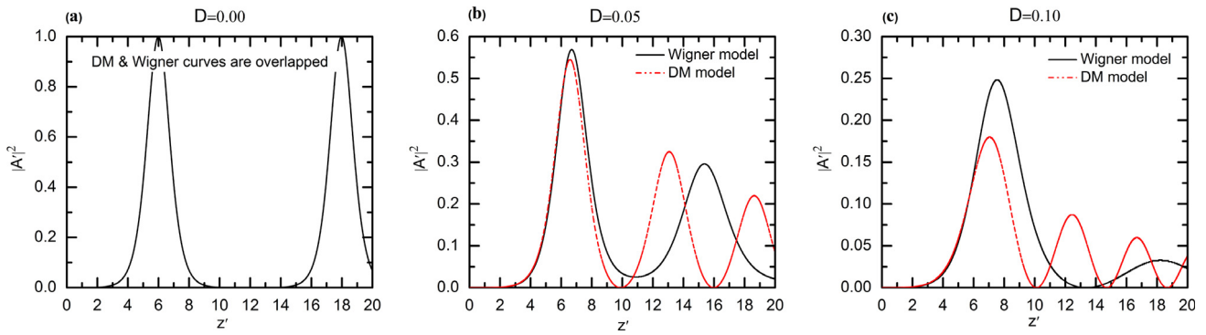
Fig. 3. For the density matrix (DM) and Wigner models, scaled intensity |A|^2 is plotted as a function of z in the quantum regime for different values of the spontaneous emission rate (a) D = 0.0 (b) D = 0.05 (c) D = 0.1 .
