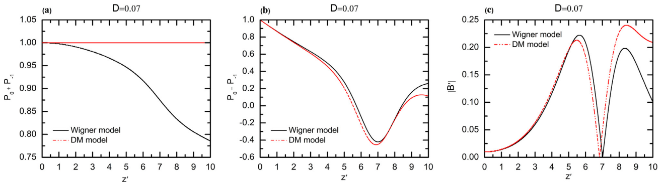
Fig. 4. For the density matrix (DM) and Wigner models when D = 0.05 , (a) The trace of probabilities P_0 + P_{-1} vs. z . (b) The population difference P_0 - P_{-1} vs. z . (c) The bunching factor B vs. z .
