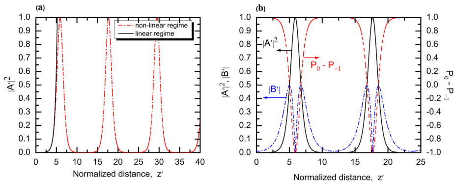
Fig. 2. (a) |A|^2 vs. z in the linear and nonlinear regimes. (b) |A|^2 , |B| , and P_0 - P_{-1} vs. z .
