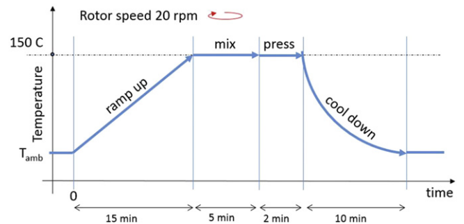
Fig. 2. Graphical view of the duration of the different phases of the scaffold fabrication process by referring to the different ranges of temperature.
