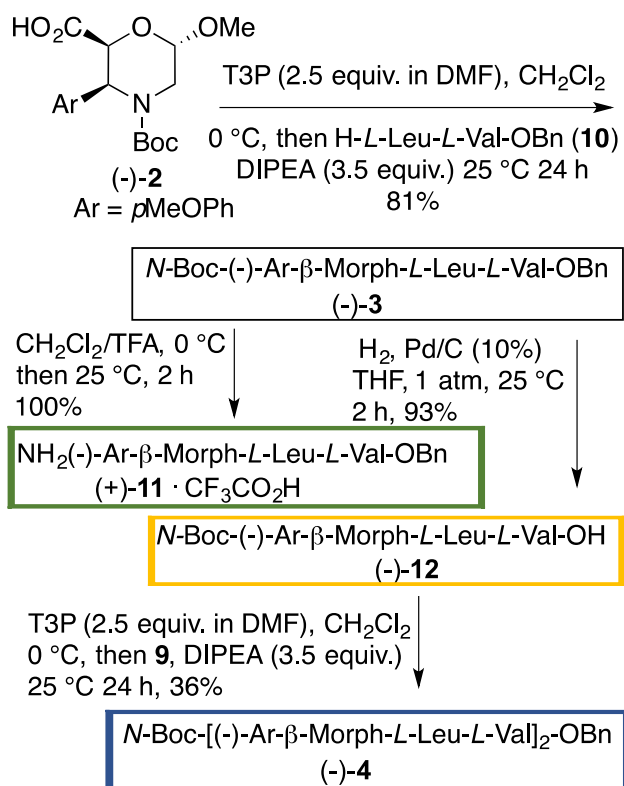
Scheme 2. Synthesis of tripeptide and (-)- 3 and hexapeptide (-)- 4
