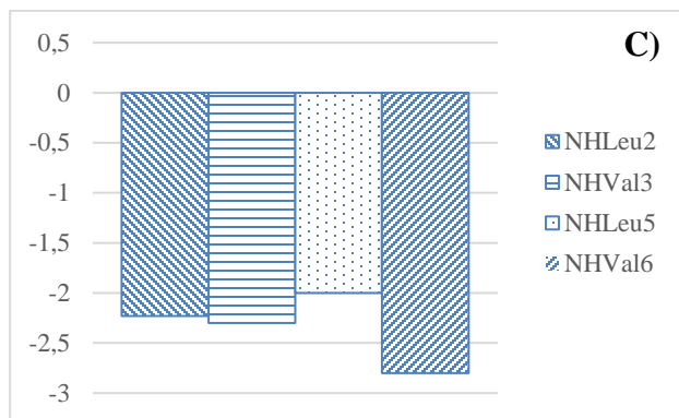
Figure 3. NMR data for hexapeptide (-)- 4 ( \text{CD}_3\text{CN} , mM, 600 MHz): A) NOEs of morpholino ring protons (blue arrows) and between the different AAs (red arrows) and H-bonds (dotted lines). B) Zoom of Val 3 /Morph 4 region. C) \Delta\delta/\Delta T NH values (273-333 K).
