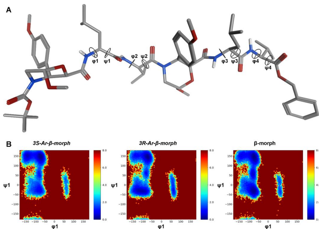
Figure 2. A) Representative geometry of the most populated cluster c0 for (3 S )-4. B) Heatmaps describing the relative free energy (kcal/mol) associated to different values for the \phi_1/\psi_1 dihedral pair for peptides (3 S )-4, (3 R )-4 and 5 , 24 containing 3 S -Ar- \beta -Morph, 3 R -Ar- \beta -Morph and \beta -Morph, respectively. The geometrical analysis was conducted on the 1000-1500 ns section of the unbiased H-REMD replica. Heatmaps for all the considered dihedral pairs are reported in Figure S1.
