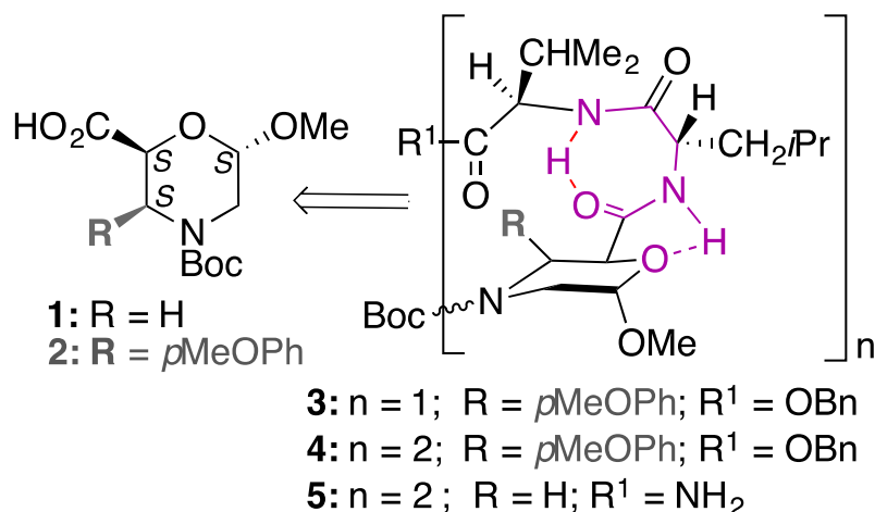
Figure 1. \beta -Morpholino containing peptides.
