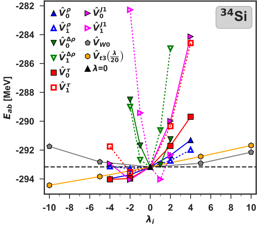
Figure 3. Perturbed ab initio energies compared with the unperturbed energy in ^{34}\text{Si} . Symbols shown in the legend correspond to different generators \hat{V}_i^{\text{gen}} . The full triangle represents the unperturbed energy at \lambda_i = 0 and the dashed line shows the reference value of E^{\text{ab}}(0) .
