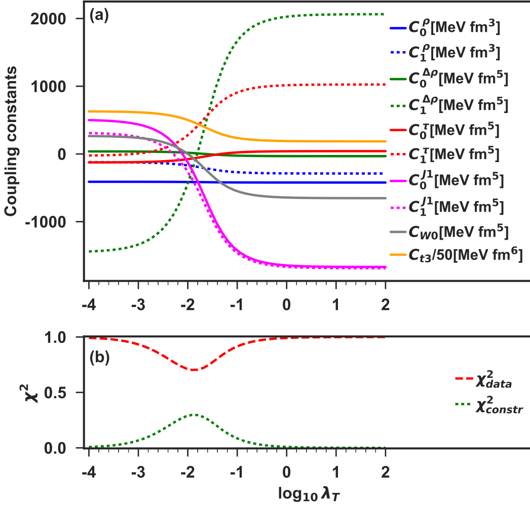
Figure 6. (a) Results obtained for the D_{\text{H-F}}(10) coupling constants with m^*/m constrained to 0.70 using the Tikhonov regularisation. (b) Contributions of the data, \chi_{\text{data}}^2 , and constraint, \chi_{\text{constr}}^2 , to the total penalty function \chi_T^2 (37).
