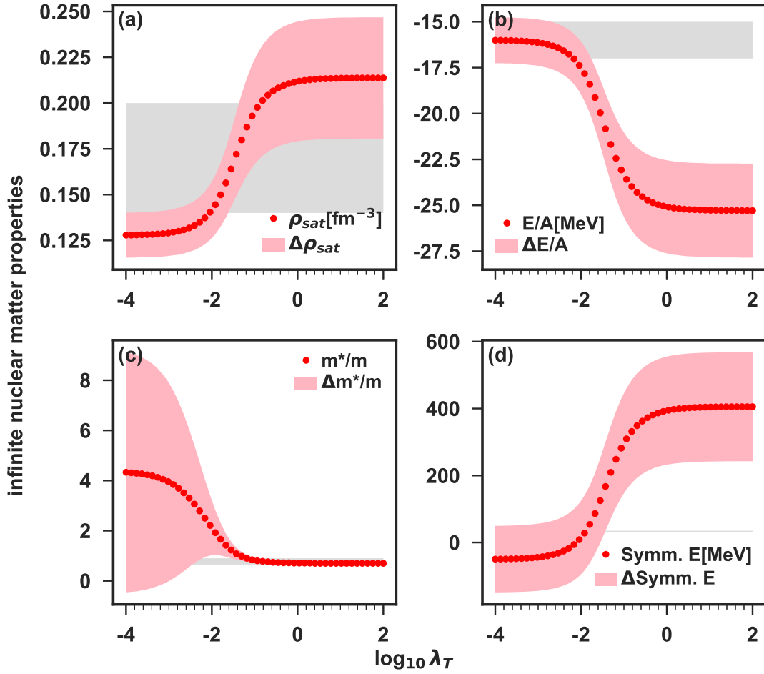
Figure 7. Infinite nuclear matter properties: \rho_{\text{sat}} (a), E/A (b), m^*/m (c), and symmetry energy J (d). obtained by the Tikhonov regularisation of the D_{\text{H-F}}(10) coupling constants with m^*/m constrained to 0.70. Shadows show the propagated error bars and grey regions indicate the ranges of empirical values.
