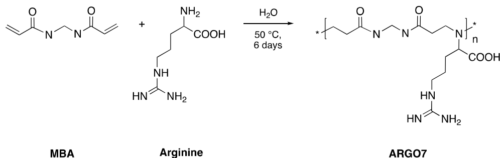
Scheme 1. Synthesis of ARG07.
