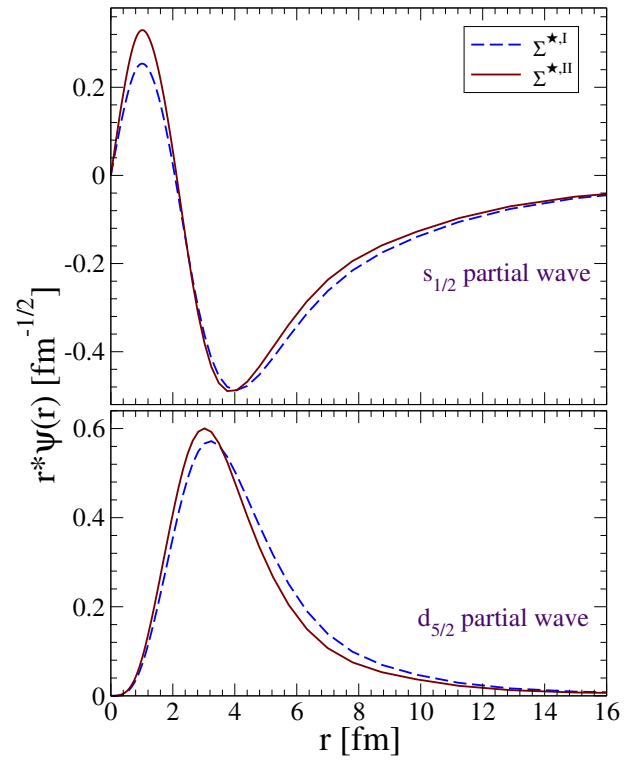
FIG. 6: Radial part of the overlap wave functions between ^{16}\text{O} and the bound d_{5/2} and s_{1/2} states of ^{17}\text{F} .
