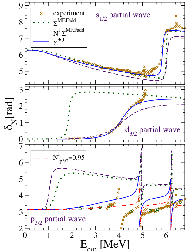
FIG. 3: Phase shifts obtained from the self consistent self-energy of Ref. [14] [Eq. 1] before (dotted lines) and after (dashed lines) correcting the depth of \Sigma^{MF,Fadd} to reproduce the quasiparticle (and quasihole) energies. The full lines are obtained when also the momentum components outside the model space \mathcal{P} are included, Eq. (3a). The s_{1/2} , d_{3/2} and p_{3/2} partial waves are shown. For p_{3/2} , the dot-dashed line was obtained by fitting N_{p_{3/2}}^I to reproduce the background phase shifts rather than the quasihole energy. The values of the corrections N_{lj}^I are reported in Tab. I. The experimental results are from Refs. [31] (crosses) and [32] (circles).
