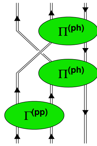
FIG. 2: Example of a diagrammatic contribution included in the Faddeev expansion for R^{(2p1h)} (see Fig. 1). A quasiparticle is coupled to the response function \Pi^{(ph)} that describes the target nucleus. It can also participate in a pairing processes, which is accounted by the two-body propagator g^{II,(pp)} .
