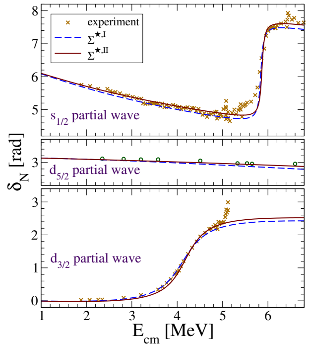
FIG. 4: Phase shifts for positive parity waves obtained from the the self-energies I (dashed lines) and II (full lines). The experimental results are from Refs. [31] (crosses) and [32] (circles).
