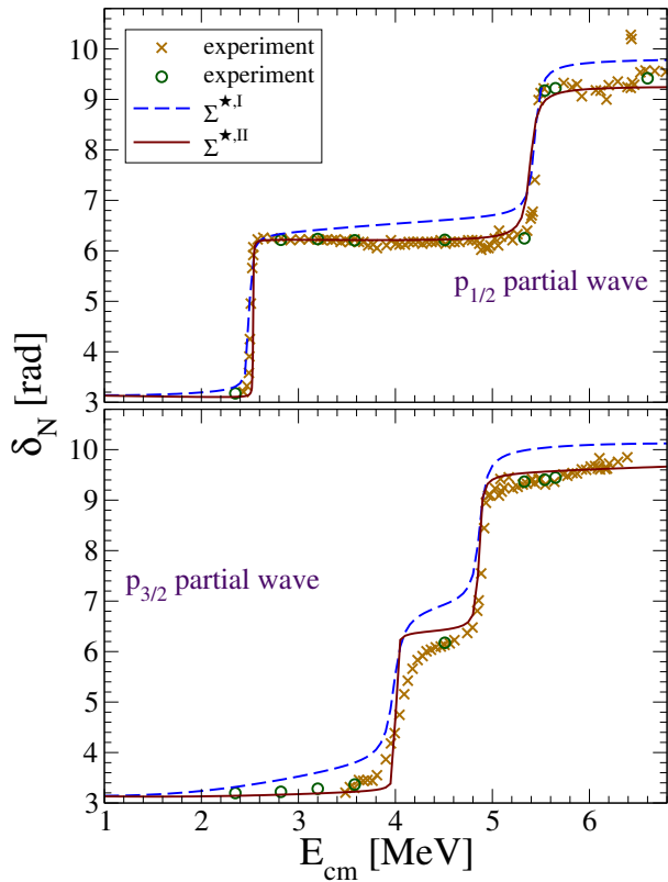
FIG. 5: Phase shifts for negative parity waves obtained from the the self-energies I (dashed lines) and II (full lines). The experimental results are from Refs. [31] (crosses) and [32] (circles).
