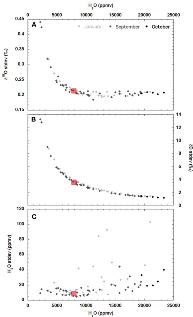
Figure 4. Water background stability. Each point corresponds to the standard deviation of (a) \delta^{18}\text{O} , (b) \delta\text{D} , and (c) the water concentration ( \text{H}_2\text{O} ). Each set background was analyzed over a period of 3 h and we averaged the data over the last 30 min. Red squares correspond to the background values chosen.
