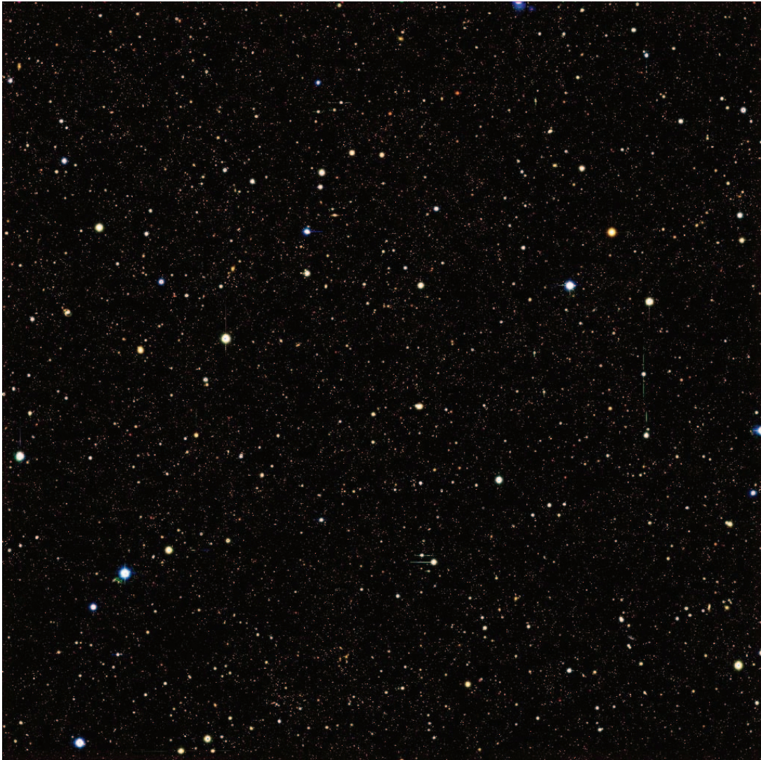
FIG. 4.—Color image of the COSMOS field made from B , r' , and z' data. The image size is 1.5^\circ \times 1.5^\circ .
