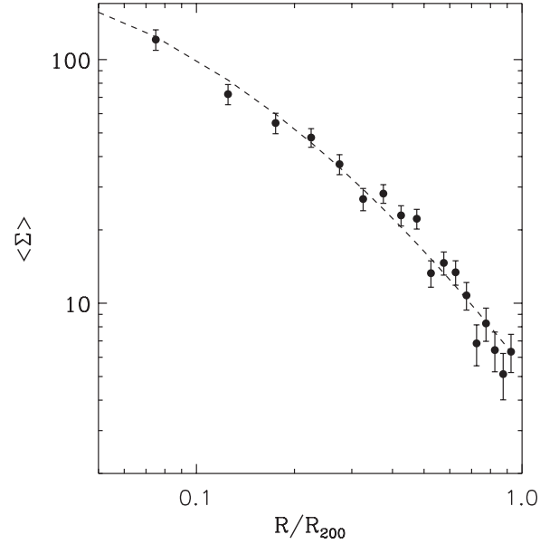
Figure 3. Radial profile of the average number galaxy density for the 91 COSMOS groups/poor clusters. The dashed line shows the best fit NFW profile ( c \sim 4 ). The unit of the surface density is number per area in unit of \pi R_{200}^2 and normalized to the total number of systems.
