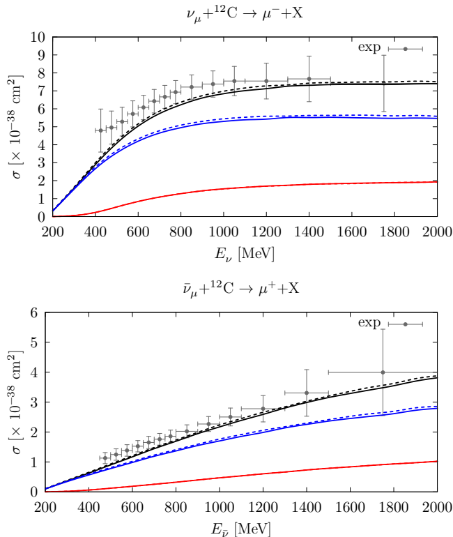
FIG. 7. CCQE \nu_{\mu} - ^{12}\text{C} total cross section per nucleon as a function of the neutrino energy. The MiniBooNE data points [28] are plotted as a function of the reconstructed neutrino energy.
