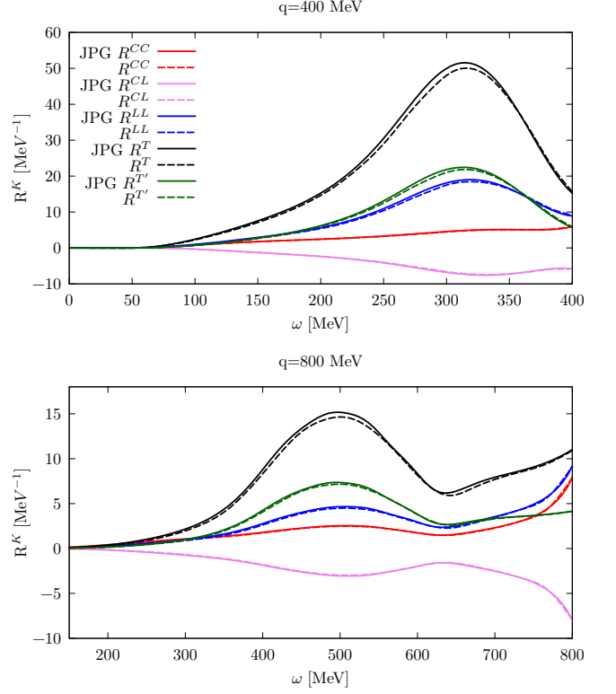
FIG. 2. The upper and lower panel display the two-body CC response functions of ^{12}\text{C} for |\mathbf{q}|=400 , and 800 MeV, respectively, obtained within the Relativistic Fermi gas model. We benchmark our results displayed by the dashed curves with those of Ref. [22] corresponding to the solid curves.
