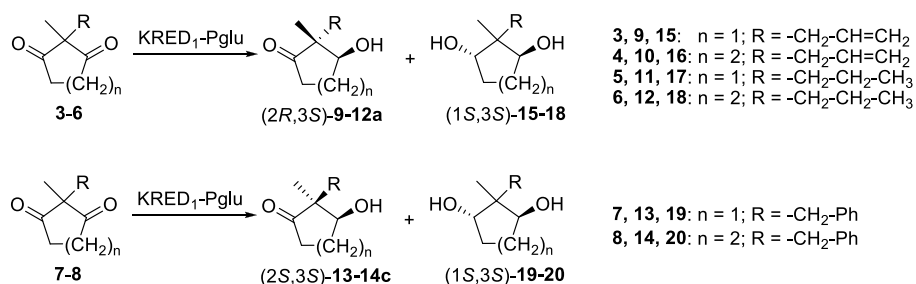
Scheme 4. Reduction of 2,2-disubstituted-1,3-cyclopentanediones and 1,3-cyclohexanediones with KRED1-Pglu.
