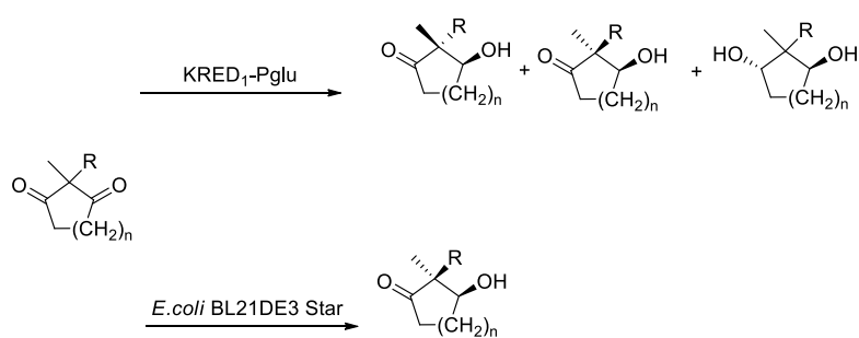
Scheme 1: Aim of the work
