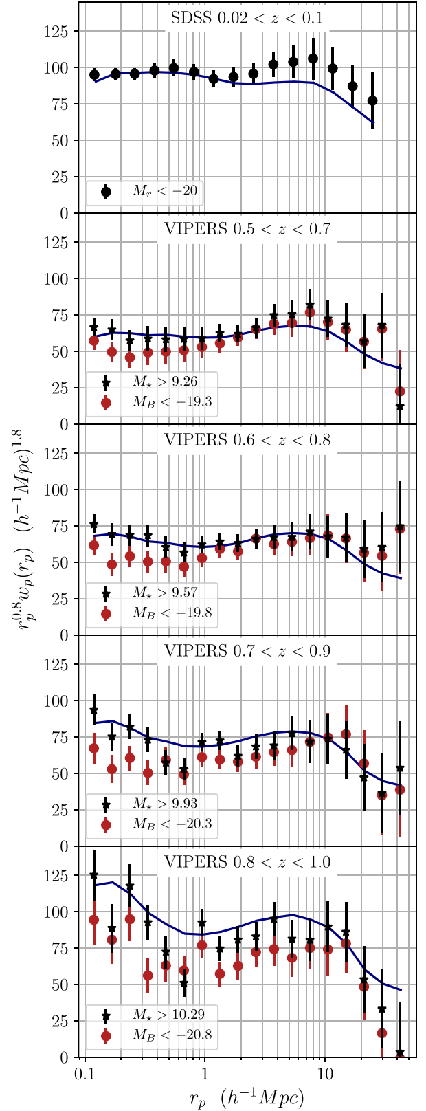
Figure 4. The projected correlation function measured in SDSS (top panel) and VIPERS (bottom four panels) in luminosity- and stellar-mass-selected samples. The matched samples have the same number density and thus share the same SHAM model (solid curve).
