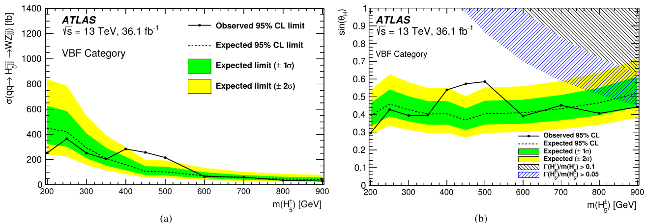
Fig. 7. Observed and expected 95% CL upper limits on (a) \sigma \times \mathcal{B}(H_5^{\pm} \rightarrow W^{\pm}Z) and (b) the parameter \sin\theta_H of the GM Model as a function of m_{H_5^{\pm}} . The shaded region shows where the theoretical intrinsic width of the resonance would be larger than 5% or 10% of the mass.
